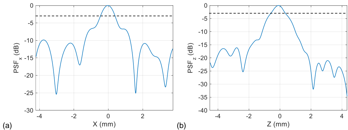
Figure II-20. 1D cuts of the experimental reconstructed PSF in (a) x-direction and (b) z-direction, in dB. The dashed line indicates the level of -3dB at which the value of the experimental resolution is extracted.
