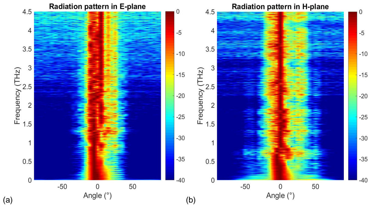
Figure II-10. Spectral radiation pattern of the antenna from 0 to 4.5 THz at (a) E-plane and (b) H-plane, in dB. The amplitude is normalized to the maximum at each frequency.
