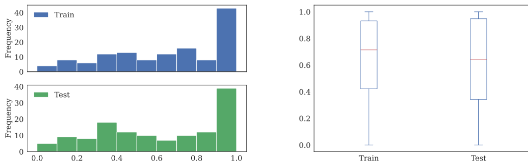
Figure 6.6: Distribution of the normalized anomaly score obtained with GMME on the ACRE category.
