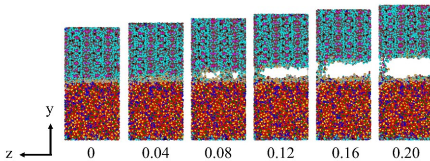
Figure 2.33 Direct tension of C-S-H (I)/H 2 O (3.1 Å)/AFt composite counterclockwise rotated in y-direction (Cube shape supercells).
