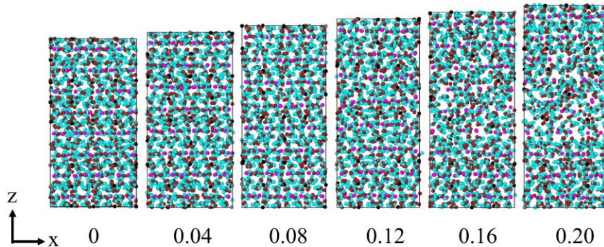
Figure 1.17 Direct tension in z-direction in xz-plane after relaxation to 20% strain of 2 \times 2 \times 2 AFt supercell with ReaxFF force field and strain rate of 10^{-6} fs ^{-1} .
