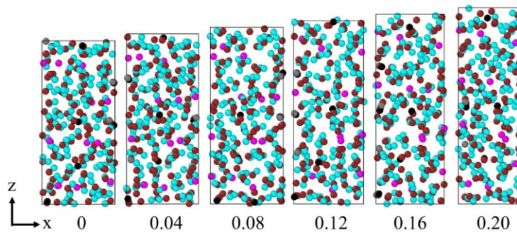
Figure 1.16 Direct tension in z-direction in xz-plane after relaxation to 20% strain of 1 \times 1 \times 1 AFt supercell with ReaxFF force field and strain rate of 10^{-6} fs ^{-1} .
