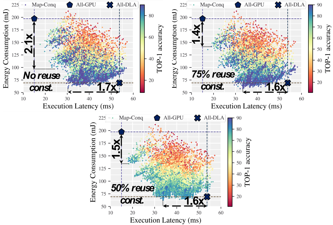
Figure 5.6 Results of three search strategies ( From left to right ): No constraint is set on the Fmap Reuse . Under a constraint of reusing only less than 75% of feature maps . Under a constraint of reusing only less than 50% of feature maps . All the results are reported for Visformer on the AGX Xavier MPSoC. In the three plots, we highlight the configurations that exhibit the highest latency-energy tradeoff while preserving less than 0.5% drop in accuracy
