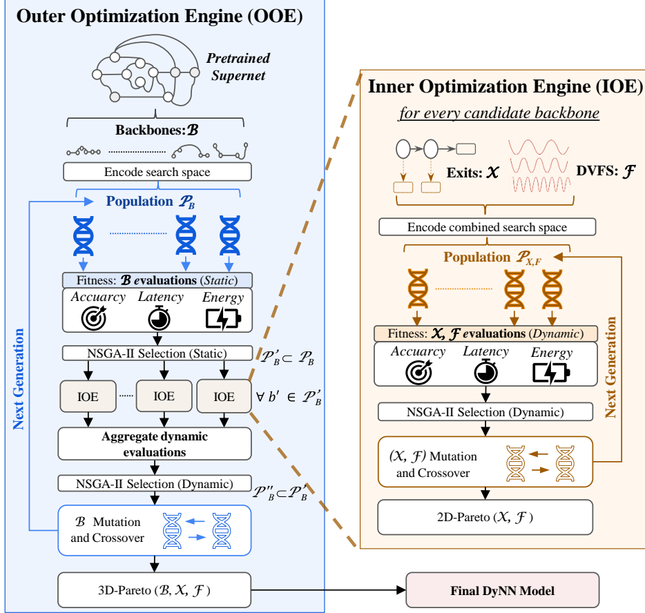
Figure 3.3 HADAS co-optimization framework.
