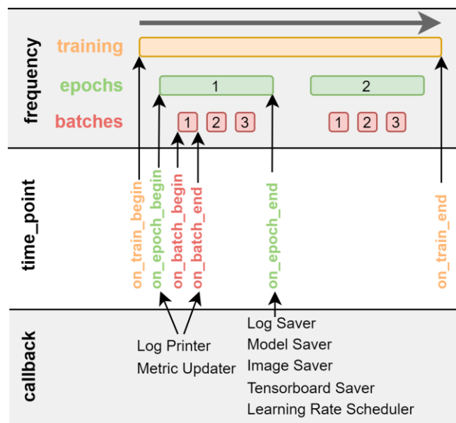
Figure 3-16 – Callback Module principle. The whole training ( top row, orange ) is divided into epochs ( green ) themselves divided into batches ( red ). Callbacks are Python classes that can have one or more class-functions, each representing one of 6 different time points ( middle row ). Biom3d currently has 7 types of Callback Modules ( bottom row ).
