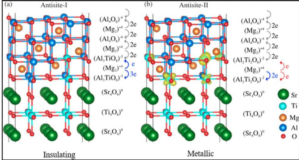
Figure 1.10 – Atomic intermixing at the \text{MgAl}_2\text{O}_4/\text{SrTiO}_3(001) interface. Depending on the antisite model, the interface can (a) remain insulating or (b) become conducting. The model “Antisite-II” could explain the experimental measurements. The charge density of the conducting 3d states is printed in yellow. (Reprinted from Ref. [154] with permission)
