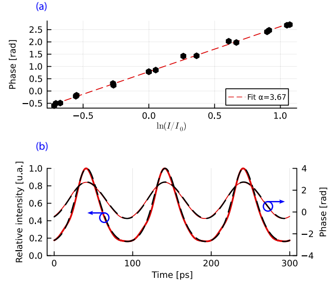
Fig. 4. (a) Plot of \phi(t) as a function of \ln(I/I_0) . (b) Reconstructed (full lines) versus simulated (dashed lines) I(t) and \phi(t) . The simulation uses Eqs. (6)–(8), with \alpha = 3.67 , r = 3 , m = 0.59 , \epsilon = 0.028 .
