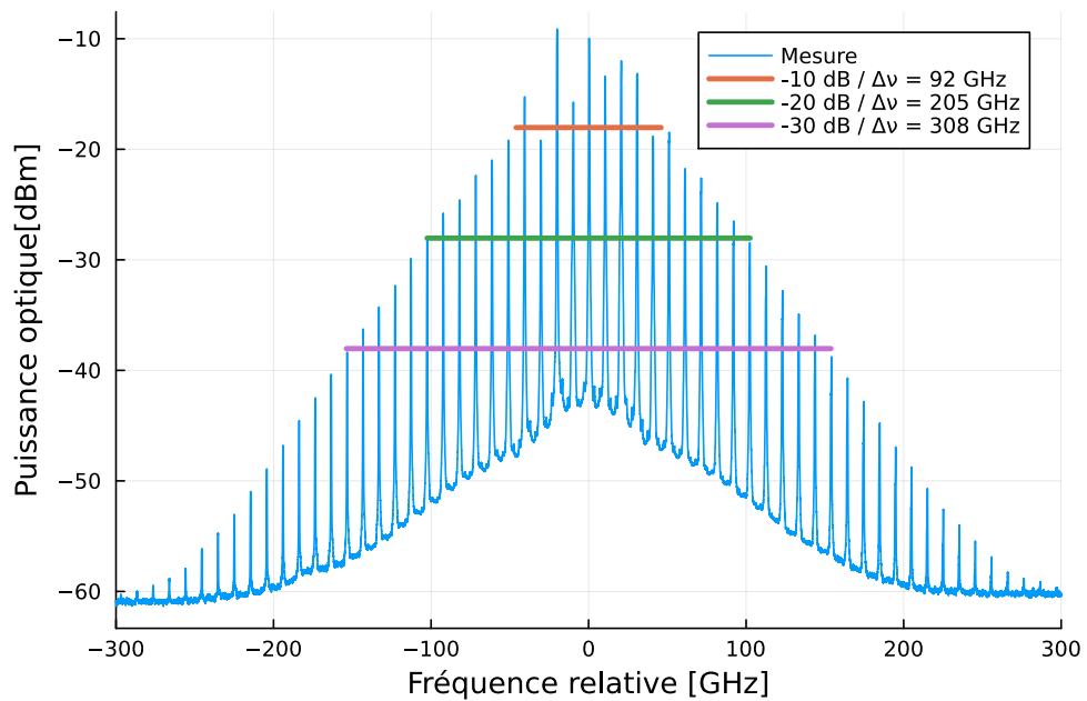
FIGURE 4.26 – Spectre optique.
