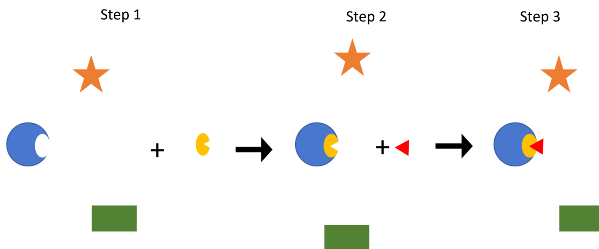
Figure 15 : Labelling of a biomolecule by bioorthogonal chemistry. Step 1 is the first step in which the chemical reporter (yellow oval) is added to the sample containing the target biopolymer (blue circle), as well as other molecules that not affected by the reaction (green rectangle and orange star). The reporter is the bioorthogonal compound with the reactive function to be incorporated. Step 2 is the addition of the probe (red triangle). Step 3 is the specific (bioorthogonal) reaction of the probe with the chemical reporter that leads to the specific labelling of the target biopolymer.
