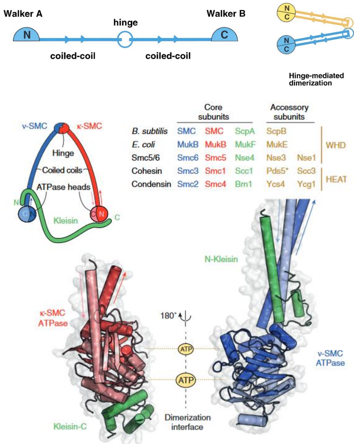
Fig. I5 General structure of SMC complexes (1)
