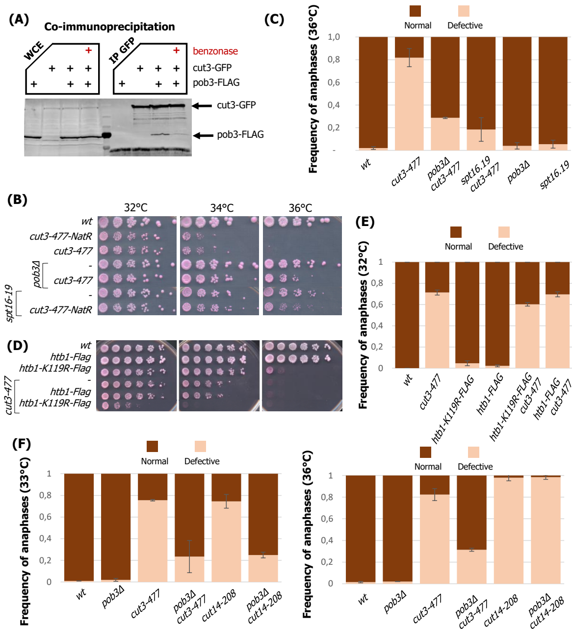
Fig. 2 FACT is a functional antagonist of condensin
