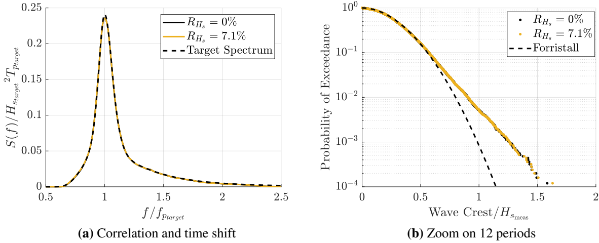
Figure 3.27 – Effects of reflected waves on the spectrum and crest distribution: R_{H_s} = 7.1\% compared with R_{H_s} = 0\% (35 seeds, HOS-NWT simulations, s s 6 g 5 sea state scale 60, x = 52\lambda_p )
