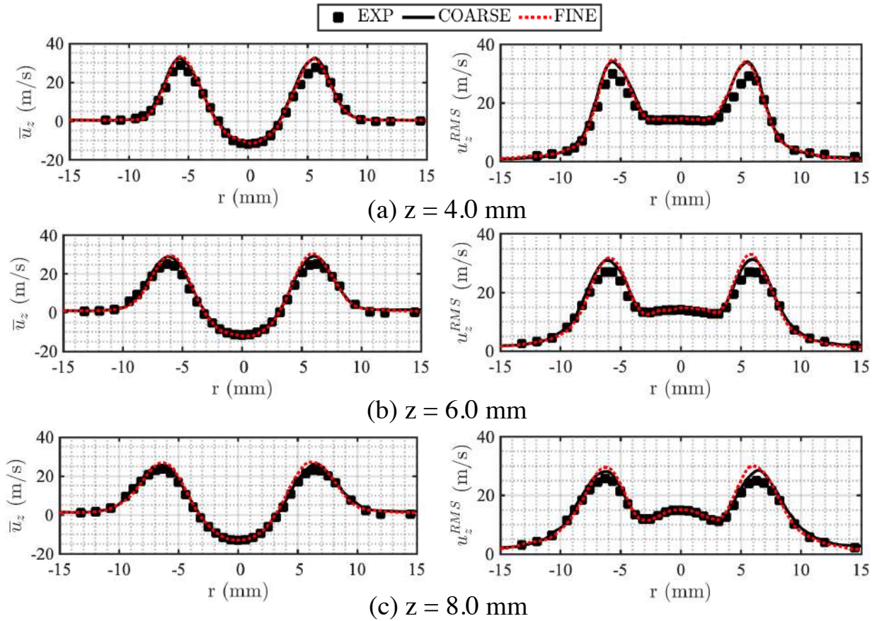
Figure 6.4. – Radial profiles of (left) the mean axial gas velocity \bar{u}_z and (right) root-mean square axial gas velocity \bar{u}_z^{RMS} at z = 4 mm, z = 6 mm and z = 8 mm. Experimental results are plotted with black filled squares. Simulations performed with the COARSE and FINE meshes are respectively plotted with continuous black lines and dotted red lines.
