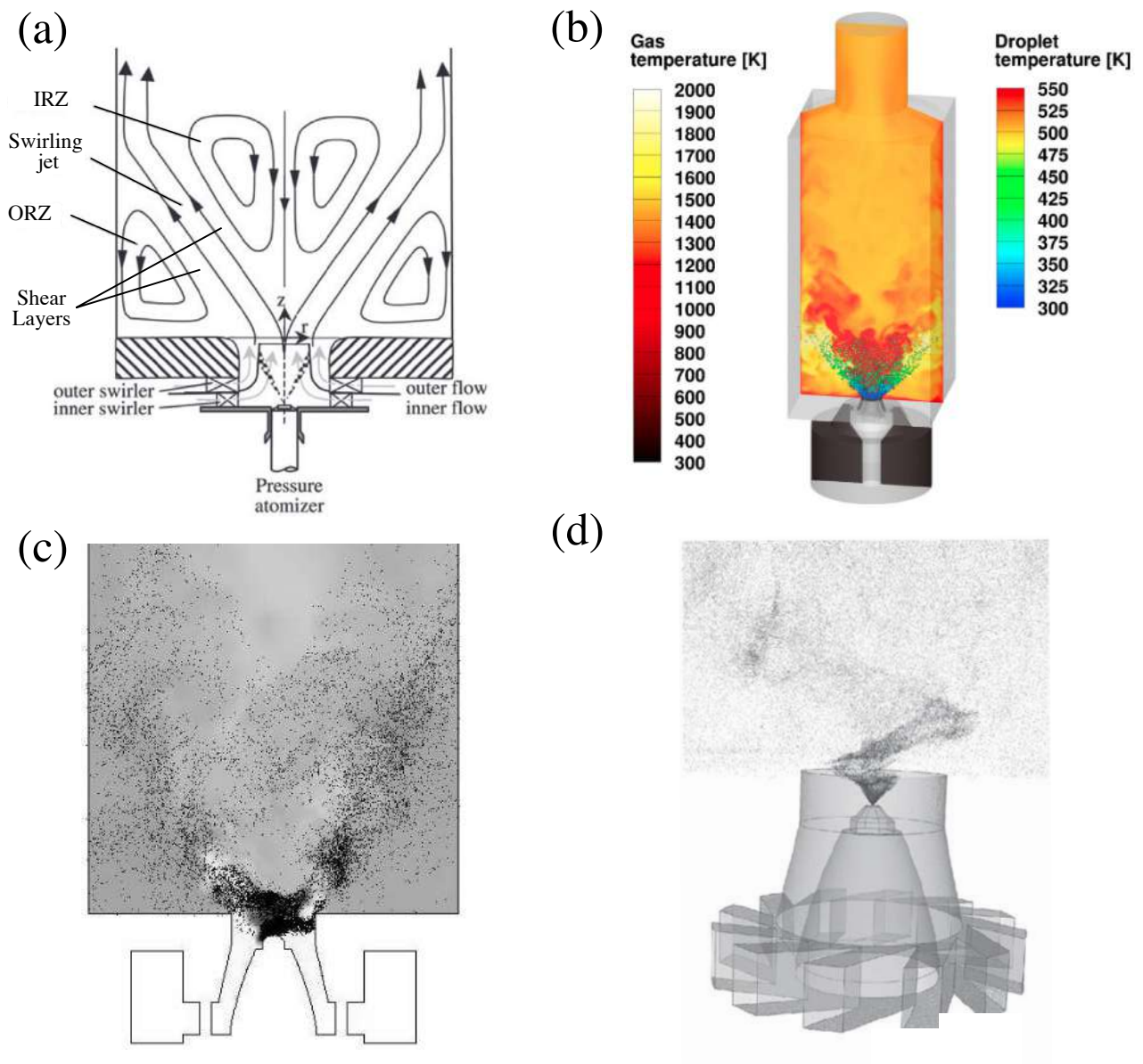
Figure 1.10. – (a) Characteristic flow features of a swirling flow (adapted from [28]) (b) Swirl-stabilized spray flame (reproduced from [29]) (c) Instantaneous droplet distribution in swirling flow (reproduced from [30]) (d) Structure of the PVC highlighted by the presence of droplets (reproduced from [31]).
