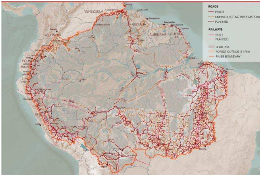
Figure 9: Roads in the Amazon (Source: Map 7 in RAISG 2020, p.21).
