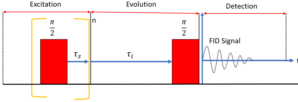
Figure 1.9: Example of the progressive saturation-recovery pulse (PSR) sequence. n is the number of \frac{\pi}{2} pulses separated by a fixed time interval \tau_s (a pulse train "comb").
