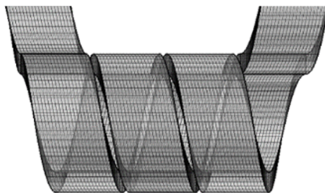
Figure 3.17: Mesh mapped method used by COMSOL Multiphysics 6.1 for the NMR coil simulation L_t .
