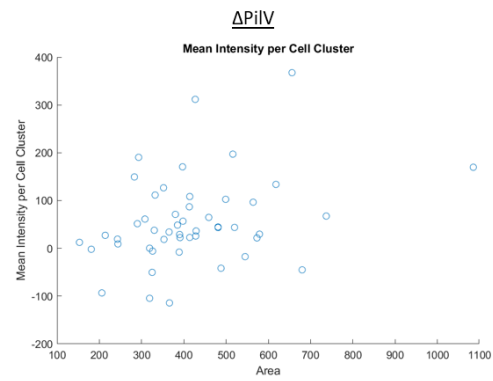
xlvi Mean intensity per Cell Cluster against area in (a) MS11 and (b) ΔPiV
