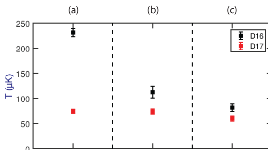
Figure 4.27: Temperature of {}^6\text{Li} and {}^7\text{Li} as function of pulse duration. The total D1 time is kept constant to \sim 3 \text{ ms} and the duration of each pulse is varied. (a) The pulse sequence ends with a {}^7\text{Li} D1 pulse. The temperature of {}^7\text{Li} remains constant whereas we observe heating in {}^6\text{Li} as we increase the pulse duration. The dotted line represents the linear fit for pulse duration \geq 50 \mu\text{s} . The corresponding heating rate is \sim 0.69 \mu\text{K}/\mu\text{s} which is in fair agreement with the calculated heating rate of section 4.7.1. (b) The pulse sequence ends with a {}^6\text{Li} D1 pulse. The temperature of {}^7\text{Li} remains unaffected and, as we increase the last pulse duration, the {}^6\text{Li} temperature quickly drops to a steady state.
