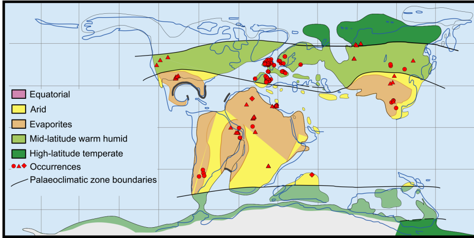
(a) Aptian
