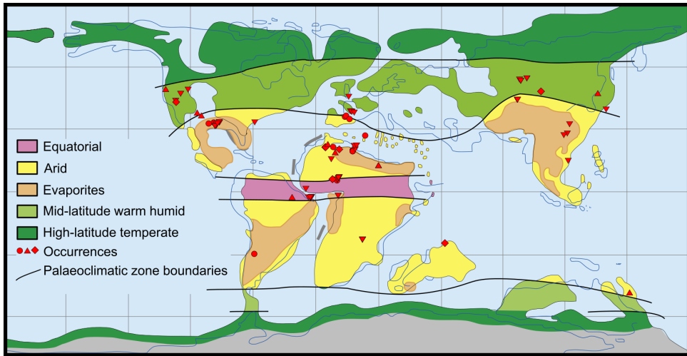
(b) Albian
