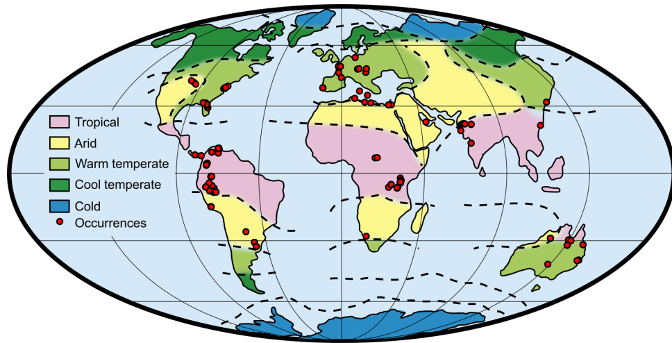
(e) Miocene
