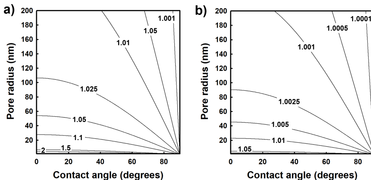
Figure 9: Estimations of PCS effect by contact angle and pore radius for \text{SrSO}_4 in water as estimated by the modified Kelvin equation (Eq. 9). a) PCS effect for celestine nucleation, b) PCS effect for hydrate nucleation.
