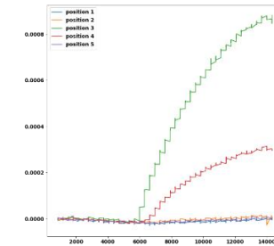
10% + Thiol
