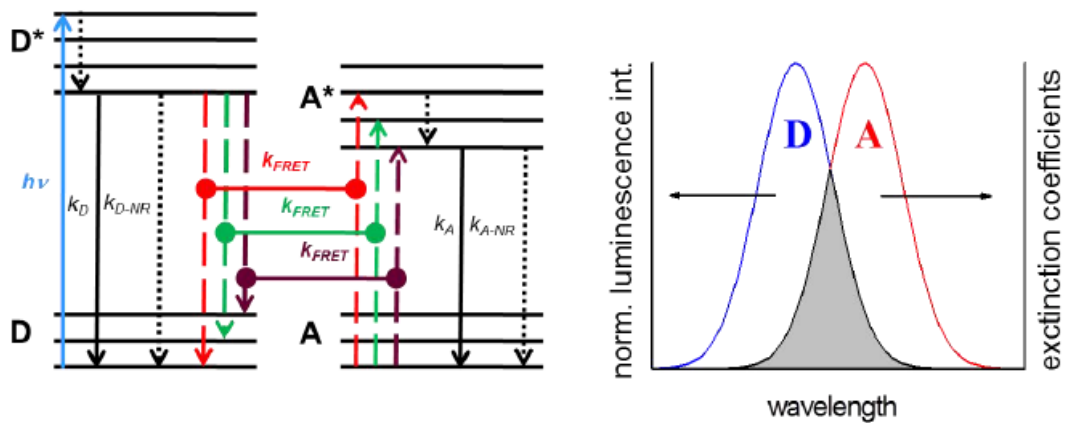
Figure 2.12 (Left) Simplified Jablonski diagram representing the energy levels of the donor (D) and acceptor (A) molecules. (Right) Spectral overlap between the donor emission and the acceptor absorption. 51
