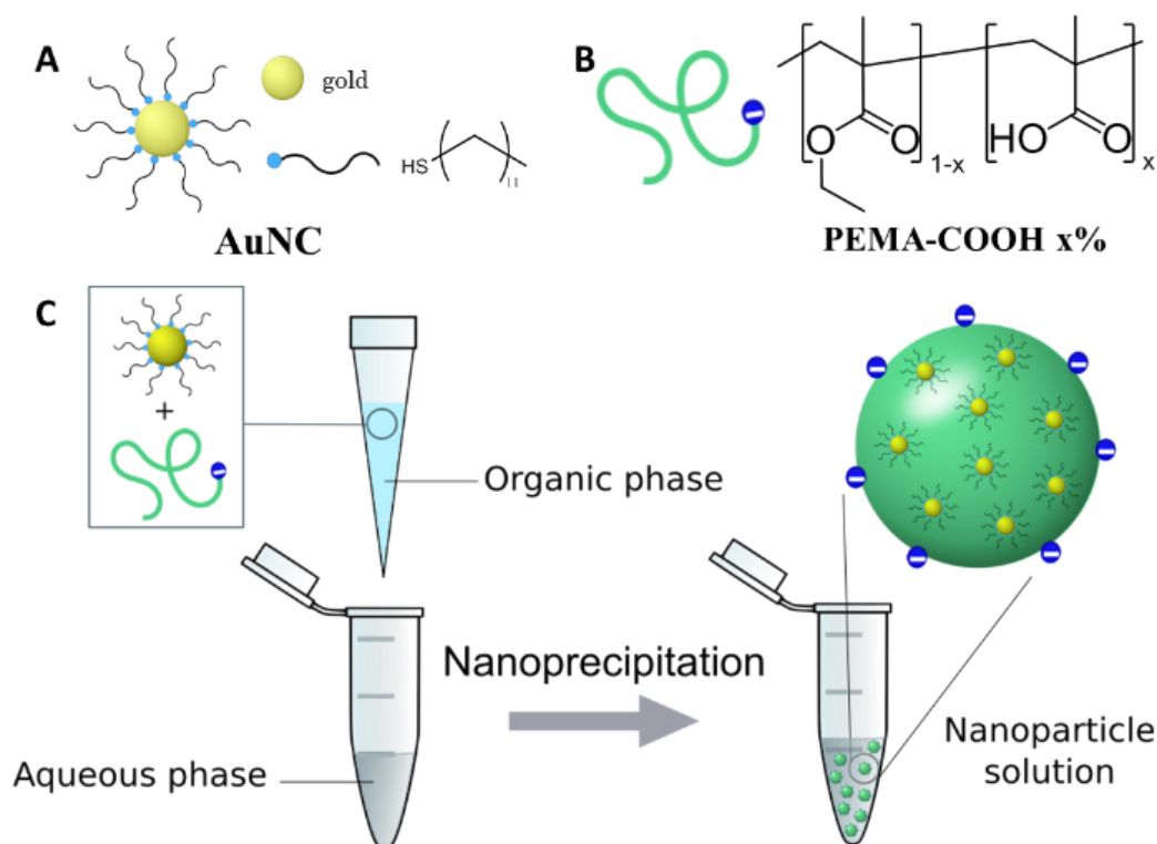
Figure 3.0 (A) Structure and representation of gold nanoclusters stabilised by dodecanethiol (AuNC). (B) Structure and representation of the polymer. (C) Principle of NP synthesis through nanoprecipitation
