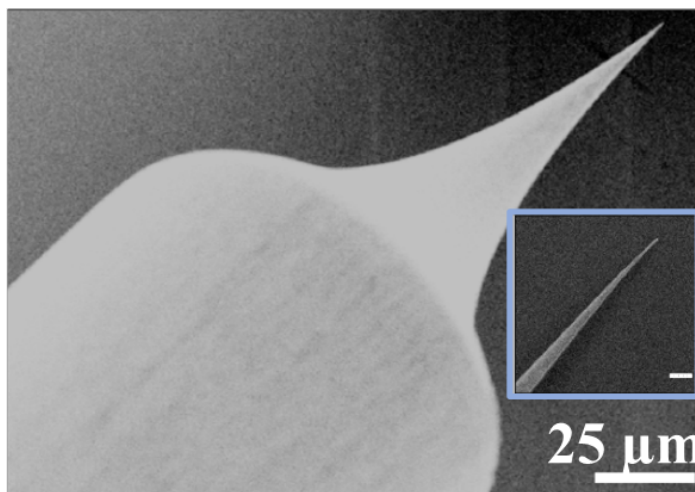
Figure 2.10 – SEM image of the tip apex, the inset shows a zoom of the apex. The scale in the inset image is 2\mu\text{m} .
