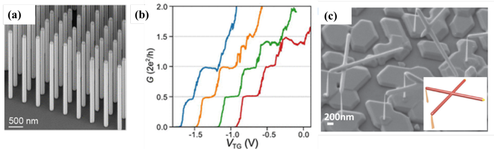
Figure 1.14 – (a) Vertical stemless InSb nanowires [72] (b) Measured Quantum Point Contact (QPC) conductance versus the top-gate voltage at 6K presenting quantized conductance behaviour [72] (c) , InSb nanocrosses resulting from the merging process between two InSb nanowires. The inset shows InAs and InSb segments in orange and red, respectively, and the Au–In droplet is in yellow [71].
