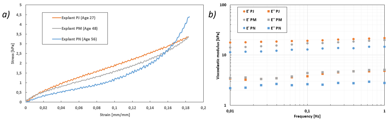
Figure 4.22: Results of tensile tests on 3 explants from 3 donors of different ages. Explant PN (56 years old) considered to be old; explant PJ (27 years old) considered to be young; explant PM (48 years old) from an intermediate age group. a) Simple traction (speed = 10 mm.min -1 ). b) Frequency sweep (strain = 10%).
