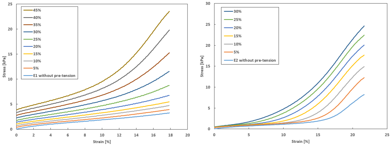
Figure 3.12: Influence of explant pre-tension on its mechanical behaviour in elongation. Tensile tests on 2 human skin explants (right and left graphics - speed = 10 mm.min -1 ) with different initial pre-tensions.
