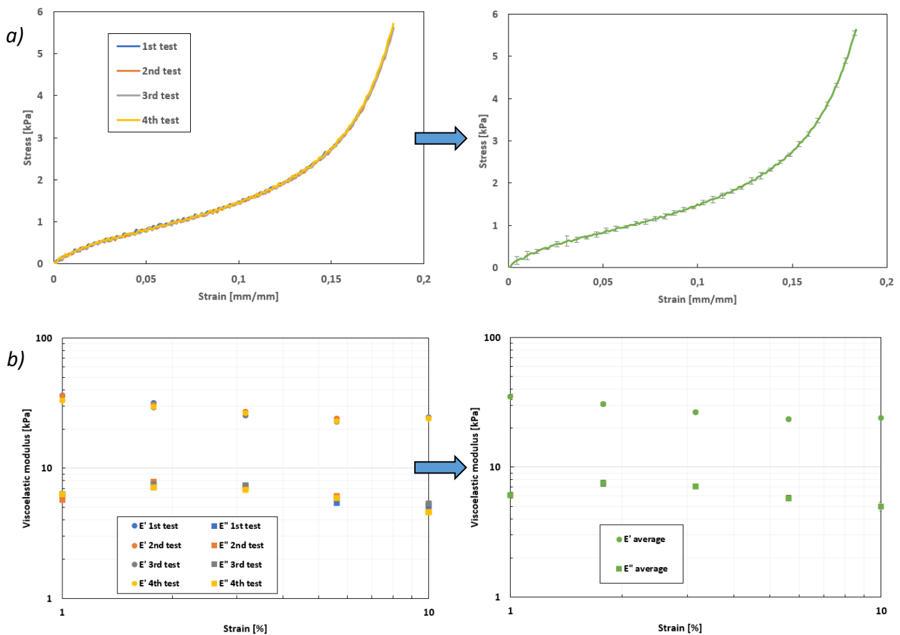
Figure 3.3: Repeatability of tests on a human skin explant. a) Tensile test (speed = 10 mm.min -1 ): 4 tests + average curve with standard deviation. b) Dynamic test (strain sweep at 0.5 Hz): 4 tests + average curve with standard deviation.
