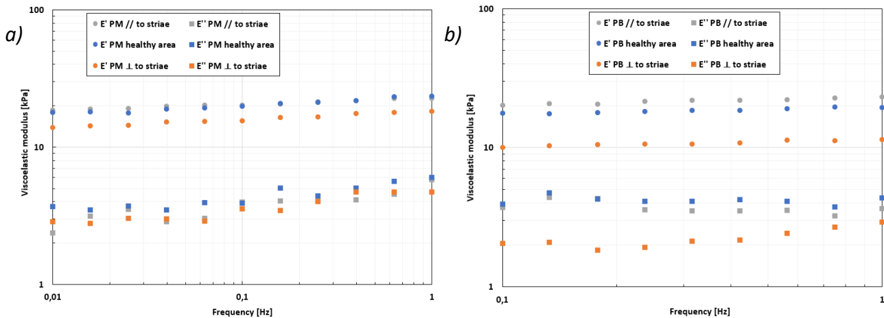
Figure 5.7: Study on stretch marks: frequency sweep tests on 2 explants with stretch marks, in 3 load directions (strain = 10%). Graphs of viscoelastic moduli as a function of frequency. Explants PM (a) and PB (b).
