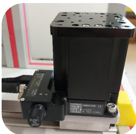
Figure 2.10: Specific support with integrated motor controllers and encoders.
