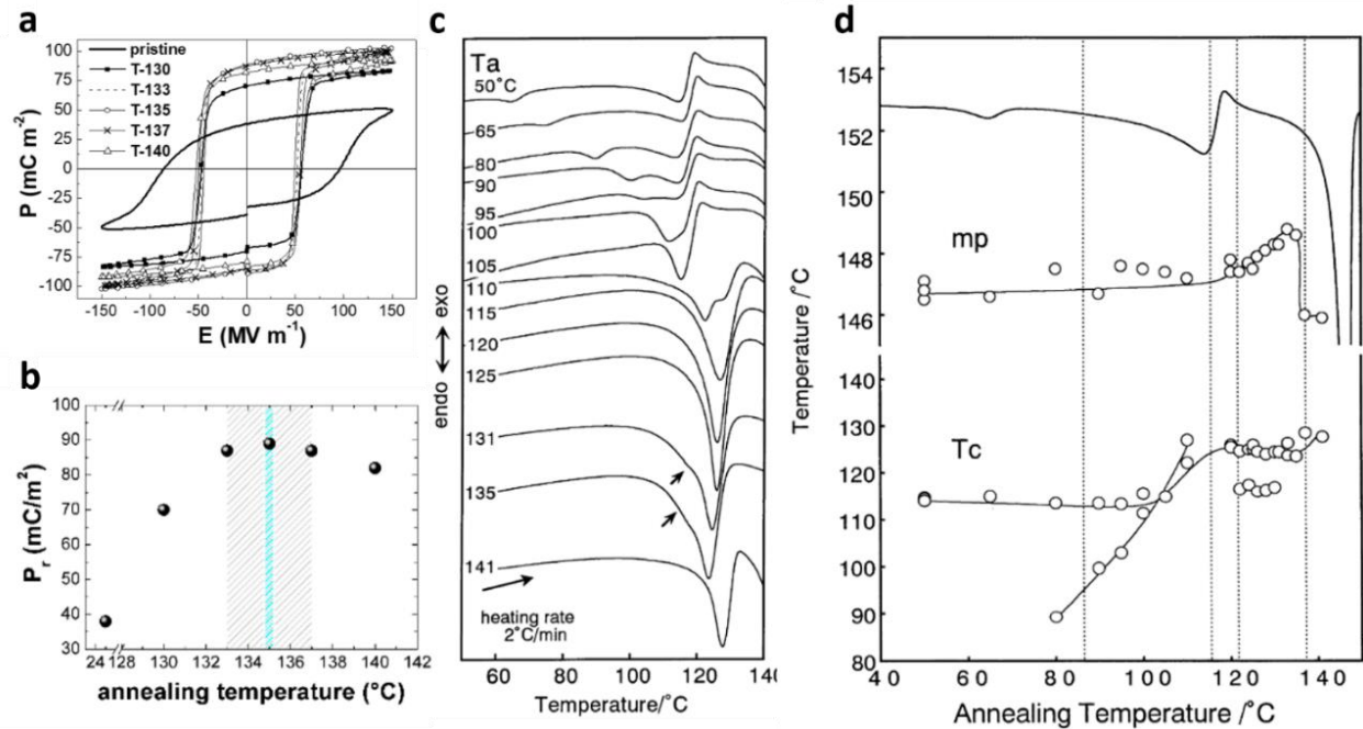
Figure 22. (a) and (b) Polarization loops and remanent polarization values according to the annealing temperature of a P(VDF-TrFE) copolymer reproduced from Spampinato 73 , (c) and (d) DSC thermograms and evolution of the Curie transition temperature ( T_c ) and the melting point ( mp ) reproduced from Tanaka et al. 54
