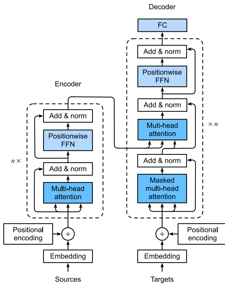
FIGURE 2.11 – Architecture Transformer encodeur-décodeur [Dev+19].
