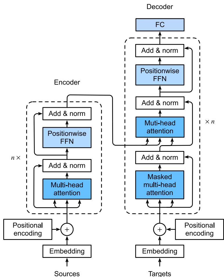
FIGURE 2.11 – Architecture Transformer encodeur-décodeur [Dev+19].
