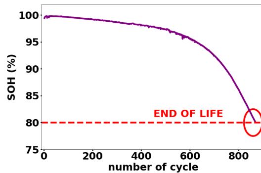
Figure 6: Evolution of SOH, from 100% to 80%
