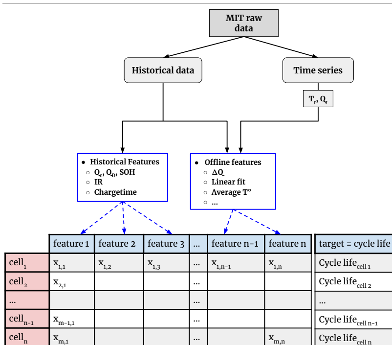
Figure 2.6: Cell-based dataset for the offline prediction of the global cycle life
