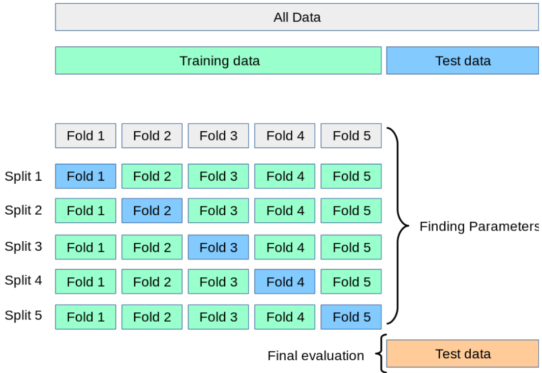
Figure 2.10: K-fold validation process (Sklearn, Cross-validation: evaluating estimator performance)
