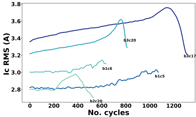
Figure 3.4: I_C RMS
