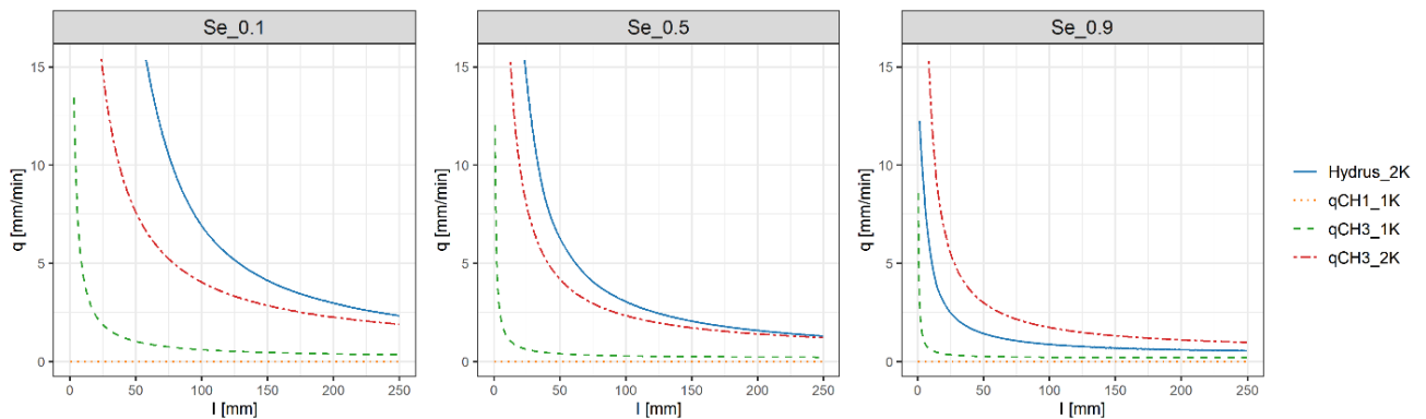
Figure (4.7): Result of direct infiltration modeling using the ( CH1_1K , CH3-1K , CH3-2K ) models for Loam compared to numerical infiltration modeled using Hydrus-2K for three different saturation scenarios (Dry soil ( Se=0.1 ), intermediate soil ( Se=0.5 ), saturate soil ( Se=0.9 ))
