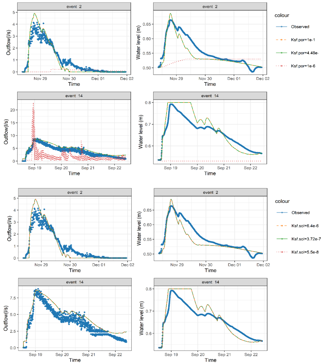
Figure (4.12): The sensitivity analysis of the model regarding the conductivity hydraulic of macropores and matrix
