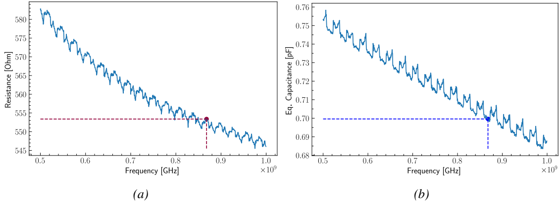
Figure 3.19: Equivalent resistance (a) and capacitance (b) of a MEMS with ( R = 100\mu\text{m}, h = 3.5\mu\text{m}, g_0 = 0.3\mu\text{m} ). The dotted lines highlight the extracted equivalent resistance and capacitance of the MEMS at 868 MHz.
