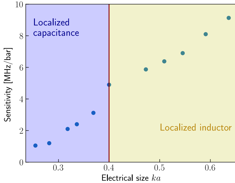
Figure 2.32: Sensitivity of the sensor vs antenna electrical size
