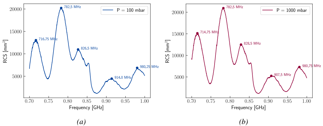
Figure 4.22: Raw measurement of the Slot sensor before the time gating, at 100 mbar (a) and 1 bar (b) with the frequencies of the main peaks.
