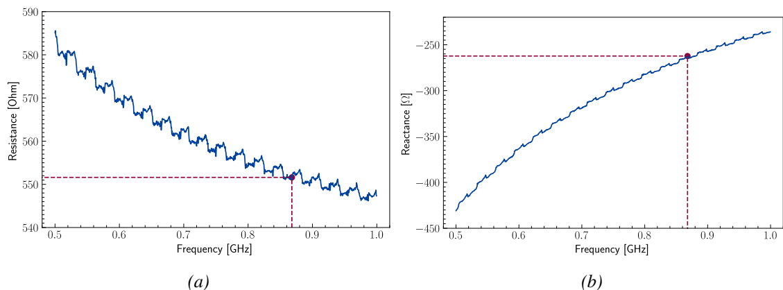
Figure 4.2: Real (a) and imaginary parts (b) of the impedance of one of the 4 MEMS put in parallel as the load of the PIFA antenna at 1 bar. The points with the dotted lines correspond to the value of the impedance at 868 MHz. The small periodic variations in the curves are due to the prober used for the characterization of the MEMS. At 868 MHz and 1 bar, the 4 MEMS in parallel have an equivalent impedance of 137.9 - j65.57\Omega .
