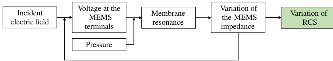
Figure 5.8: Block diagram of the interrogation of resonant MEMS using intermodulation, with the current step of the calculation highlighted. This section focuses on determining the expression of the RCS of the antenna based on the reflection coefficient. Then, the expression of the electric signal received can be expressed.
