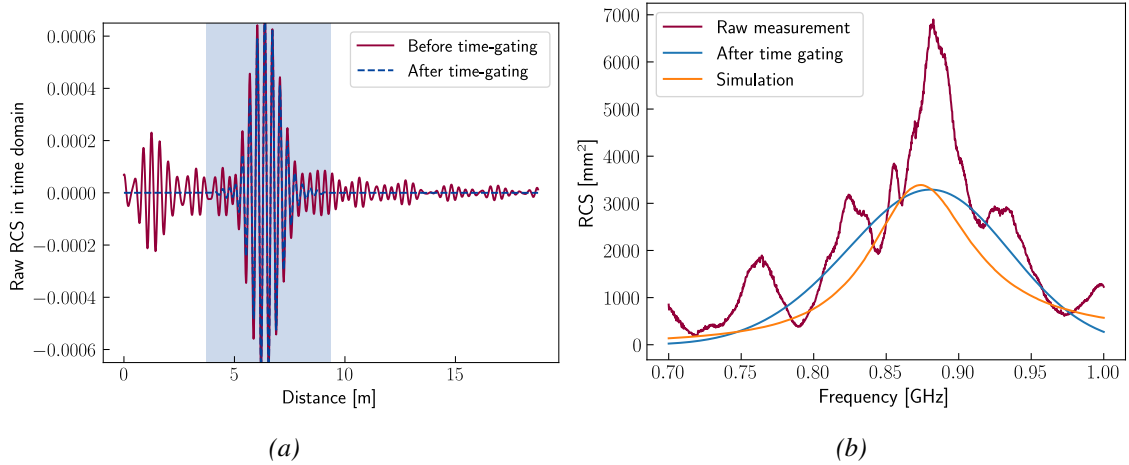
Figure 4.14: Time-domain (a) and frequency (b) response of the PIFA and comparison with the simulation. The colored area correspond to the window applied.
