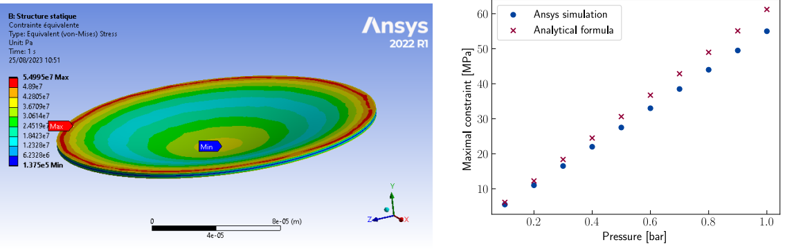
Figure 2.5: Simulation on Ansys Mechanical of the constraint on the membrane of the MEMS with dimensions of (R = 100\mu\text{m}, g_0 = 0.3\mu\text{m}, h = 3.5\mu\text{m}) at 1 bar and comparison between the maximal constraint extracted from simulation and from equation 2.4.
