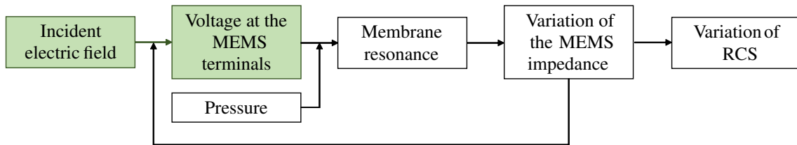
Figure 5.3: Block diagram of the interrogation of resonant MEMS using intermodulation, with the current step of the calculation highlighted. This section focuses on determining the voltage across the MEMS based on the incident electric field.
