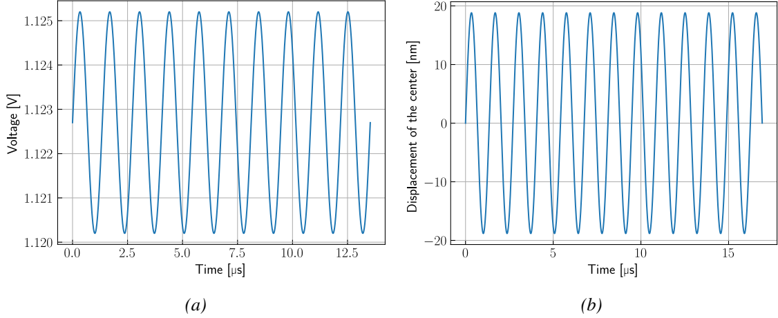
Figure 5.16: Example of voltage (a) and displacement of the center of the membrane (b) in time-domain and steady state, calculated using the complete model. Using the linearized model, the calculated voltage is V_S = 1.1226V , and the calculated displacement of the center of the membrane is \Delta x(t) = 18.839 \times 10^{-9} \sin \omega_m t (in meters).
