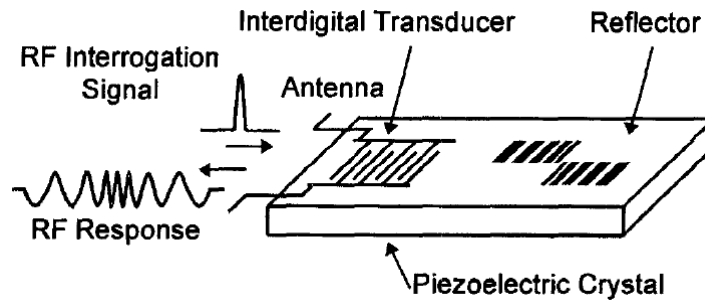
Figure 1.4: Working principle of a wireless surface acoustic wave sensor [15].
