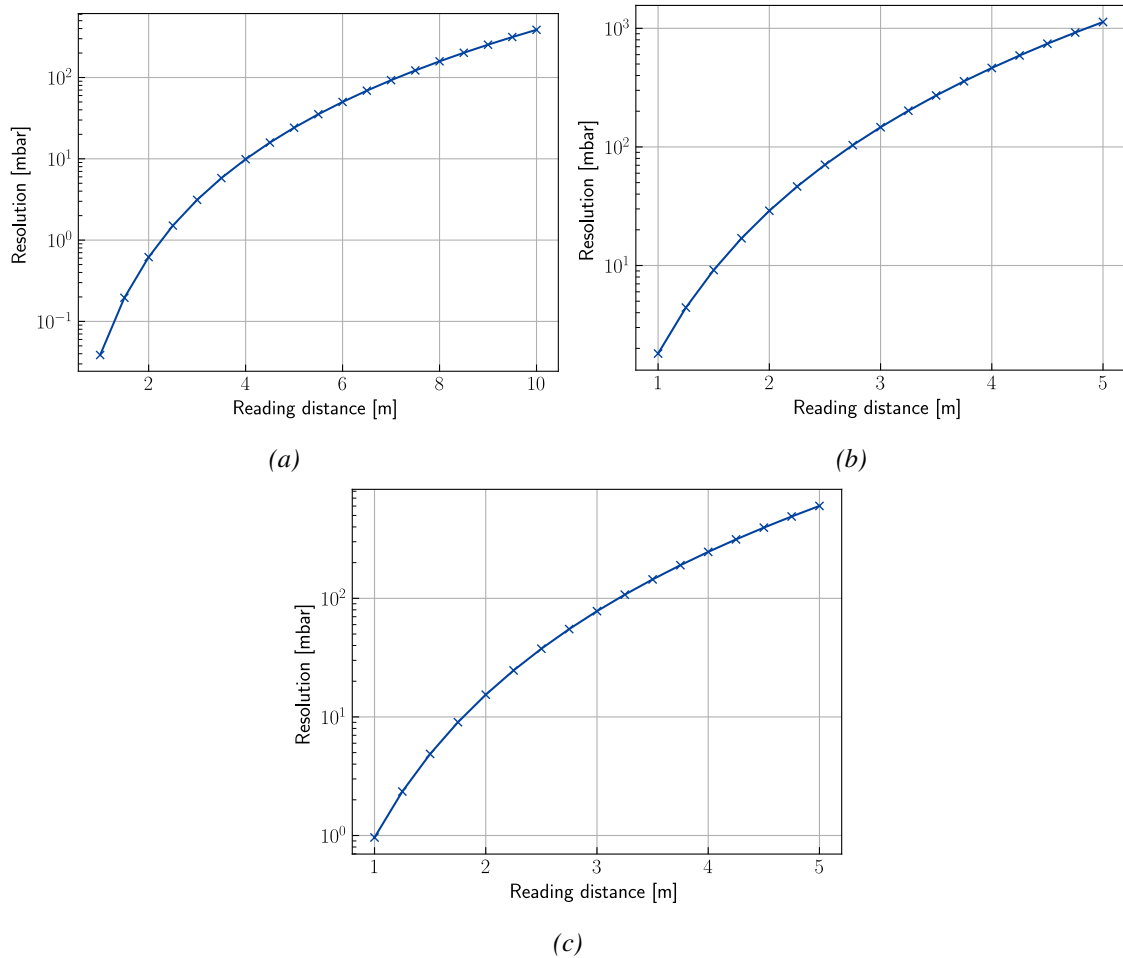
Figure 4.30: Evolution of the maximal resolution achievable in function of the distance for the PIFA sensor (a), the Loop sensor (b) and the Slot sensor (c).
