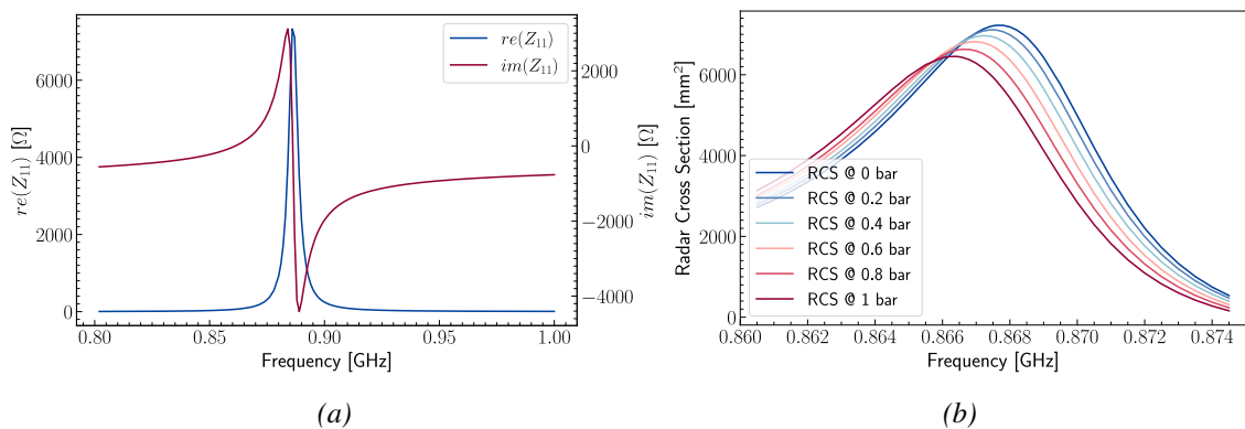
Figure 5.14: Input impedance (a) and evolution of the RCS with the pressure (b) for the CLL antenna used in this analysis.
