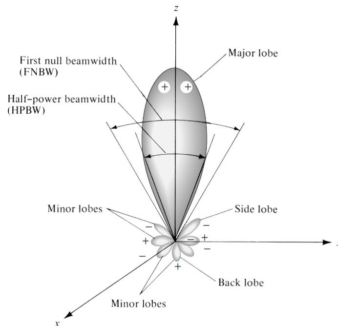
Figure 1.9: 3D representation of a radiation pattern [33].
