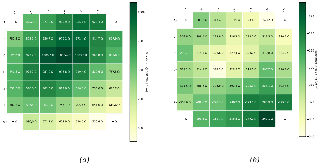
Figure 3.20: Mappings of resistance (a) and reactance (b) at 868 MHz of a MEMS with R = 100\mu\text{m}, h = 3.5\mu\text{m} and g_0 = 0.3\mu\text{m}
