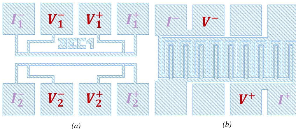
Figure 3.12: Test structures to characterize the quality of etching of AlCu. (a) Test structure to characterize the over-etching and the sheet resistance. (b) Test structure to characterize isolation and continuity.
