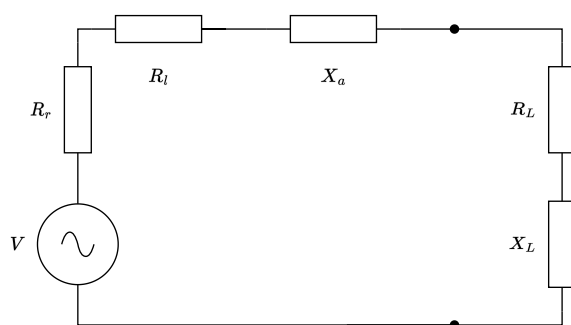
Figure 1.8: Equivalent circuit of a loaded antenna.
