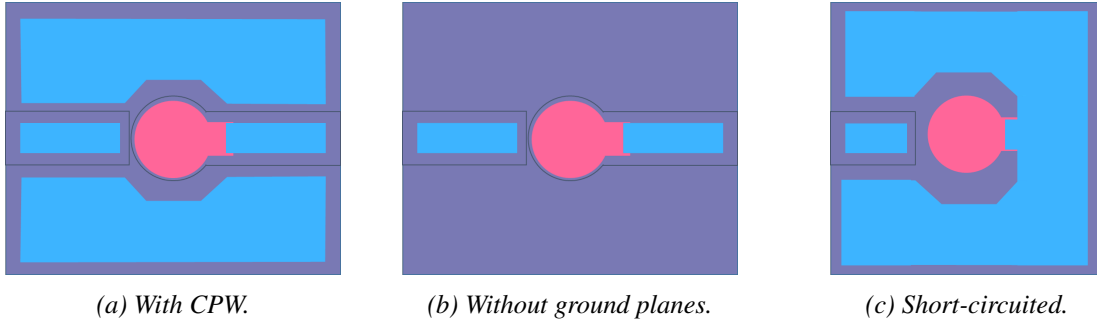
Figure 2.16: Variants of the lines of the MEMS on the wafer.
