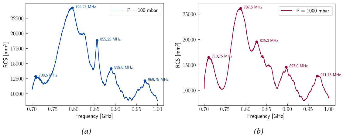
Figure 4.21: Raw measurement of the Loop sensor before the time gating, at 100 mbar (a) and 1 bar (b) with the frequencies of the main peaks.
