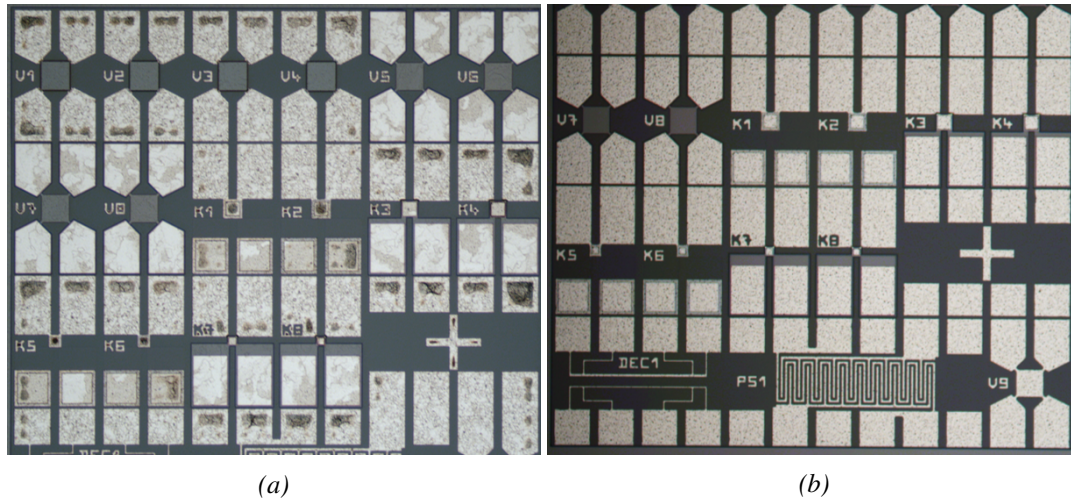
Figure 3.13: Comparison between the appearance of the two metals used AlCu and AlSi. (a) Cell of technological tests with AlCu. (b) Cell of technological tests with AlSi.
