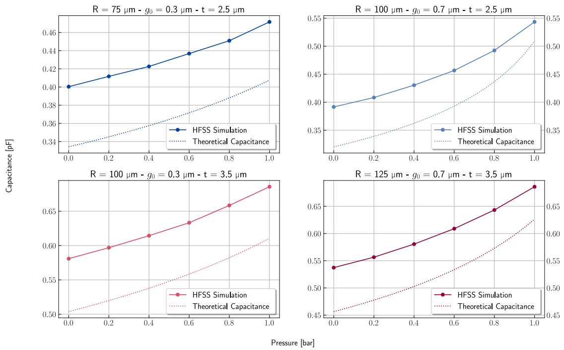
Figure 2.20: Simulated equivalent capacitance of the MEMS of the first set and comparison with analytical results.
