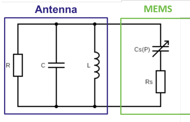
Figure 2.33: Representation by a simplified equivalent circuit of the antenna loaded by the MEMS.
