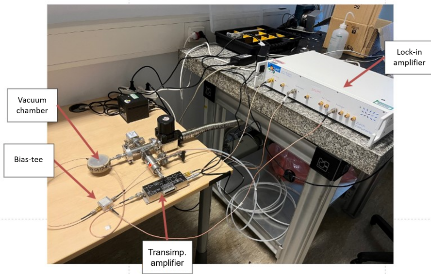
Figure 5.24: Setup of measurement of the peaks of intermodulation of the MEMS. The MEMS is placed on a PCB inside a vacuum chamber. The two sent signals were generated using a lock-in amplifier. A bias-tee is used at the output of the MEMS to separate the DC and the AC signals of the voltage, which is then converted into current thanks to a transimpedance amplifier.
