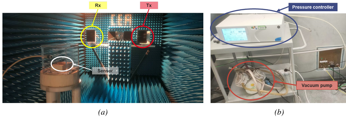
Figure 4.17: Measurement setup of the sensors in anechoic chamber. The sensor are placed inside a vacuum chamber. The pressure controller, connected to a vacuum pump, is used to change the pressure inside the vacuum chamber. The two antennas in Rx and Tx are used for the interrogation of the sensor. (a) Interior of the anechoic chamber (b) Vacuum pump and pressure controller outside the anechoic chamber.
