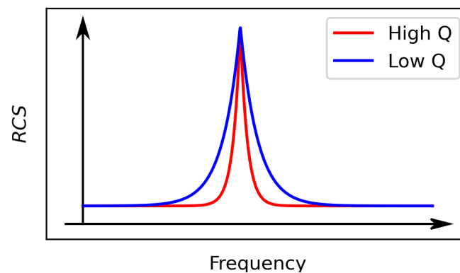
Figure 1.10: Comparison of the curves of the transfer functions of the antenna for high and low quality factors
