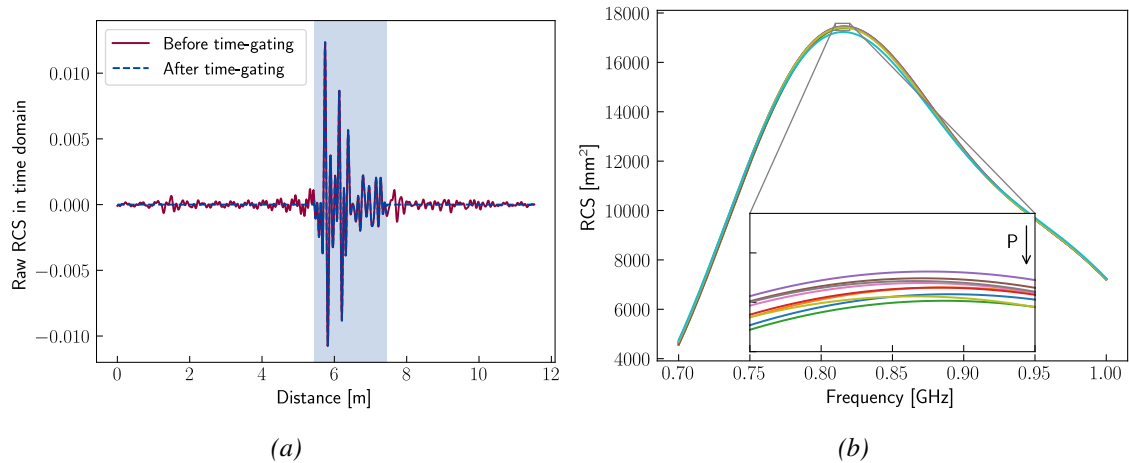
Figure 4.24: RCS of the Loop sensor extracted from the algorithm in time-domain (a) and frequency domain (b). The colored area in time-domain correspond to the window applied. The arrow indicates the reading direction for increasing pressure. 10 measurements are taken between 100 and 1000 mbar, in 100 mbar steps.
