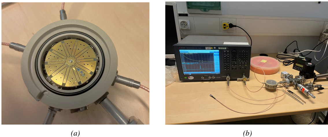
Figure 5.21: View of the PCB inside the vacuum chamber (a) and the measurement setup (b) including a Keysight E5061B ENA Vector Analyzer and a vacuum pump.
