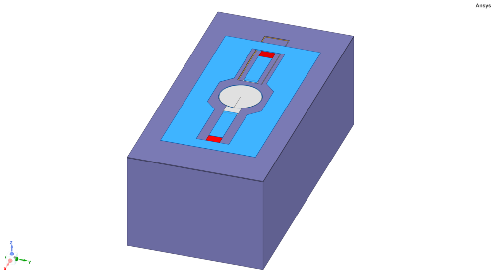
Figure 2.19: MEMS geometry simulated on Ansys HFSS. The red rectangles are the lumped ports.
