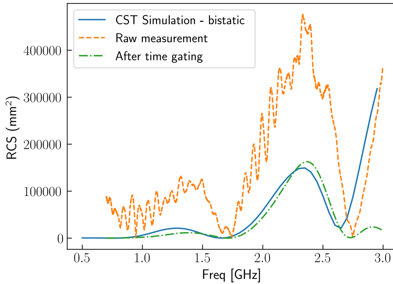
Figure 4.18: RCS of the vacuum chamber. At 868 MHz, the vacuum chamber does not reflect a lot of power, as its RCS is 573.86 mm 2 .
