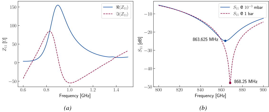
Figure 4.7: Electrical properties of the Loop sensor. (a) Input impedance of the Loop antenna at the location of the MEMS. (b) Reflection coefficient of the antenna loaded by the MEMS.
