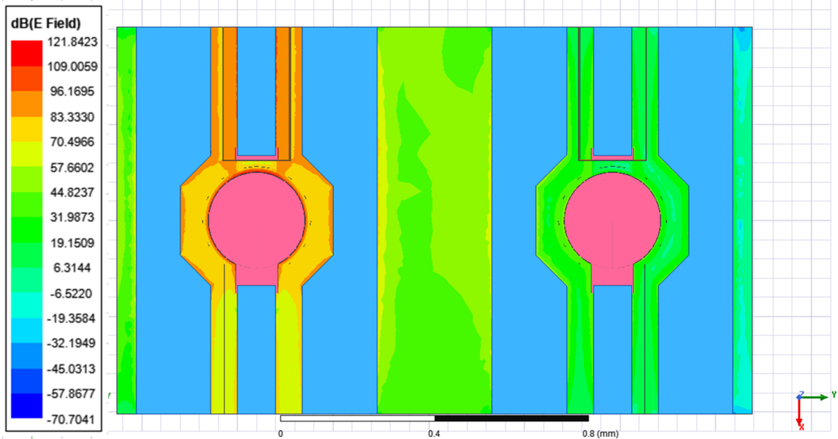
Figure 2.29: EM simulation of two MEMS on Ansys HFSS to simulate the cross-talk, with the electric field plotted.
