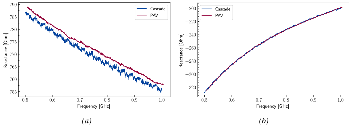
Figure 3.23: Comparison of the measurements made by the two probers of the real (a) and imaginary part (b) of the impedance after de-embedding.
