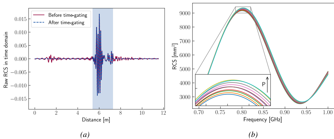
Figure 4.26: RCS of the Slot sensor with a maximum at 803MHz extracted from the algorithm in time-domain (a) and frequency domain (b). The colored area in time-domain correspond to the window applied. The arrow indicates the reading direction for increasing pressure. 10 measurements are taken between 100 and 1000 mbar, in 100 mbar steps.
