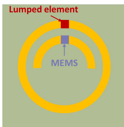
Figure 2.31: CLL antenna used for the analysis of the impact of the electrical size, with the position of the elements
