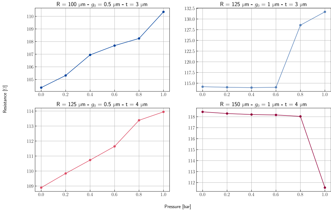
Figure 2.23: Simulated resistance of the MEMS of the second set.
