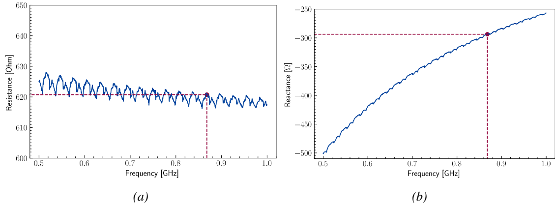
Figure 4.9: Real (a) and imaginary parts (b) of the impedance of one of the 2 MEMS put in parallel as the load of the Slot antenna. The points with the dotted lines correspond to the value of the impedance at 868 MHz. The small periodic variations in the curves are due to the prober used for the characterization of the MEMS. At 868 MHz and 1 bar, the 2 MEMS in parallel have an equivalent impedance of 310.37 - j146.86\Omega .
