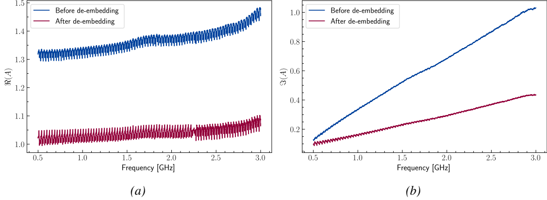
Figure 3.18: Impact of the de-embedding on the real (a) and imaginary parts (b) of the A parameter of the ABCD matrix for the MEMS with dimensions of R = 100\mu\text{m} , h = 3.5\mu\text{m} and g_0 = 0.3\mu\text{m} .
