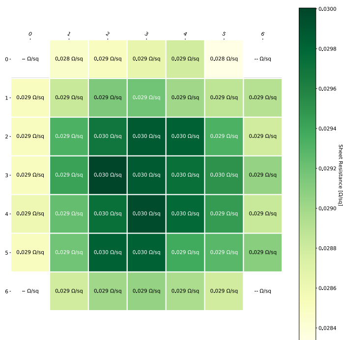
Figure 3.8: Mapping of the sheet resistance of AlCu over a wafer.
