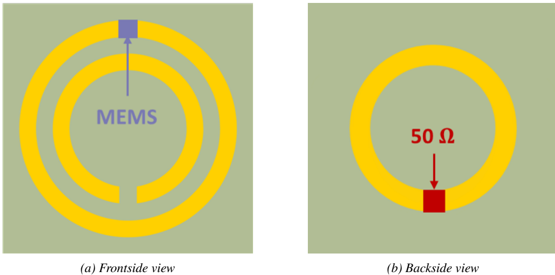
Figure 2.38: Geometry of the miniature antenna based on a SRR excited by a backside loop, with the positions of the load and the MEMS.
