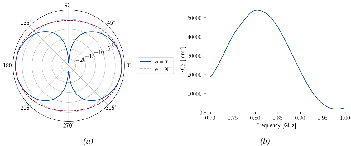
Figure 4.8: Electromagnetic behavior of the Loop. (a) Realized gain of the Loop sensor (in dB) at 1 bar and 868 MHz. (b) RCS of the Loop sensor at 1 bar.
