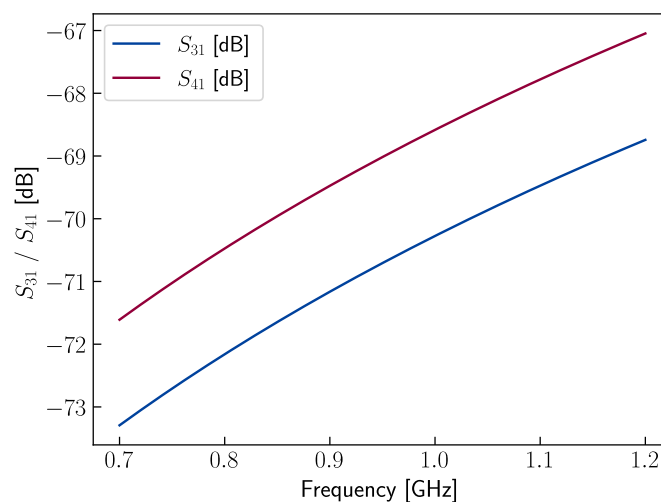
Figure 2.28: Cross-talk between two lines on the same chip separated by 1000 \mu\text{m} between the center of the signal lines.
