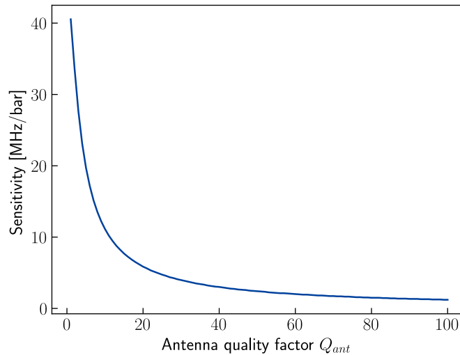
Figure 2.34: Variation of antenna sensitivity with its quality factor.
