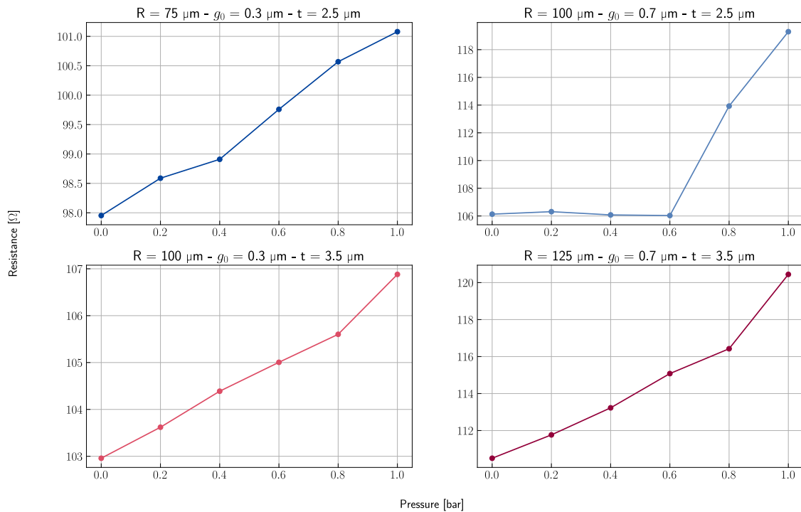
Figure 2.22: Simulated resistance of the MEMS of the first set.
