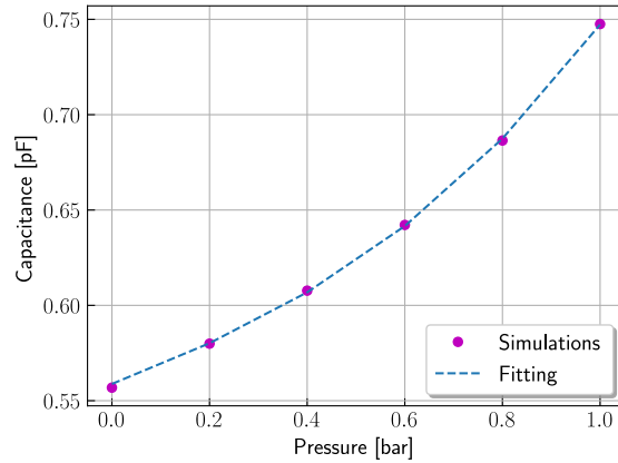
Figure 5.12: Variation of the capacitance of the MEMS with dimensions of ( R = 150\mu\text{m} , t = 4\mu\text{m} , g_0 = 1\mu\text{m} ) with pressure, obtained by simulations on Ansys HFSS. The curve is obtained by a polynomial fitting of order 5.
