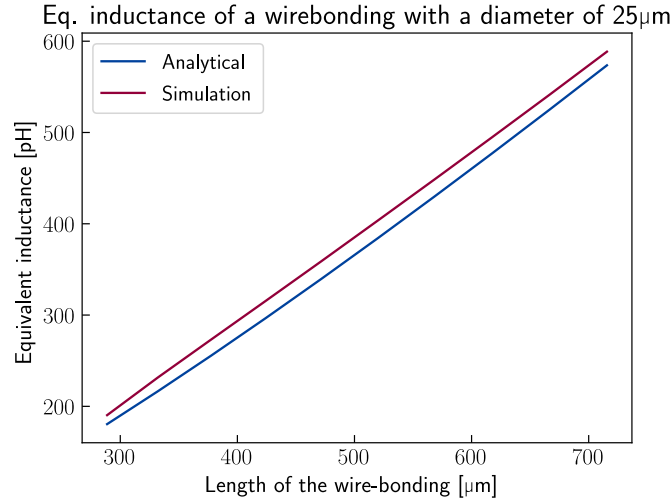
Figure 2.37: Variation of the inductance of a wire-bonding of 25 \mu\text{m} of diameter as function of its length.
