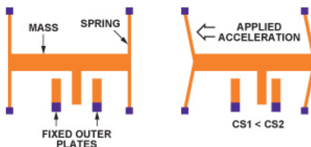
Figure 1.13: Working principle of a 1-axis MEMS accelerometer. The acceleration will move the mobile part, which will change the capacitance at the outer plates.
