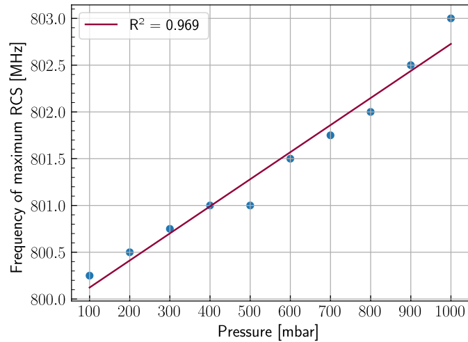
Figure 4.27: Variation of the frequency of the maximum RCS of the Slot sensor at 800 MHz with pressure. The point at 500 mbar is at the same value of frequency than 400 mbar due to the frequency resolution of the interrogation.
