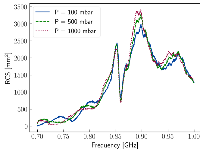
Figure 4.23: Comparison of the raw RCS measurements of the PIFA sensor at 100 mbar, 500 mbar and 1 bar.
