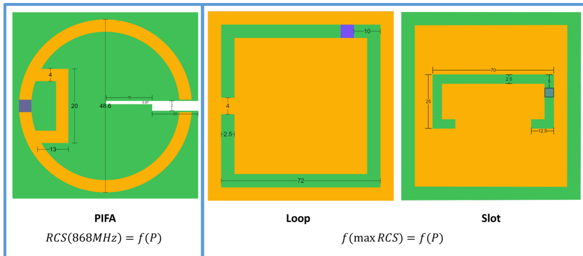
Figure 4.1: Geometries of the antennas, where the yellow part is the copper, the green part the substrate and the blue part the position of the MEMS. The PIFA is designed to study the variation of RCS at 868 MHz and the two others ones the variation of the frequency of maximum of RCS.
