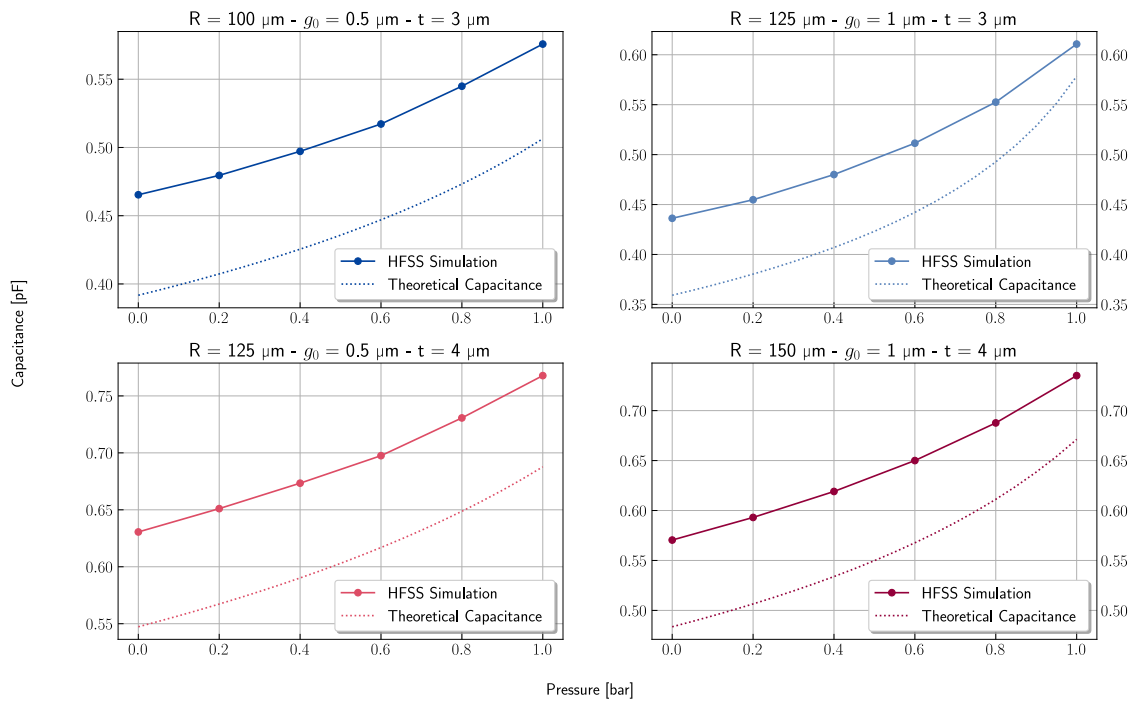
Figure 2.21: Simulated equivalent capacitance of the MEMS of the second set and comparison with analytical results.
