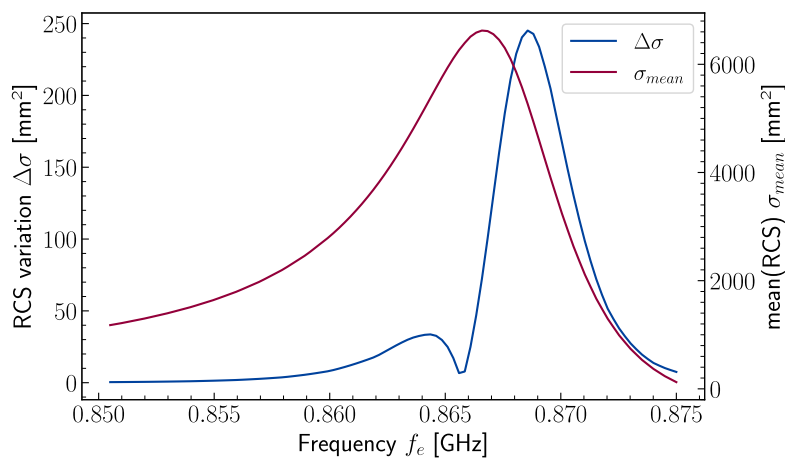
Figure 5.18: Variation of the mean value of the RCS \sigma_{mean} and the variation of RCS \Delta\sigma with the interrogation frequency f_e .
