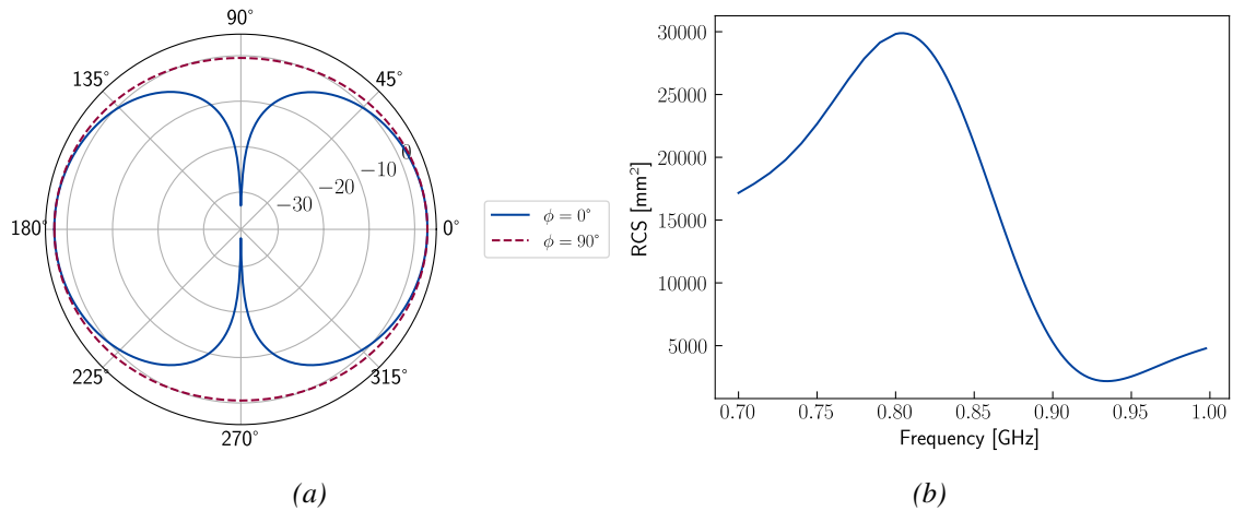
Figure 4.11: Electromagnetic behavior of the Slot. (a) Realized gain of the Slot sensor at 1 bar and 868 MHz. (b) RCS of the Slot sensor at 1 bar.
