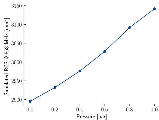
Figure 4.5: Simulated RCS at 868 MHz versus pressure for the PIFA sensor.
