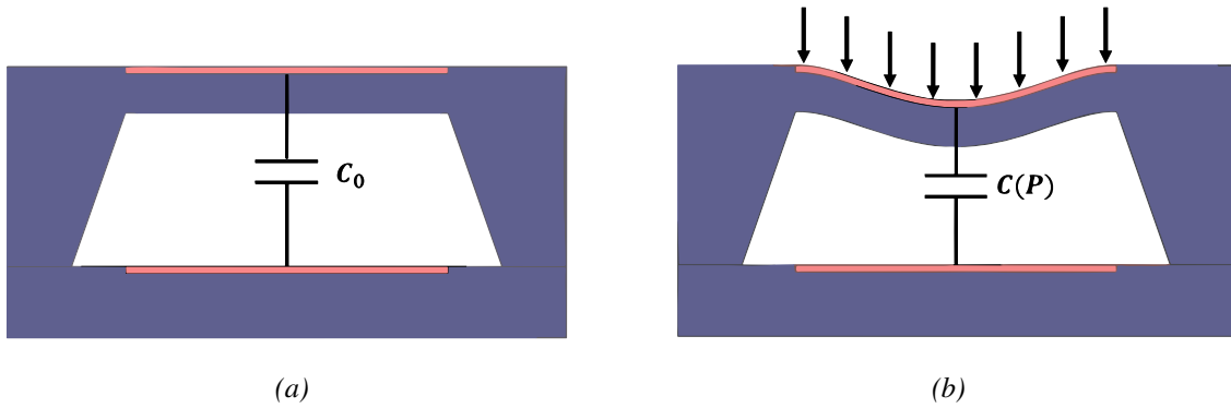
Figure 2.1: Working principle of the capacitive pressure sensor: under vacuum (a), the membrane and the bottom electrode are parallel, while applying a pressure on the membrane (b), it will deflect and change the value of the capacitance.
