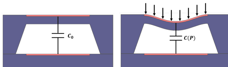
Figure 1.15: Operating principle of a capacitive pressure sensor. The membrane will deflect due to applied pressure. The deflection changes the value of the capacitance between the two electrodes (in pink).
