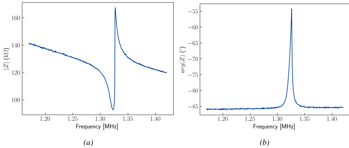
Figure 5.22: Modulus (a) and argument (b) of the non-metallized MEMS impedance under vacuum with electrostatic actuation. The ENA was calibrated using an Open-Short-Thru-Load calibration. The measured quality factor under vacuum, extracted thanks to a MBVD fitting, is 271.
