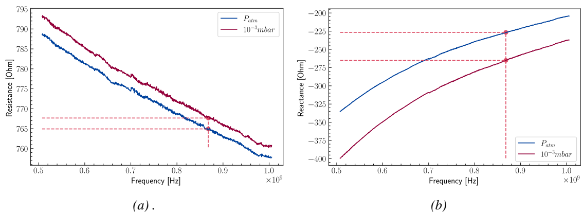
Figure 3.24: Resistance (a) and reactance (b) of a MEMS with R = 100\mu m , h = 3.5\mu m and g_0 = 0.3\mu m as function of pressure. The dotted line highlights the resistance and reactance of the MEMS at 868 MHz.
