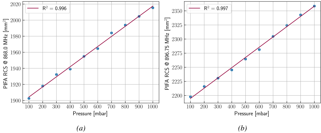
Figure 4.29: Variation of the RCS of the PIFA sensor at 868 MHz (a) and at 896.75 MHz, the peak of the frequency response (b).
