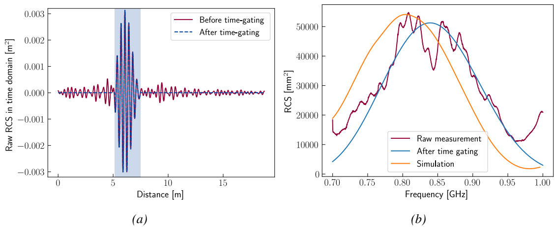
Figure 4.16: Time-domain (a) and frequency (b) response of the Loop and comparison with the simulation. The colored area correspond to the window applied.
