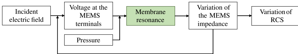
Figure 5.5: Block diagram of the interrogation of resonant MEMS using intermodulation, with the current step of the calculation highlighted. This section focuses on determining an expression for the pressure-dependent mechanical resonance frequency of the membrane, and establishing the equation of motion of the membrane under the application of a pressure and an electrostatic force.
