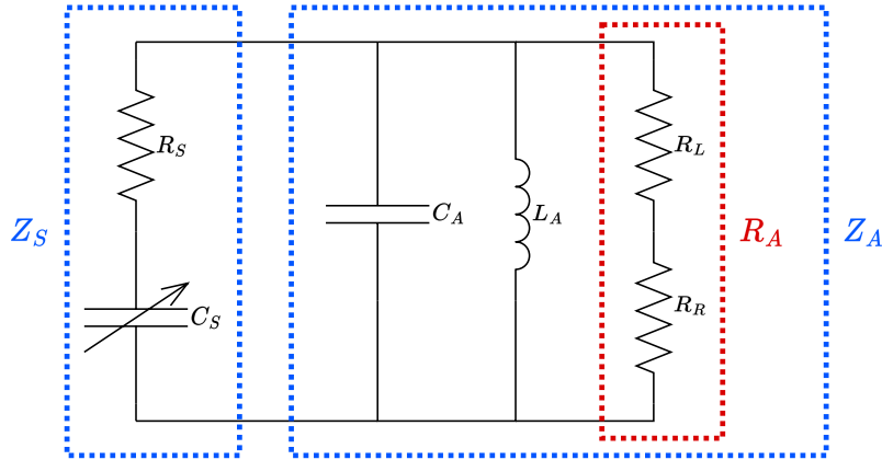
Figure 5.9: Equivalent circuit of a sensor used for the simplified model. The parallel RLC representation is used to represent the input impedance of the antenna around the antiresonance.
