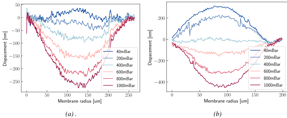
Figure 3.25: Measurement of the profile of MEMS with a metallized membrane (a) and a non-metallized membrane (b), at different level of pressure.
