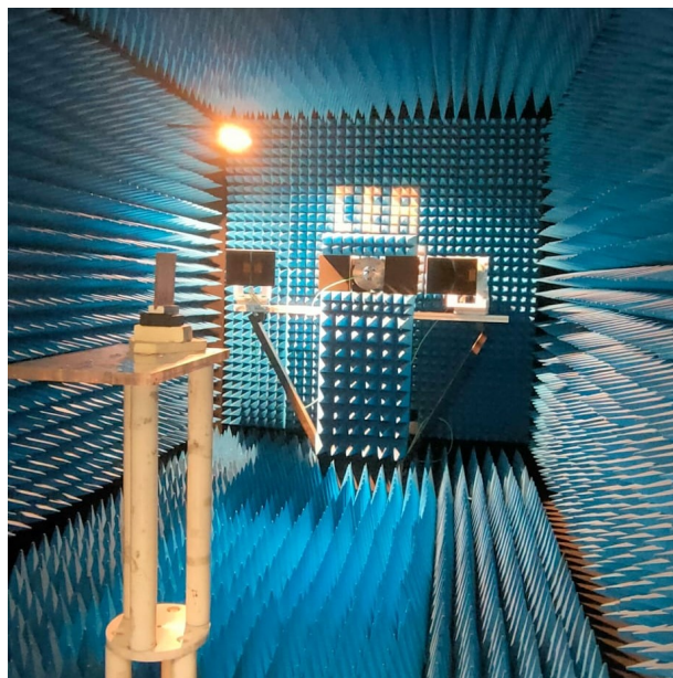
Figure 4.13: CEA-Leti anechoic chamber, for measurements up to 40 GHz, with the sensor to characterize in frequency placed on the support.
