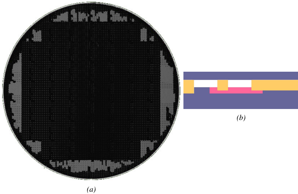
Figure 3.3: In-line characterization of the bonding of the wafers. (a) SAM full-wafer view after the bonding. The light areas show where the wafer is not correctly bonded to the SiO 2 . (b) Side view of the MEMS at the corresponding step.
