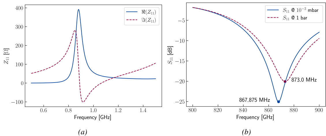
Figure 4.10: Electrical properties of the Slot sensor: (a) Input impedance of the Slot antenna at the location of the MEMS. (b) Reflection coefficient between the antenna and the MEMS.
