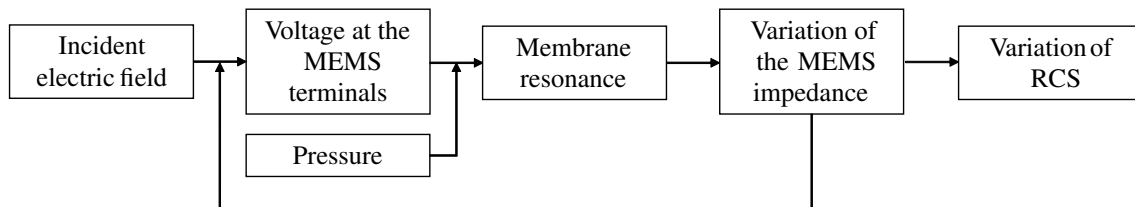
Figure 5.2: Block diagram of the interrogation of resonant MEMS using intermodulation. Two signals at f_0 and f_0 + f_\Delta with f_\Delta \ll f_0 are sent to the sensor. Due to the non-linear aspect of the electrostatic force, the MEMS is put in mechanical resonance at f_\Delta . This resonance modulates the backpropagated signal by adding peaks in the spectrum received back by the reader. Only the two first intermodulation peaks are considered here.
