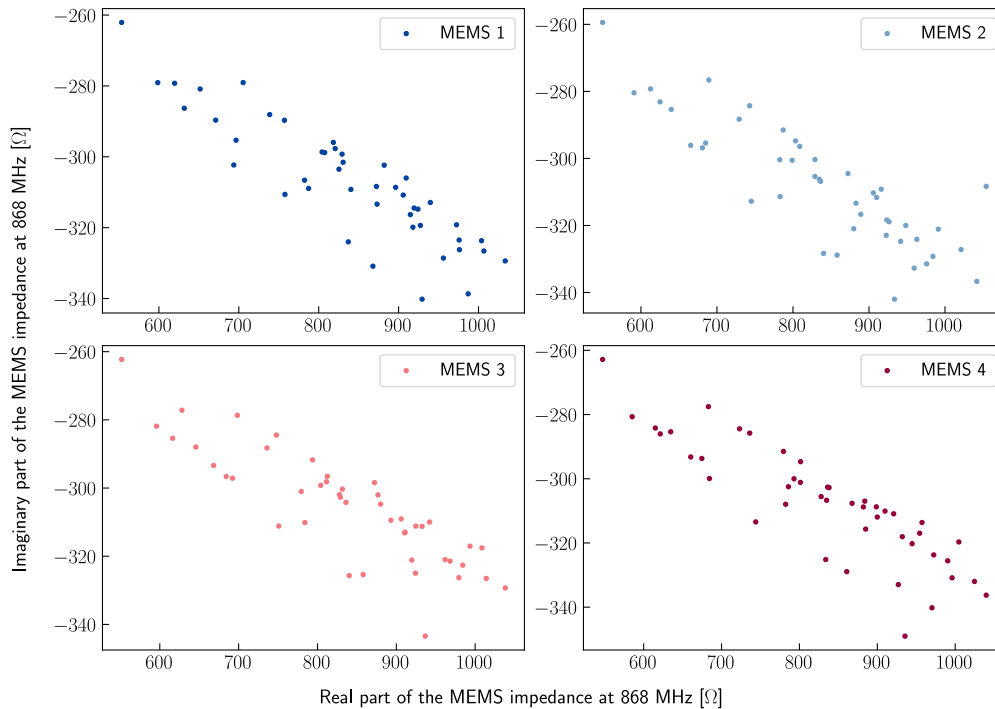
Figure 3.21: Plot of the relationship between the resistance and the reactance at 868 MHz of 4 MEMS with the same geometries over the wafer. A correlation between the value of the resistance and the reactance is observed.
