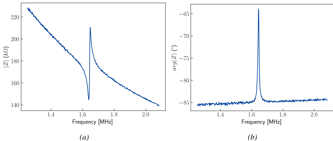
Figure 5.23: Modulus (a) and argument (b) of the metallized MEMS impedance under vacuum with electrostatic actuation. The ENA was calibrated using an Open-Short-Thru-Load calibration. The measured quality factor under vacuum, extracted thanks to a MBVD fitting, is 184.
