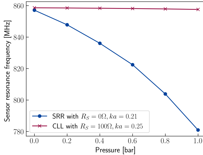
Figure 2.39: Variation of the resonance frequency of the SRR antenna with the MEMS as a perfect capacitance
