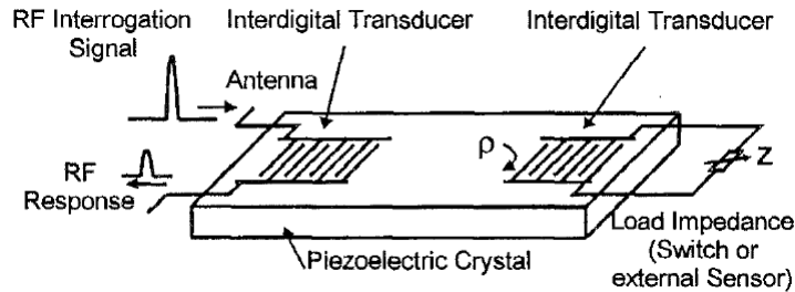
Figure 1.6: Representation of an external sensor connected to a SAW device. The sensor impedance will change the reflection coefficient of the interdigital transducer. [15]
