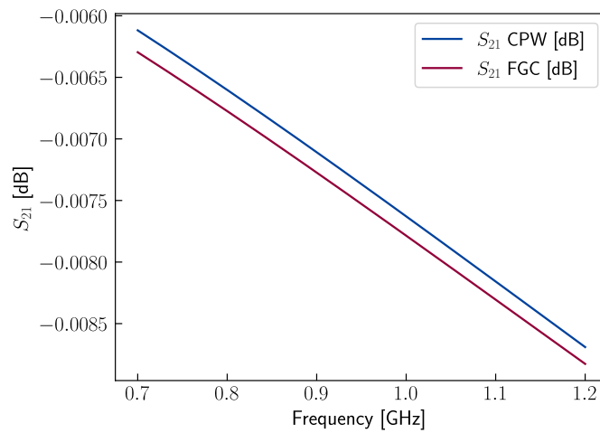
Figure 2.26: Transmission properties of the two types of lines
