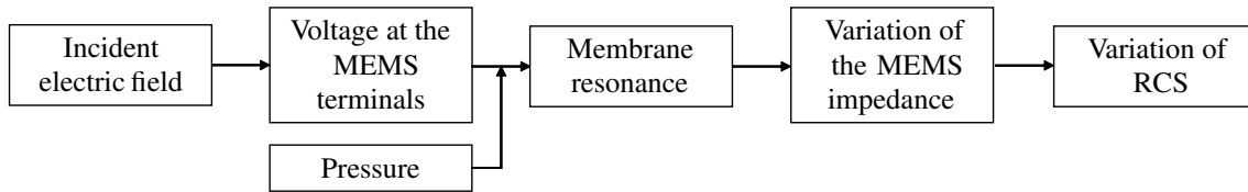
Figure 5.10: Simplified block diagram of the interrogation of resonant MEMS using intermodulation. The feedback loop is no longer present due to the approximation of constant voltage.
