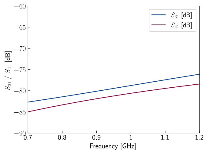
Figure 2.30: Cross-talk between two MEMS on the same chip separated by 1000 \mu\text{m} between the center of the signal lines.
