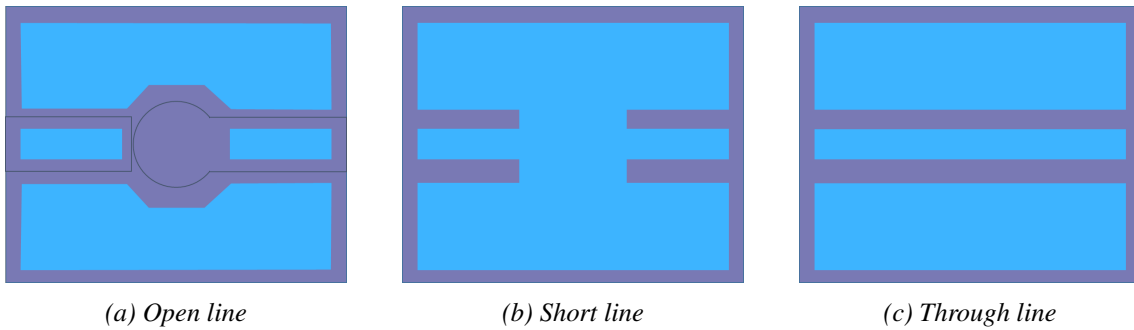
Figure 2.17: Variants of RF test structures on the wafer.
