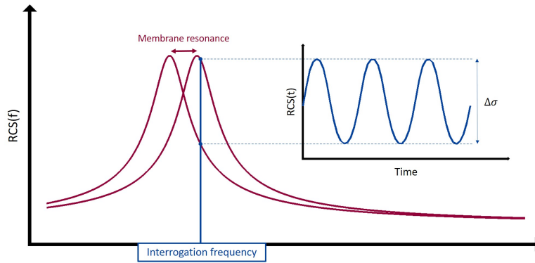
Figure 5.19: Illustration of the impact of the resonance of the MEMS on the RCS while interrogated at a frequency different than the maximum of RCS. The vibration of the membrane periodically shift the frequency response of the antenna, which periodically changes the value of the RCS at the interrogation frequency.
