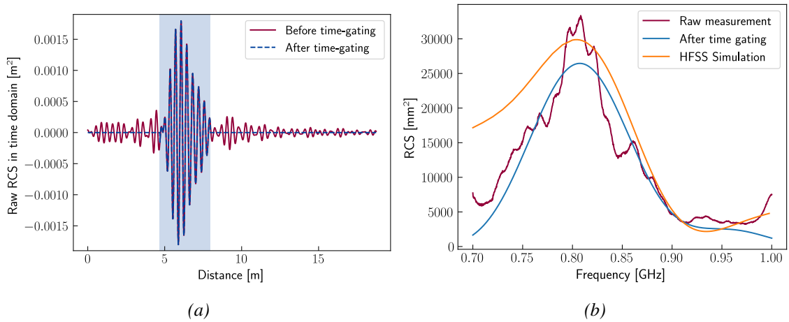
Figure 4.15: Time-domain (a) and frequency (b) response of the Slot and comparison with the simulation. The colored area correspond to the window applied.
