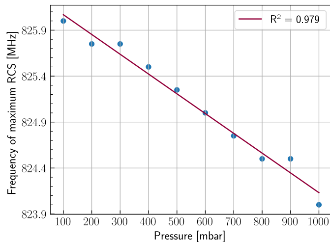
Figure 4.25: Variation of the frequency of maximum RCS of the Loop sensor with pressure. The points at 300 and 900 mbar are at the same frequencies at the previous ones due to the frequency resolution of the interrogation.
