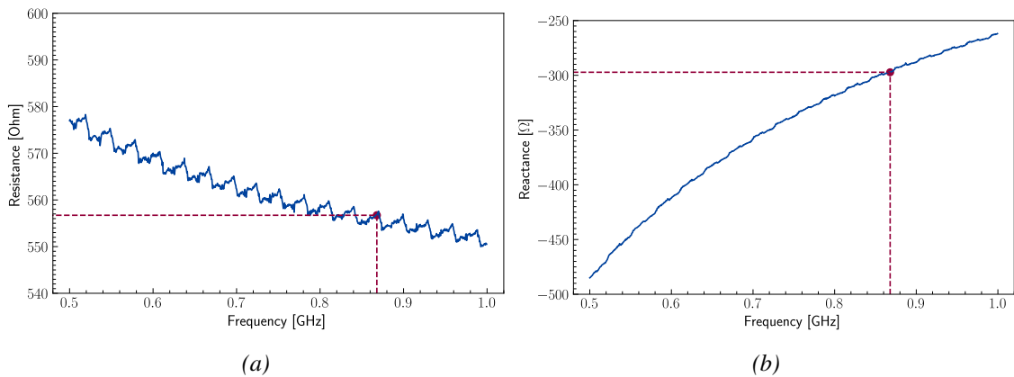
Figure 4.6: Real (a) and imaginary parts (b) of the impedance of one of the 4 MEMS put in parallel as the load of the Loop antenna. The points with the dotted lines correspond to the value of the impedance at 868 MHz. The small periodic variations in the curves are due to the prober used for the characterization of the MEMS. At 868 MHz and 1 bar, the 4 MEMS in parallel have an equivalent impedance of 139.18 - j74.31\Omega .
