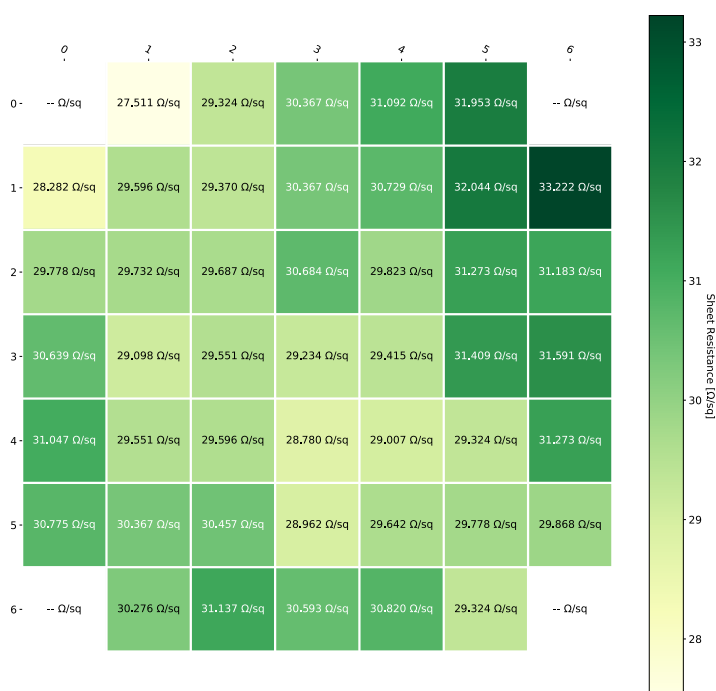
Figure 3.9: Mapping of the sheet resistance of the implant of the lower electrode over a wafer.
