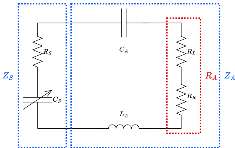
Figure 5.4: General equivalent circuit of a receiving antenna loaded by a MEMS.
