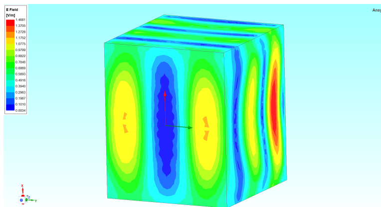
Figure 4.19: Magnitude of the electric field at the surface of the vacuum chamber at 3 GHz.
