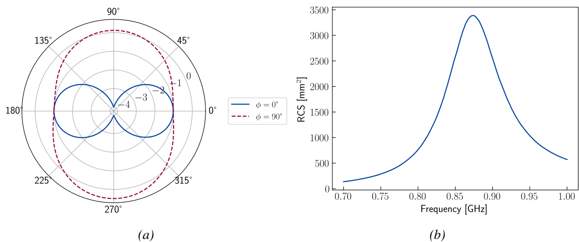
Figure 4.4: Electromagnetic behavior of the PIFA. (a) Realized gain of the PIFA sensor at 1 bar and 868 MHz. (b) RCS of the PIFA sensor at 1 bar.
