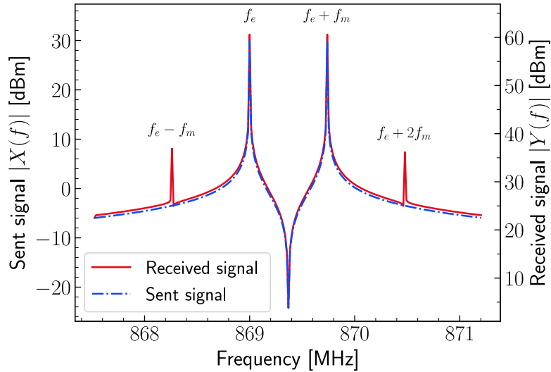
Figure 5.17: Example of FFT of sent and received signal under the conditions presented in section 5.6.1 calculated with the complete model.
