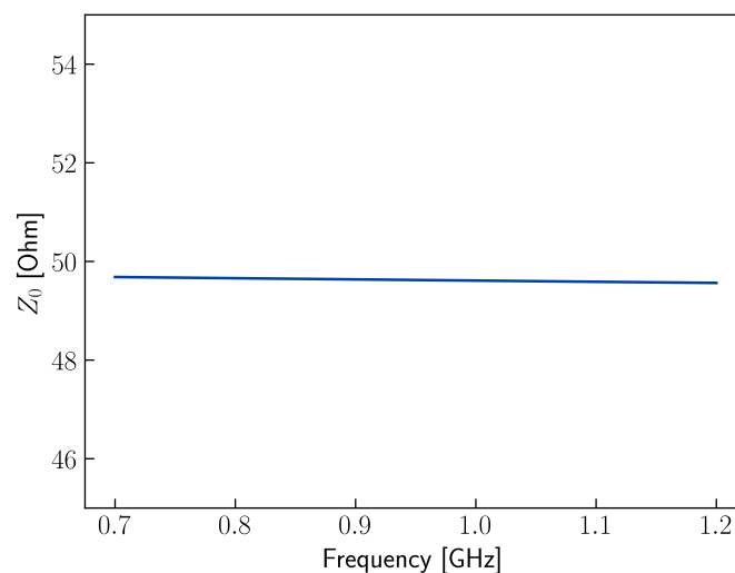
Figure 2.24: Characteristic impedance of a 1mm-long line
