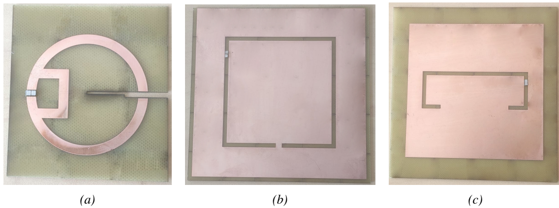
Figure 4.12: Pictures of the sensors, where the antenna is made of copper over FR4. The MEMS are wire-bonded to the antennas. (a) PIFA sensor (b) Loop sensor (c) Slot sensor.
