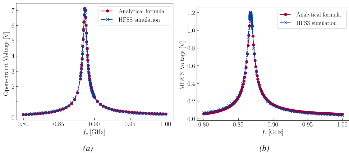
Figure 5.15: Comparison between simulation and analytical formula for the open-circuit voltage (a) and the voltage at the MEMS terminals (b).
