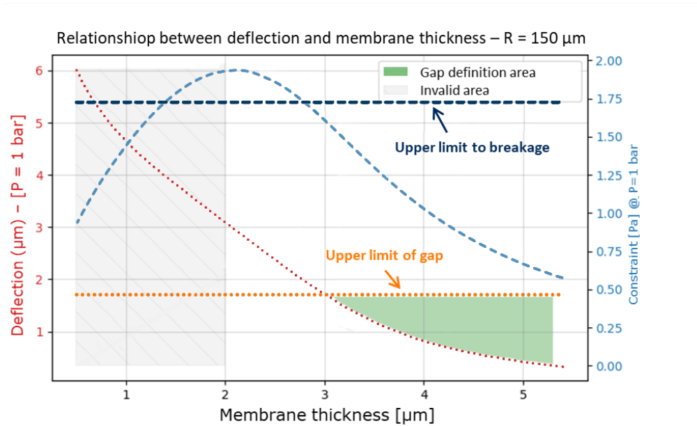
Figure 2.3: Example of curves used to determine MEMS dimensions sets for a radius R = 150\mu\text{m} . The green area represents the zone where the thickness (in x-axis) and the gap (in y-axis) can be extracted. In this area, the triplet (R, g_0, h) are considered as valid, as the deflection (red curve) is lower than the upper limit of the gap (orange line), and the stress (blue curve) is lower than the upper limit to breakage (dark blue line).
