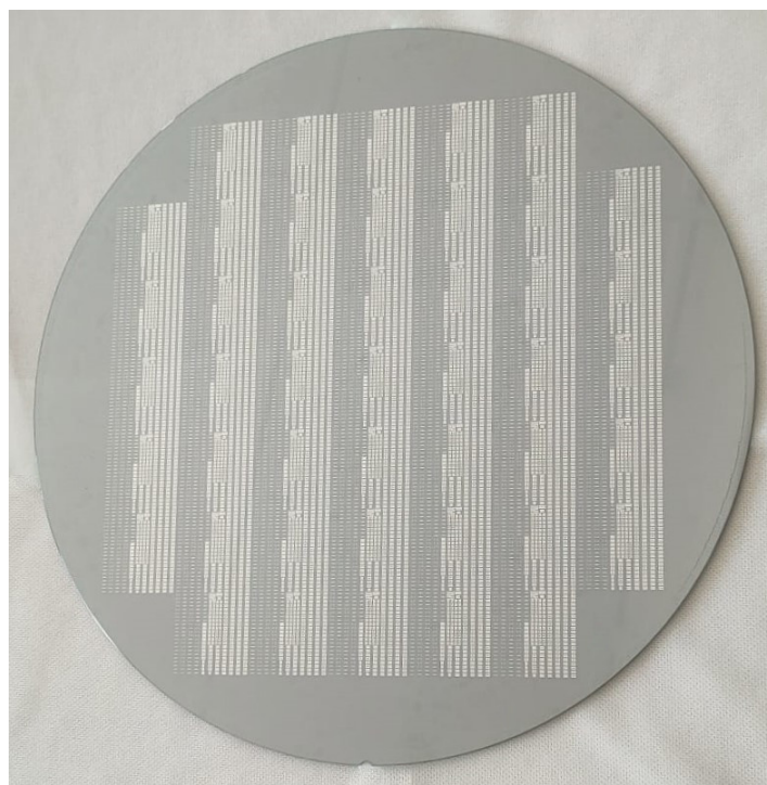
Figure 3.1: Picture of one of the wafers
