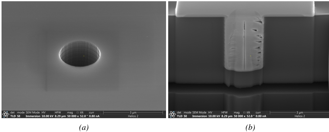
Figure 3.5: (a) Zoomed-in view of the hole in the membrane. (b) View of the depth of the etching of the hole. The hole is not fully etched.
