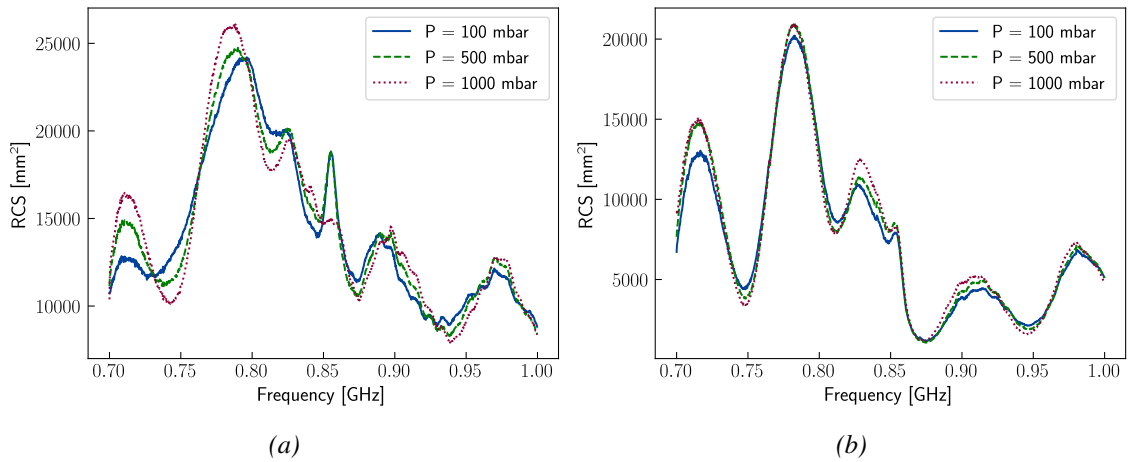
Figure 4.20: Comparison of the raw RCS measurements of the Loop (a) and Slot (b) sensors at 100 mbar, 500 mbar and 1 bar.
