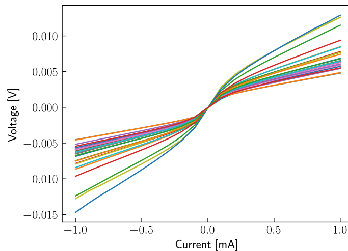
Figure 3.14: IV curves for all the contact resistances of a wafer with the correction steps.
