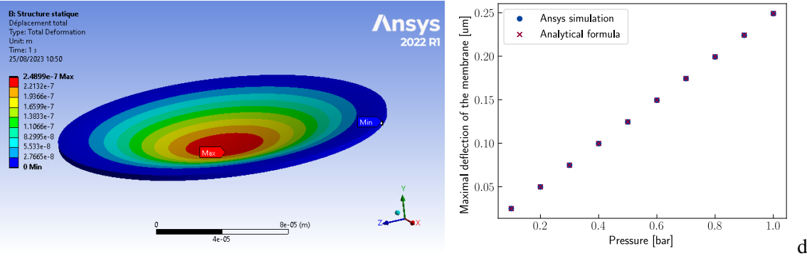
Figure 2.4: Simulation on Ansys Mechanical of the deflection of the membrane of the MEMS with dimensions of (R = 100\mu\text{m}, g_0 = 0.3\mu\text{m}, h = 3.5\mu\text{m}) at 1 bar and comparison between the maximal deflection extracted from simulation and from equation 2.2.
