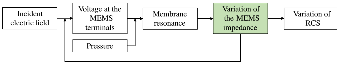
Figure 5.7: Block diagram of the interrogation of resonant MEMS using intermodulation, with the current step of the calculation highlighted. This section focuses on determining the expression of the capacitance variation and the impedance mismatch between the MEMS and the antenna.
