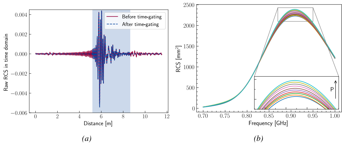
Figure 4.28: RCS of the PIFA sensor extracted from the algorithm in time-domain (a) and frequency domain (b). The colored area in time-domain correspond to the window applied. The arrow indicates the reading direction for increasing pressure. 10 measurements are taken between 100 and 1000 mbar, in 100 mbar steps.
