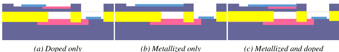
Figure 2.15: Variants of membrane stacks
