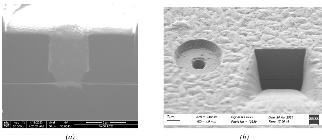
Figure 3.15: Observations after etching holes using FIB to create a reference MEMS. (a) FIB image of the first etching test. It creates deposition of materials at the bottom of the hole. (b) SEM image of a hole etched using FIB next to the hole created during the microfabrication.
