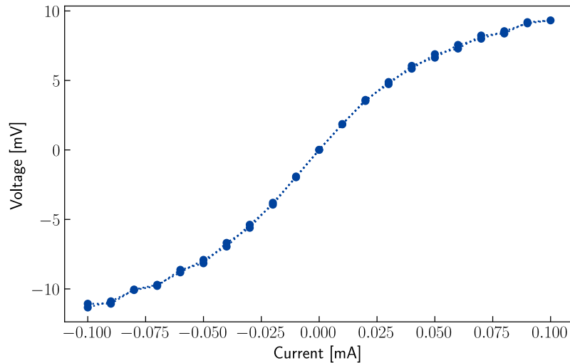
Figure 3.11: Intensity-Voltage (IV) curve for one contact between the metal and the lower implant.
