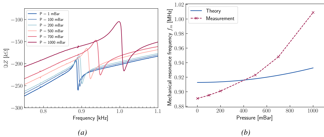
Figure 5.20: Example of variation of resonance frequency of a MEMS with pressure. (a) Imaginary part of the MEMS impedance with pressure, the resonance occurs when the curve decreases. (b) Variation of resonance frequency with pressure, the theoretical curve was calculated using Eq (5.17).
