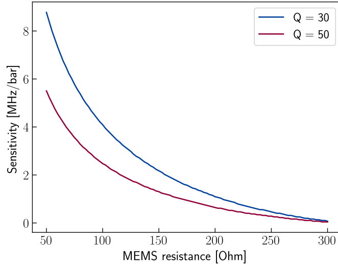
Figure 2.35: Variation of the sensitivity \Delta f with the resistive part of the impedance of the MEMS R_S for two values of the quality factor.
