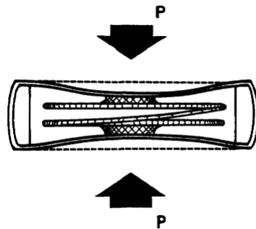
Figure 1.2: LC pressure sensor proposed by Collins [6], which consist of two coils trapped between two membranes. The pressure brings the coils closer together and changes the capacitance between them.
