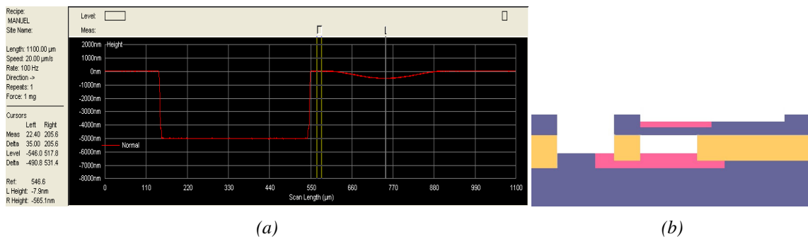
Figure 3.2: In-line characterization of the etching of the membrane. (a) Measurement of the topography of the MEMS using a profilometer after the etching of the membrane shown in Figure 2.13. (b) Side view of the MEMS at the corresponding step.
