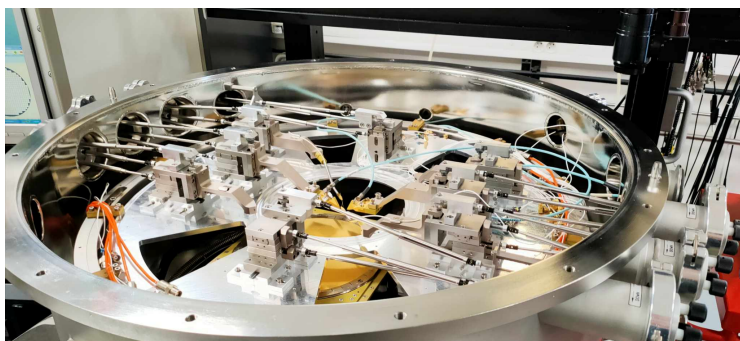
Figure 3.22: View of the inside of the vacuum chamber of the PAV2000 prober.
