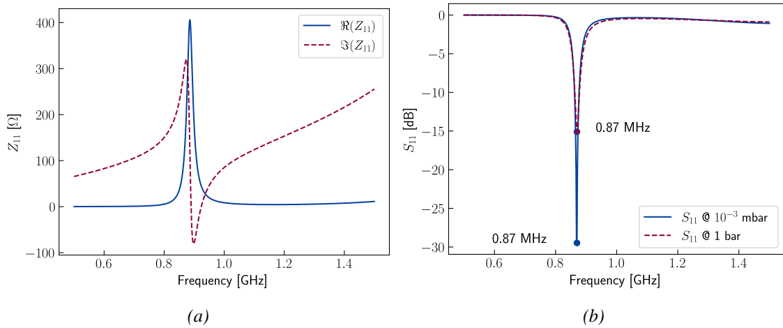
Figure 4.3: Electrical properties of the PIFA sensor. (a) Input impedance of the PIFA antenna at the location of the MEMS. (b) Reflection coefficient of the antenna loaded by the MEMS.
