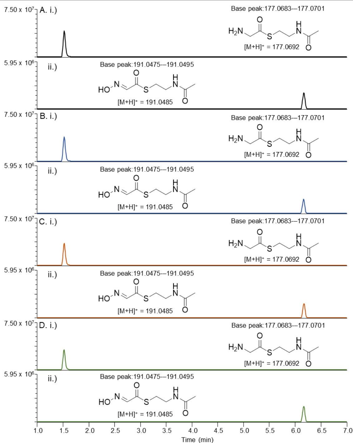
Figure S41. Base peak analyses for enzyme activity assays with LbmA-Ox E1680Q, with the intensities scaled to the maximum value of assay set 1. A–D) Shown are extracted ion chromatograms (EICs) of UHPLC-MS data of quadruplicate analyses for i) GlySNAC substrate 6 and ii) GlySNAC oxime product 7 .
