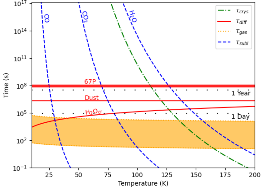
Figure 3.2: Characteristic timescales of the main physical processes taking place in a comet’s nucleus: (a) Crystallization of amorphous \text{H}_2\text{O} ice denoted by the green dashed dotted line, (b) Sublimation of different volatile species denoted by the blue dashed lines, (c) Gas diffusion within the pores for pores’ radius between 10^{-3} and 10^{-6} denoted by the orange dotted lines and the orange shaded area, (d) Heat diffusion in nucleus of different compositions: pure dust, pure crystalline \text{H}_2\text{O} ice and a nucleus with characteristics resembling those of comet 67P/Churyumov-Gerasimenko. The black loosely dotted lines serve as indicators for the timescales.
