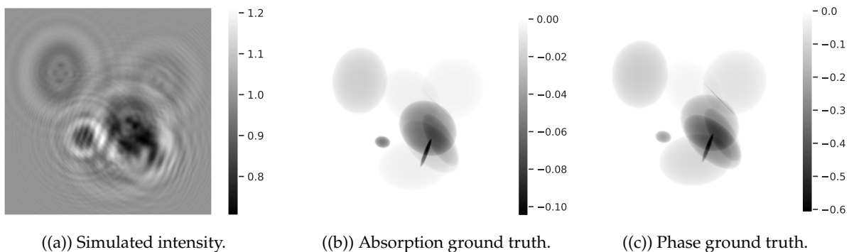
Figure 4.4.: Example of one simulated pair.
