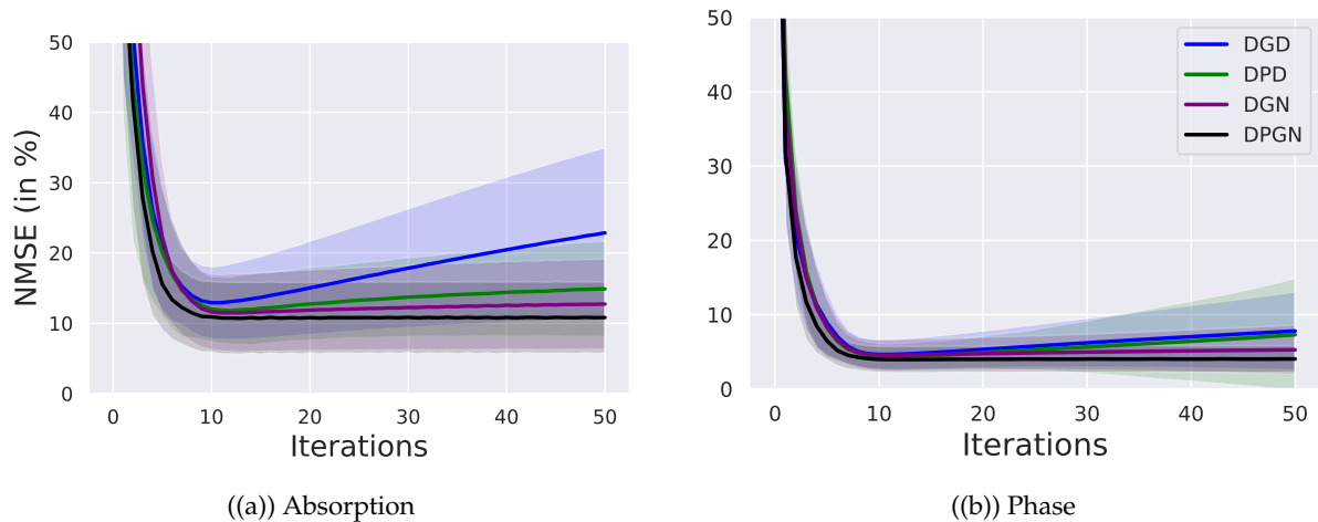
Figure 5.12.: Evolution of average NMSE (%) of the unrolling approaches for 1 000 test images when running for 50 iterations. The transparent areas correspond to the standard deviation.
