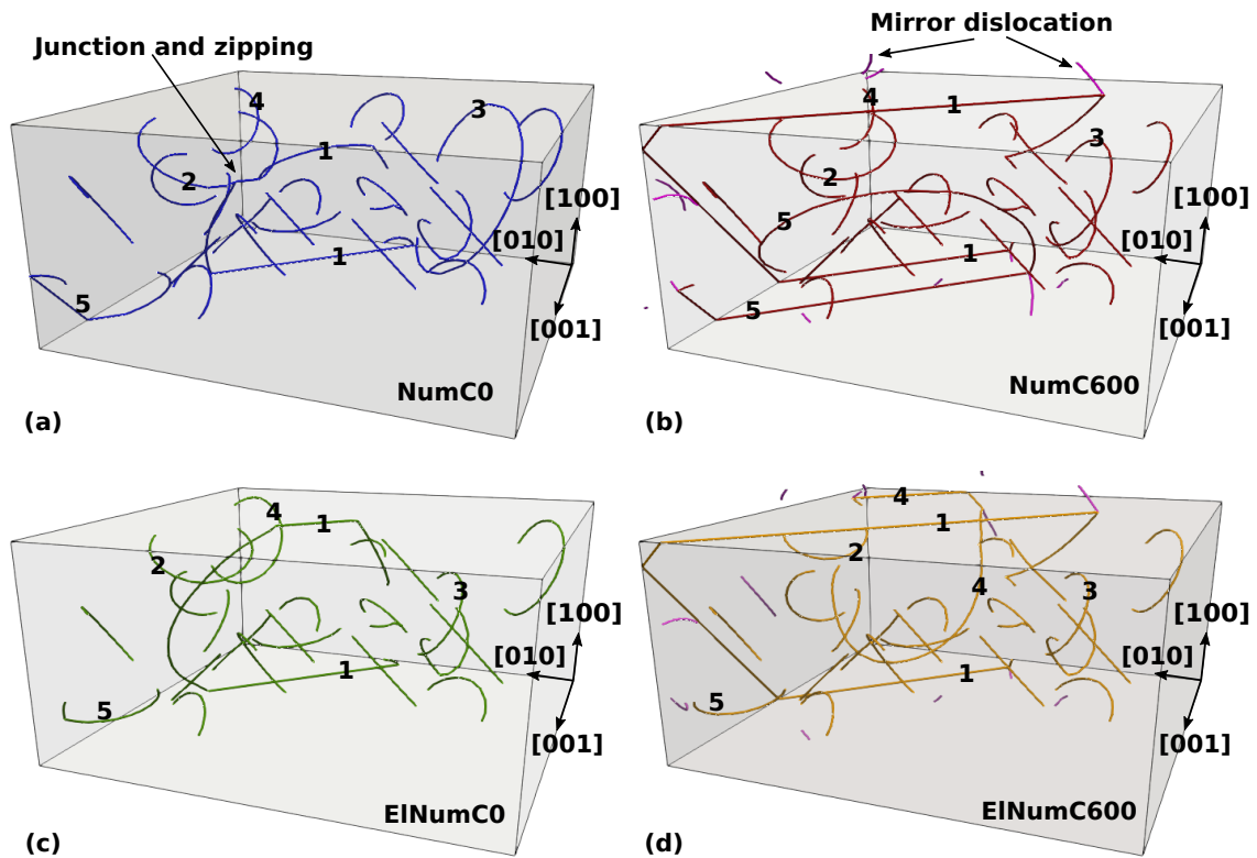
Figure 4.22: Evolution of the dislocation microstructure at the yield point for NumC0 (a), NumC600 (b), ENumC0 (c) and ENumC600 (d). The pink dislocations represent mirrored dislocation constructed with a cutoff of 600 Å. The most important dislocations are identified with number labels.
