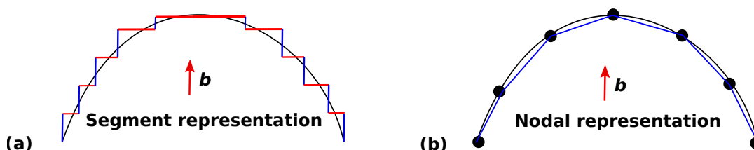
Figure 2.1: DDD Dislocation line discretization, (a) lattice-based approach where the dislocation line is discretized into segments (edge/screw model), (b) nodal-based approach with a discretization of the dislocation into curves of various orientation with respect to the Burgers vector.
