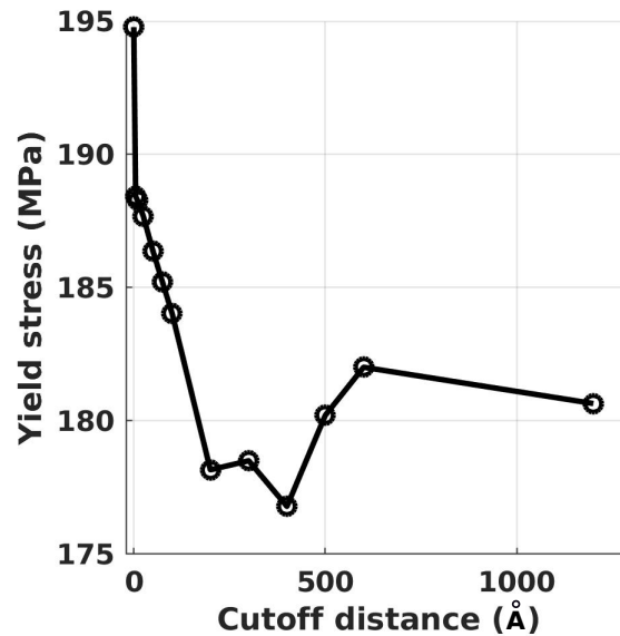
Figure 4.26: Yield stress as a function of the cutoff distance for the 0.25 \mu\text{m} thin film.
