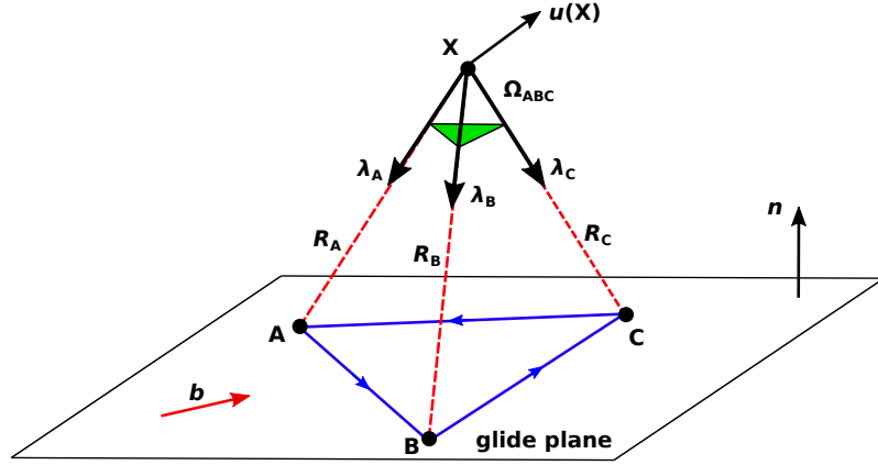
Figure 2.5: Triangular dislocation loop ABC used to calculate the displacement field u at point X with Barnett formulation considering the contribution of the solid angle \Omega_{ABC} .
