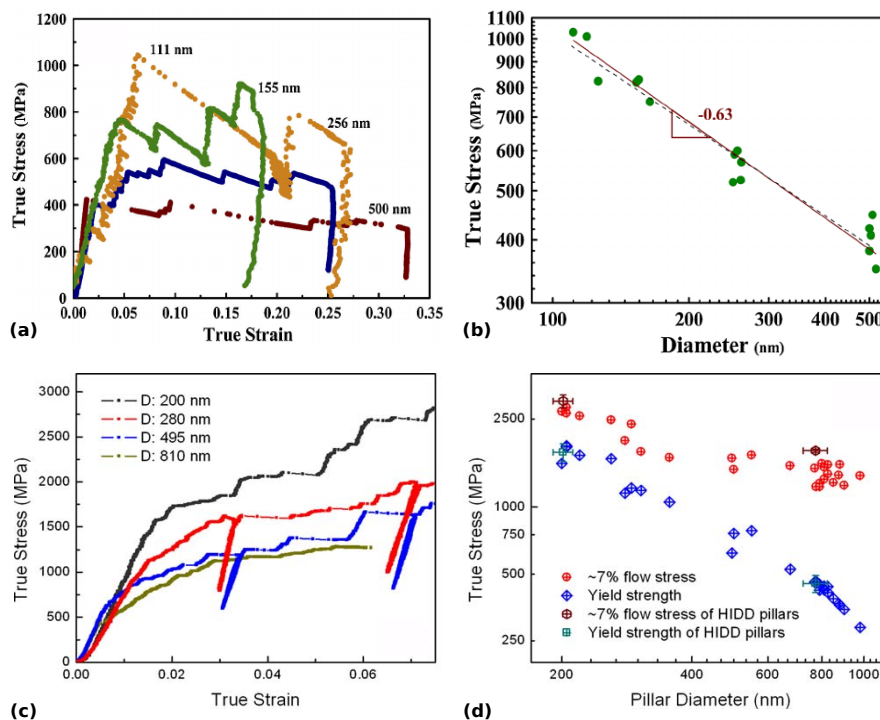
Figure 1.7: Submicronic pillars compression of FCC and BCC metals. Stress-Strain curve for Cu (a) and Mo (c) nanpillars of different diameters showing the “smaller is stronger” trend. Yield stress vs. pillar diameter for Cu (b) and Mo (d) with slopes -0.63 and -0.44 respectively. Images from [JEN 10] and [KIM 08].
