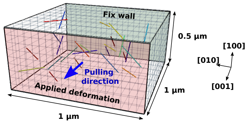
Figure 4.16: El-Numodis thin film simulation setup. The sample consists in a copper thin film of 0.5 \mu\text{m} thickness and 1.0 \mu\text{m} lateral sizes with cubic orientation in which FR sources are randomly distributed in various \frac{1}{2}\langle 110 \rangle \{111\} slip systems.
