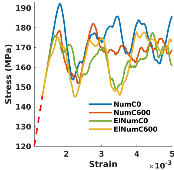
Figure 4.21: Stress-strain curves for a 0.5 \mu\text{m} thick thin film under tension using Numodis and El-Numodis with and without the pseudo-mirror image construction (NumC0/EINumC0 from one side, NumC600/EINumC600 from the other).
