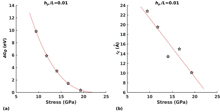
Figure 5.13: Examples of activation parameter fits in function of the shear stress ( i.e. , half the compressive stress) with (a) \Delta G_{i,0} using a Kocks law and (b) r_{c,i} using a linear equation.
