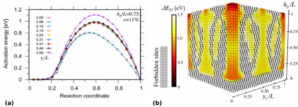
Figure 1.16: Dislocation nucleation in MgO NCs using NEB and TST, (a) Example of SDN energy barrier as function of site localization at 11 % strain. (b) Energy map for SDN in MgO NCs projected on the more probable nucleation centers. The gray colors shows the forbidden sites. Images from [AMO 21a].
