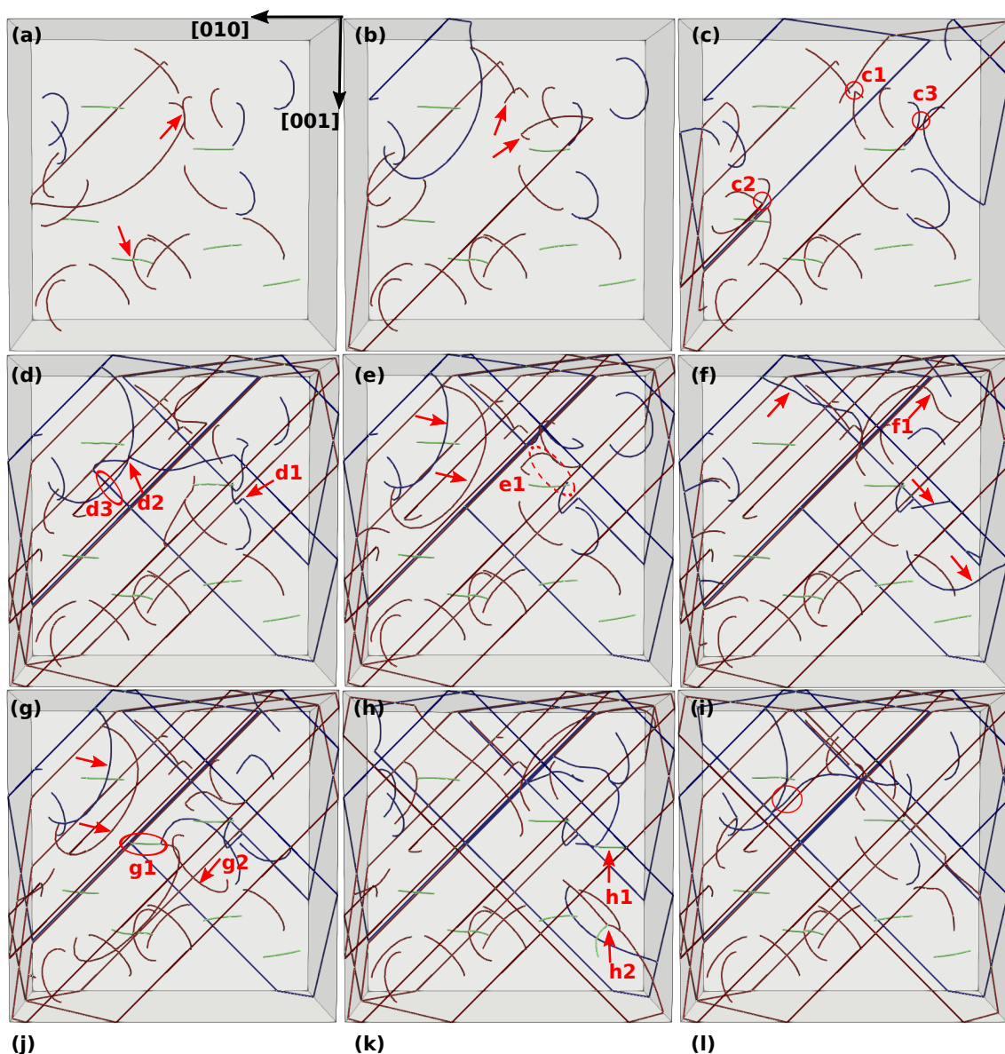
Figure 4.20: Snapshots of the simulation of a 0.5 \mu\text{m} thin film using a cutoff distance of 600 \text{ \AA} . The snapshots matches the marks on the stress-strain curve of Figure 4.19. The arrows and marks are used as guide to the description in the text. Dislocations are colored as follow: slip systems with index 5 and 11 are in blue, indices 2, 6 and 9 are in green and indices 1, 3, 4, 7, 8 and 10 are in red.
