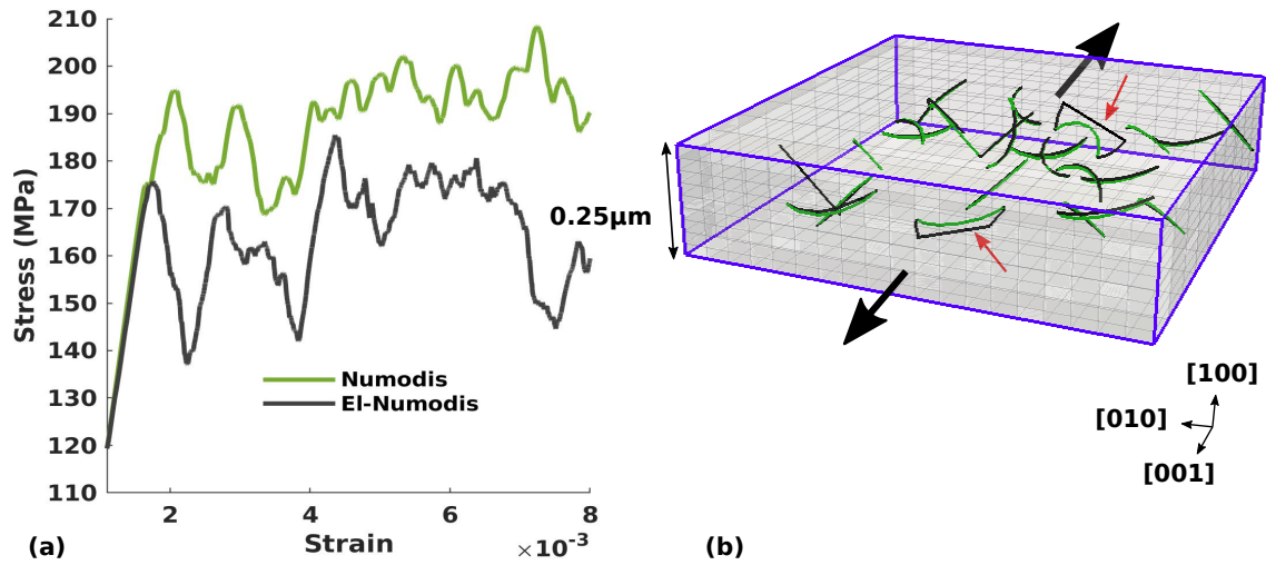
Figure 4.25: Deformation of the 0.25 \mu\text{m} thick thin film under tension using Numodis and EI-Numodis using the pseudo-mirror image construction in EI-Numodis simulation only with a cutoff of 600 \text{ \AA} . (a) stress-strain curves, (b) dislocation microstructure at the yield point.
