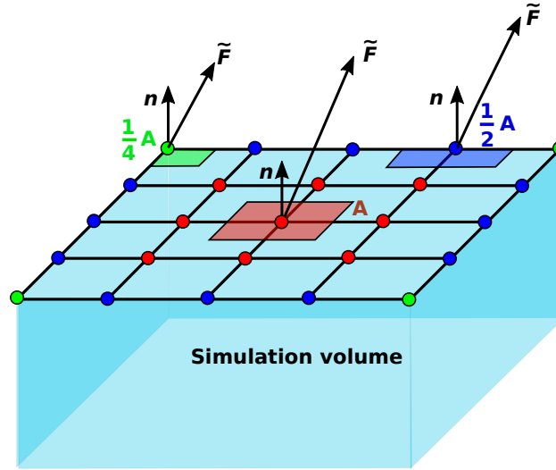
Figure 3.4: stress-to-force conversion. The volume is discretized using eight nodes hexahedron elements. Three different weighted area are present corresponding to nodes that are at the middle ( A ) of the grid, at the corners ( \frac{A}{4} ) or at the edges ( \frac{A}{2} ). Only the mesh at the surface is shown here for simplicity.
