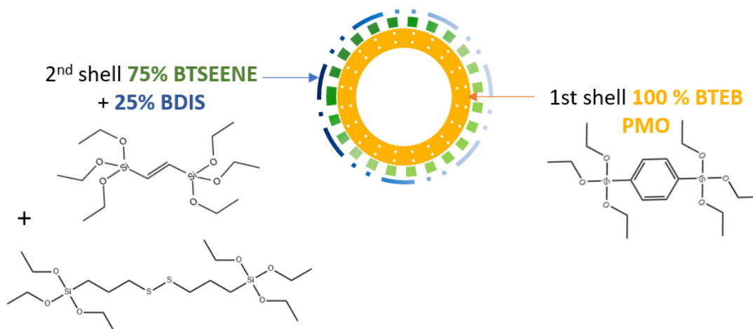
Figure II.51 Representative scheme of the double-shell PMO nanoplatfom.
