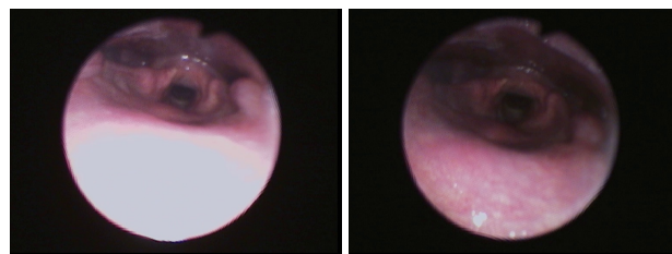
FIGURE 3.2 – K-Snare Inward [ \downarrow\widehat{kL} ] - Sujet CJ
