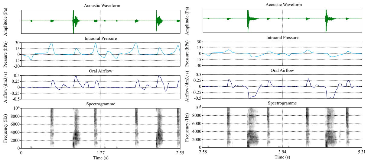
(a) [b' ts' ʔʔ]: ts' b' b' ts' ʔʔ]: ts'
