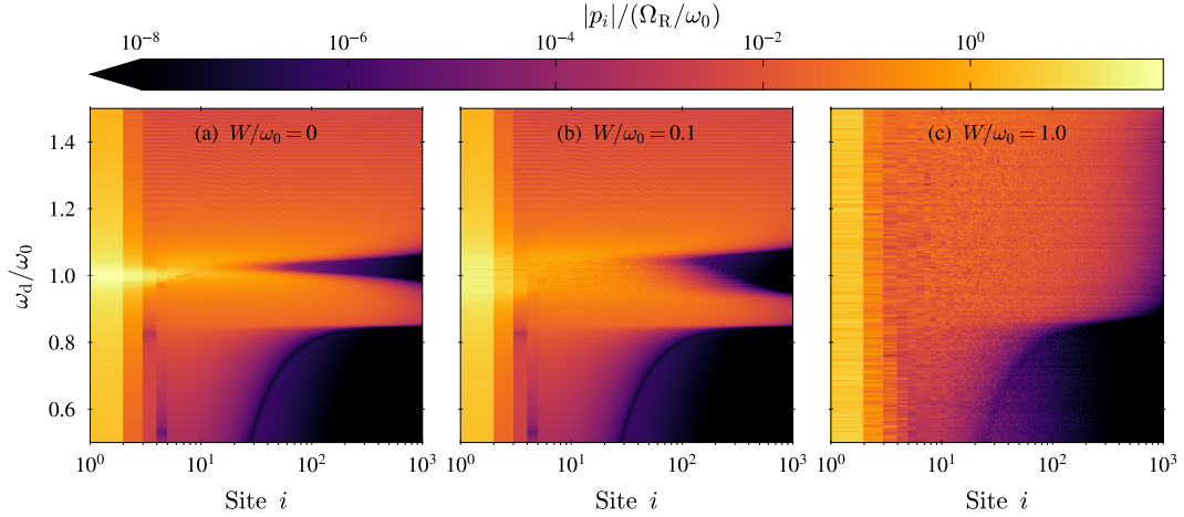
Figure 3.20: Influence of the driving frequency. Density plots of the steady-state amplitude of the dipole moment |p_i| in units of the reduced Rabi frequency \Omega_R/\omega_0 , as a function of both the site i and the driving frequency \omega_d/\omega_0 . Three cases are presented: (a) Without disorder, (b) W/\omega_0 = 0.1 , and (c) W/\omega_0 = 1 . The dipole losses \gamma/\omega_0 = 0.02 , the cavity height L_x/a = 12 , and the data have been averaged over 100 disorder realizations.
