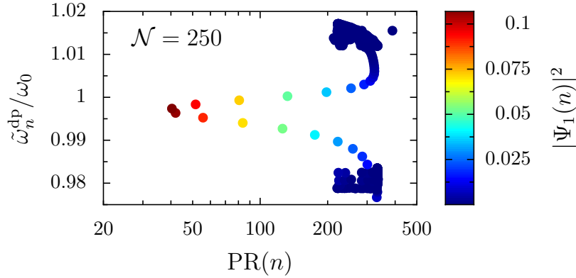
Figure 4.11: Polaritonic edge states participation ratio. Real-space polaritonic eigenfrequencies \tilde{\omega}_n^{\text{dp}}/\omega_0 as a function of the participation ratio \text{PR}(n) , as defined in Eq. (4.66). The color scale represents the corresponding probability density on the first site, i = 1 , of the chain. In the figure, the cavity height L_x = 10a , the dimerization parameter \epsilon = 0.25 , and the chain is comprised of \mathcal{N} = 250 dimers.
