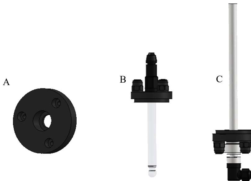
Figure 35 Reservoir cap fundamental design (A) with attached HPS fittings and pH meter on the top cap (B) and temperature sensor on the bottom cap (C)
