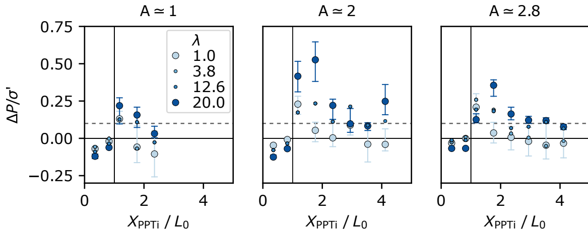
Figure 6.15. Ratio between the basal pore pressure changes \Delta P and the effective stress \sigma' when the flow front arrives to the position X_{PPTi} for all \lambda and for columns with A \approx [1, 2, 2.8] . \Delta P was considered as the median value of a 0.25 s interval after the front arrives to X_{PPTi} , and the error bars indicate the first and third quartile of the same interval. \sigma' = \phi_0 \rho_p g h_i is computed with the average flow height h_i for the same time interval. For PPTs 1 and 2, both beneath the column initial geometry, \Delta P was considered for the time interval t = [0.125 - 0.375] s (see markers in Fig. 6.14). The dashed lines indicate \Delta P / \sigma' = 0.1 .
