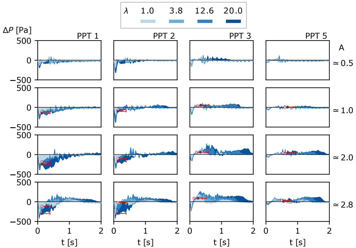
Figure 6.14. Evolution of \Delta P for the PPTs 1, 2, 3 and 5 (columns), for columns with A \approx [0.5, 1, 2, 2.8] (rows) and for all \lambda . Markers indicate \Delta P at the time when the front reaches the PPT i position for \lambda = [1, 20] and the horizontal red bar indicates a range of 0.25 s. For PPT 1 and 2, both beneath the column initial geometry, the horizontal bars indicate the time interval t = [0.125 - 0.375] .
