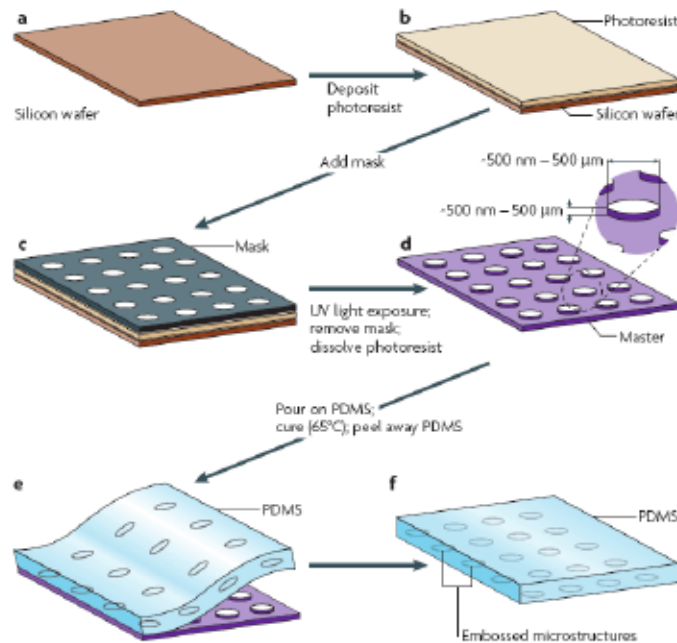
Figure 27. The process of soft lithography (Copyright: elveflow.com)
