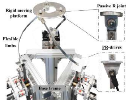
Fig. 1. A prototype of the studied parallel continuum manipulator.
