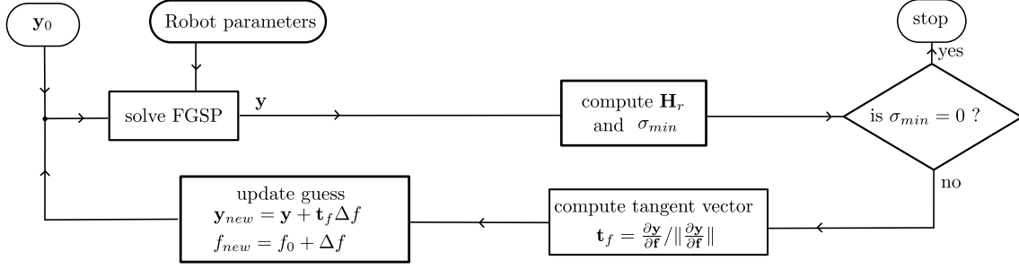
Figure 6.2: Schematics of the numerical approach for the computation of the exact critical load.
