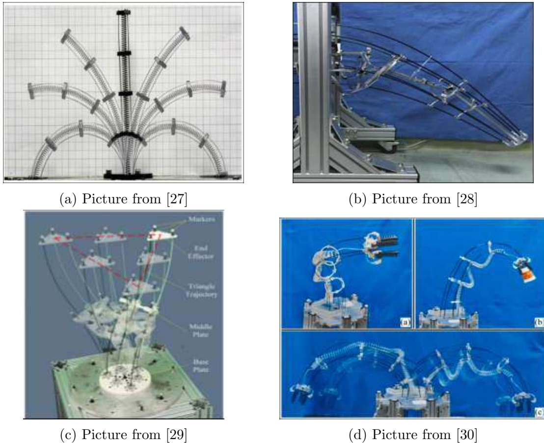
Figure 1.5: Illustration of the existing extensible CPRs . These CPRs employ intermediate disks.
