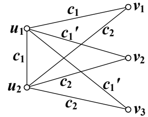
(2) G^2_k
