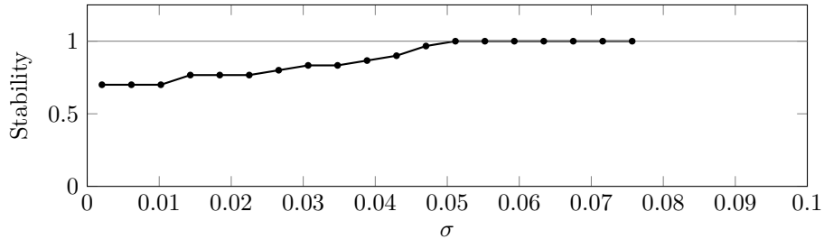
Figure 2.22 – Proportion of simulations of the fluid model reaching t = 3 out of 30 simulations, depending on the quantity \sigma of smoothing.
