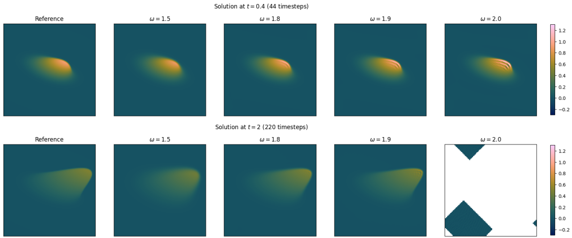
Figure 5.4.12 – (Burgers - Constant scalar relaxation) Numerical solution of the linear advection equation at t = 0.4 (top) and t = 2 (bottom) with an initial condition from the validation test cases, using different values for the constant \omega .
