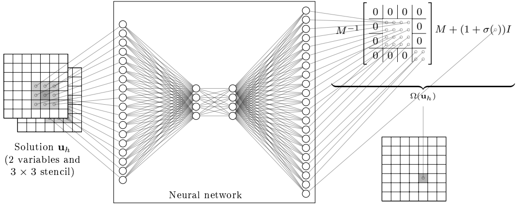
Figure 5.3.3 – Example of neural network, for a system of 2 equations solved using relaxation matrix with full matrices \Omega_v and \Omega_e .
