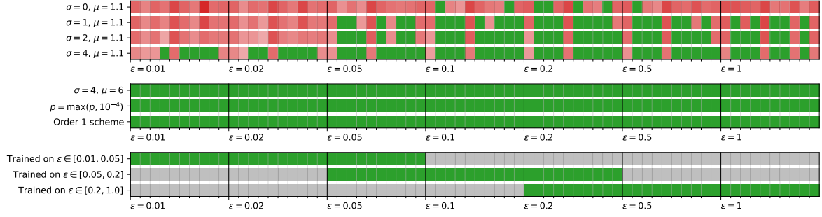
Figure 3.4.3 – Stability results for different models on 70 test cases. Green indicates stability, red instability. \sigma is the standard deviation of the gaussian kernel for smoothing the closure, \mu is the viscosity coefficient of the numerical flux, and p is the pressure.
