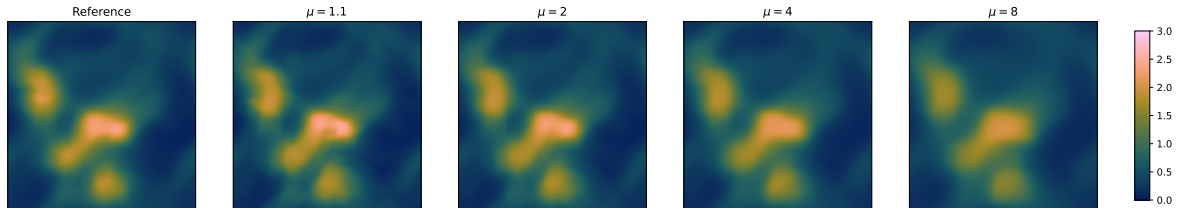
Figure 3.4.5 – Density \rho at time t = 0.2 of the solution computed with more or less viscosity \mu in the numerical flux, and smoothing with \sigma = 2 . For this illustration an initial condition that do not lead to instabilities was picked, with Knudsen number \varepsilon = 0.1 .
