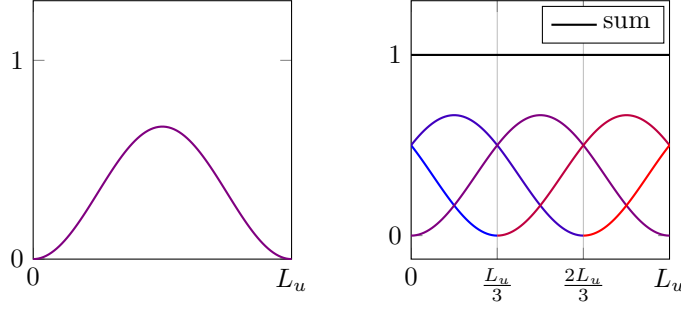
Figure 2.8 – Kernel used for the reconstruction of an entire signal from the windows predicted by the neural network, with the redundancy parameter r = 3 .
