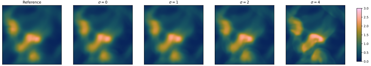
Figure 3.4.4 – Density \rho at time t = 0.2 of the solution computed with more or less smoothing applied to the closure. For this illustration an initial condition that do not lead to instabilities was picked, with Knudsen number \varepsilon = 0.1 .
