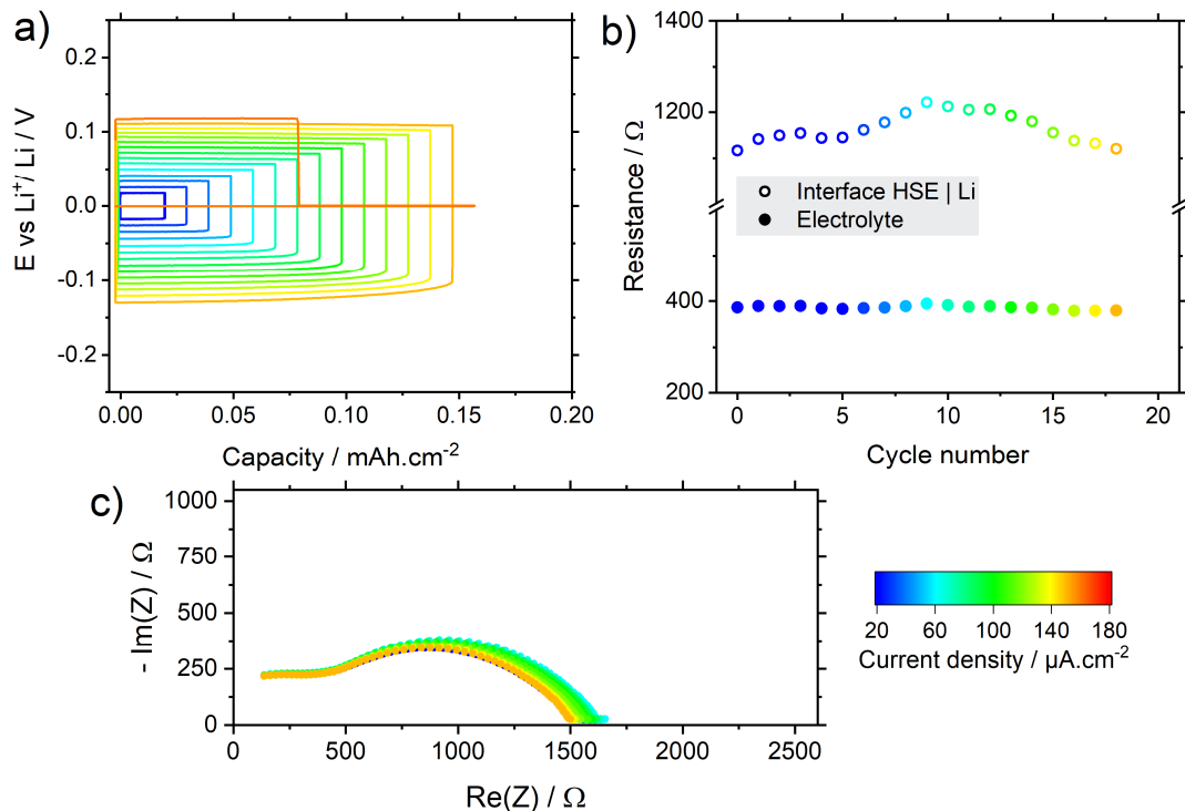
Figure S2.12 Determination of CCD of the symmetric cell with the optimised HSE based on copolymer P(EO-co-PO). (a) Voltage profile according to capacity. (b) Evolution of electrolytic and interfacial resistances over cycles. (c) EIS over cycles. Colours represent the current density applied to the symmetric cell.
