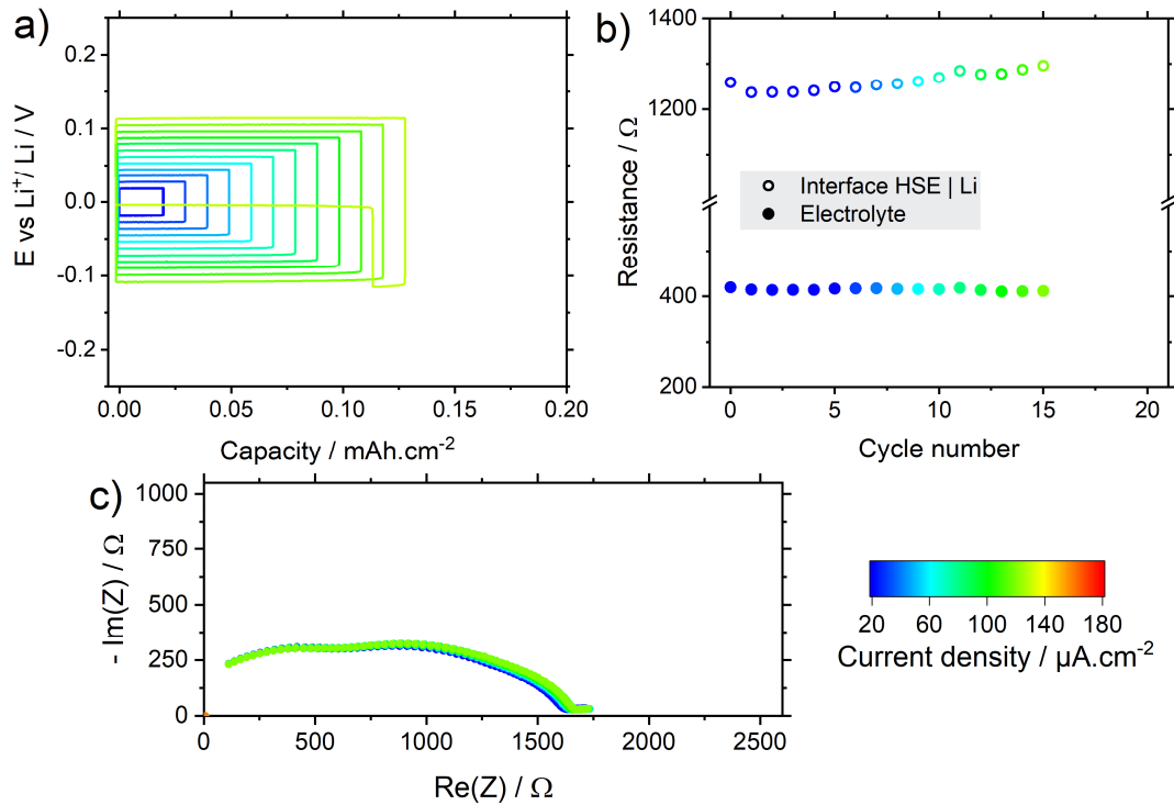
Figure S2.11 Determination of CCD of the symmetric cell with the optimised HSE based on copolymer P(EO-co-PO). (a) Voltage profile according to capacity. (b) Evolution of electrolytic and interfacial resistances over cycles. (c) EIS over cycles. Colours represent the current density applied to the symmetric cell.
