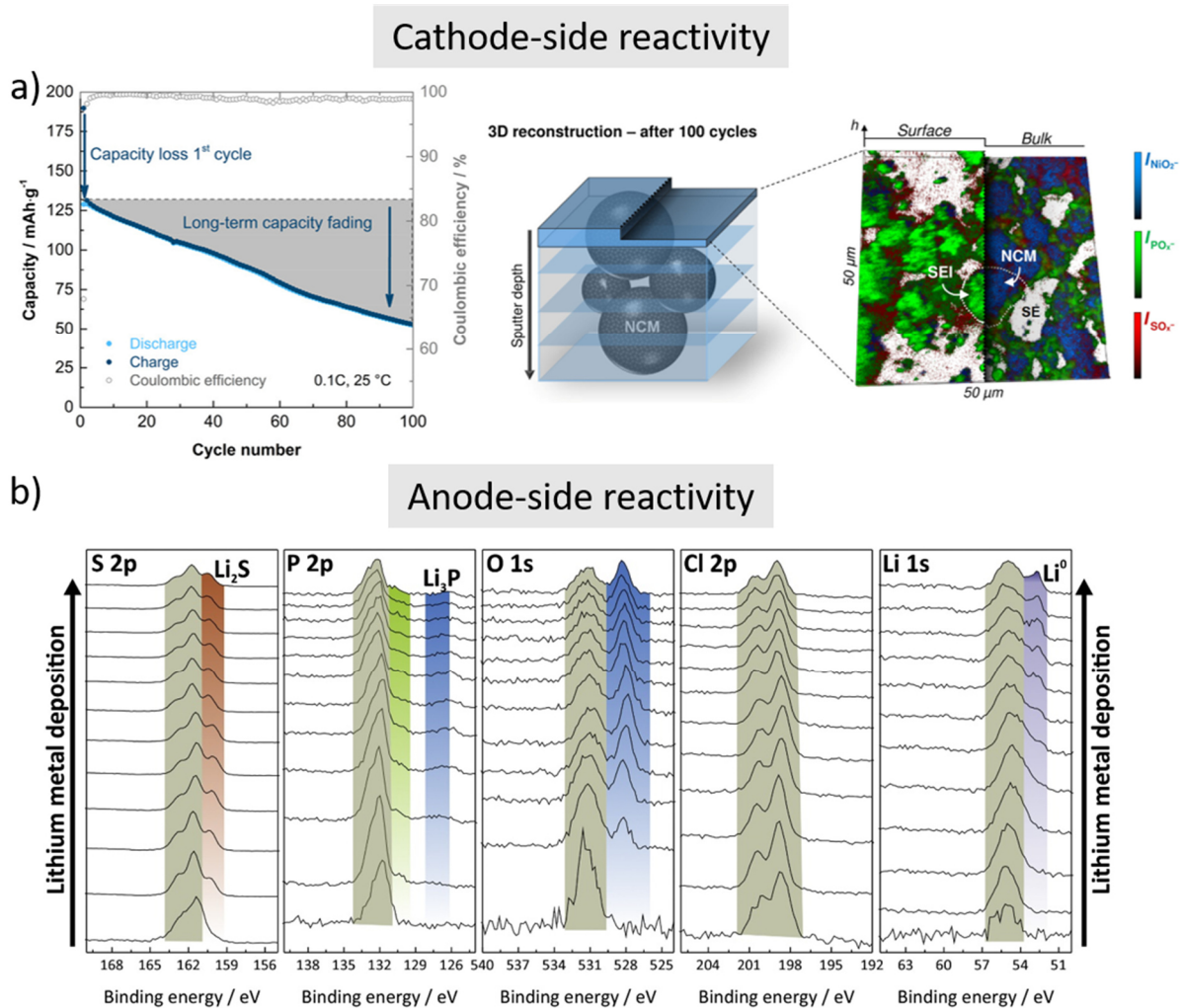
Figure 1.12 Reactivity of Li 6 PS 5 Cl at the electrodes interface. (a) Cathode side: Capacity retention of an NMC622: Li 6 PS 5 Cl | Li 6 PS 5 Cl | Li x Ni cell – Three-dimensional reconstruction of the ToF-SIMS depth profile of the cycled composite cathode. (b) In situ XPS of argyrodite during sequential lithium metal deposition, unravelling the associated degradation products. Reproduced from references. 43,99
