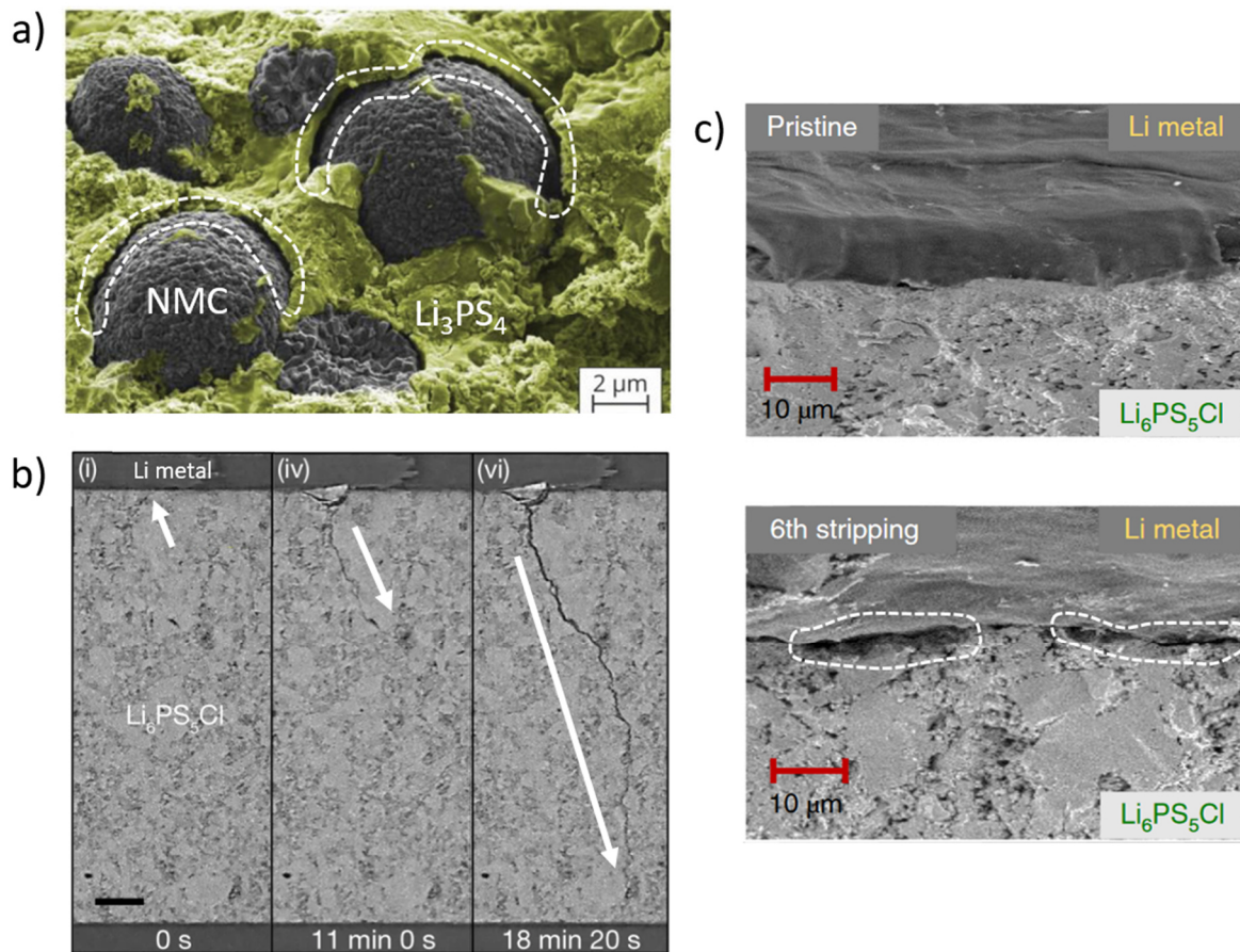
Figure 1.15 Typical mechanical issues in occurring in SSBs based on ceramic electrolyte. Dotted lines highlight the presence of voids at the electrode-SE interface. (a) Scanning electron micrographs (SEM) of cathode composite NMC811:Li 3 PS 4 in discharge state after 50 cycles. (b) Operando X-ray computed tomography (XCT) cross-sectional image slices showing the initiation of a lithium dendrite accompanied with the propagation of a crack (white arrow) in a symmetric Li | Li 6 PS 5 Cl | Li cell. (c) SEM cross-sections of the interface between lithium metal and Li 6 PS 5 Cl after 6 cycles of plating and stripping in symmetric cell configuration. Reproduced from references. 33,42,109
