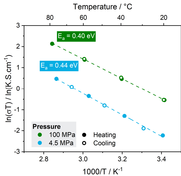
Figure S2.7 Effect of the stack pressure on pelletised Li 6 PS 5 Cl conductivity. Carbon electrodes were used to ensure best possible contact with pistons.
