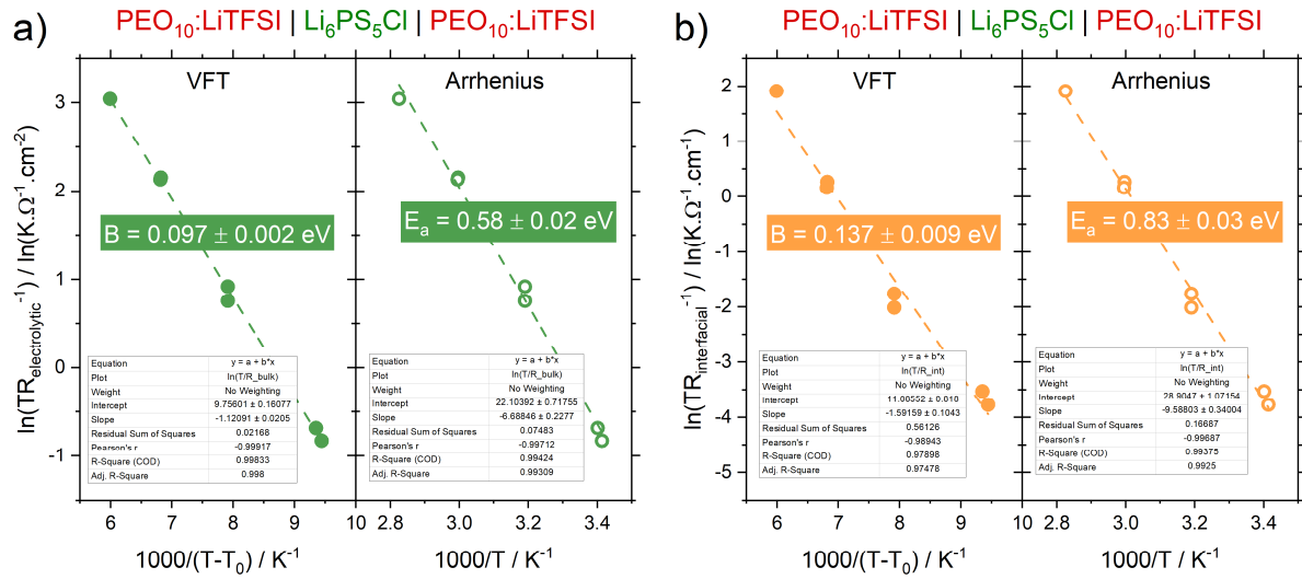
Figure S2.6 Fitting of (a) electrolytic and (b) interfacial resistances in temperature measured for the layered system PEO 10 :LiTFSI | Li 6 PS 5 Cl | PEO 10 :LiTFSI. Choice of the appropriate activation mechanism (VFT versus Arrhenius) according to highest adjusted R 2 value.
