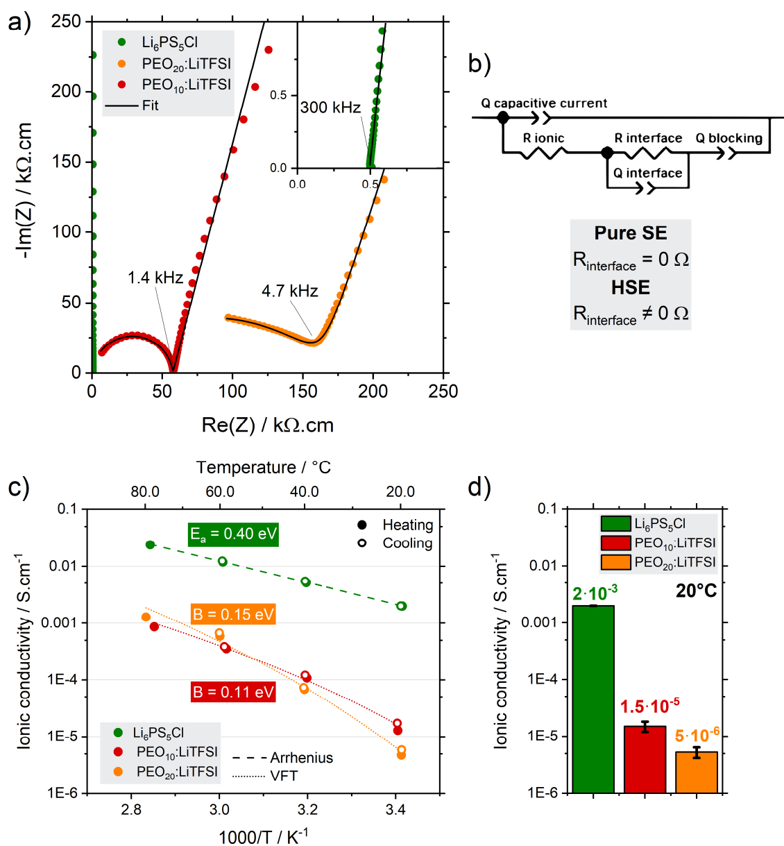
Figure 2.1 Ionic conductivity characterisation of the precursor electrolytes. (a) EIS spectra at 20^\circ\text{C} normalised by the pellet ( \text{Li}_6\text{PS}_5\text{Cl} – e = 1.2 \text{ mm} ) or the film ( \text{PEO}_x:\text{LiTFSI} – e = 50 - 100 \mu\text{m} ) form factor and their related fit. (b) Model fitting the EIS data in ion-blocking electrodes configuration. Details are available on Scheme S2.1 . (c) Temperature-dependant ionic conductivity, in the range of 20 - 80^\circ\text{C} , fitted according to the adequate activation mechanism (Arrhenius or VFT) and the associated (pseudo) activation energy E_a (or B ). (d) Ionic conductivity at 20^\circ\text{C} averaged over heating and cooling steps.
