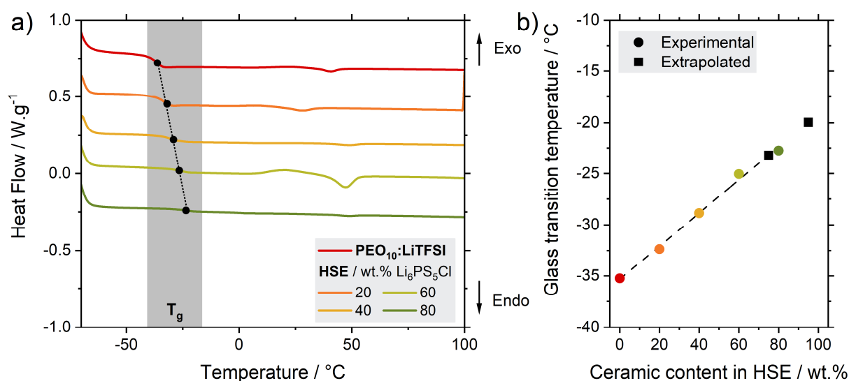
Figure 2.9 (a) Thermal analysis of the HSEs by DSC in argon atmosphere with a heat rate of 10^\circ\text{C}\cdot\text{min}^{-1} and varying content of \text{Li}_6\text{PS}_5\text{Cl} . (b) Evolution of the glass transition temperature ( T_g ) according to the ceramic content. Extrapolated values for missing points are obtained by linear fitting of the experimental data.
