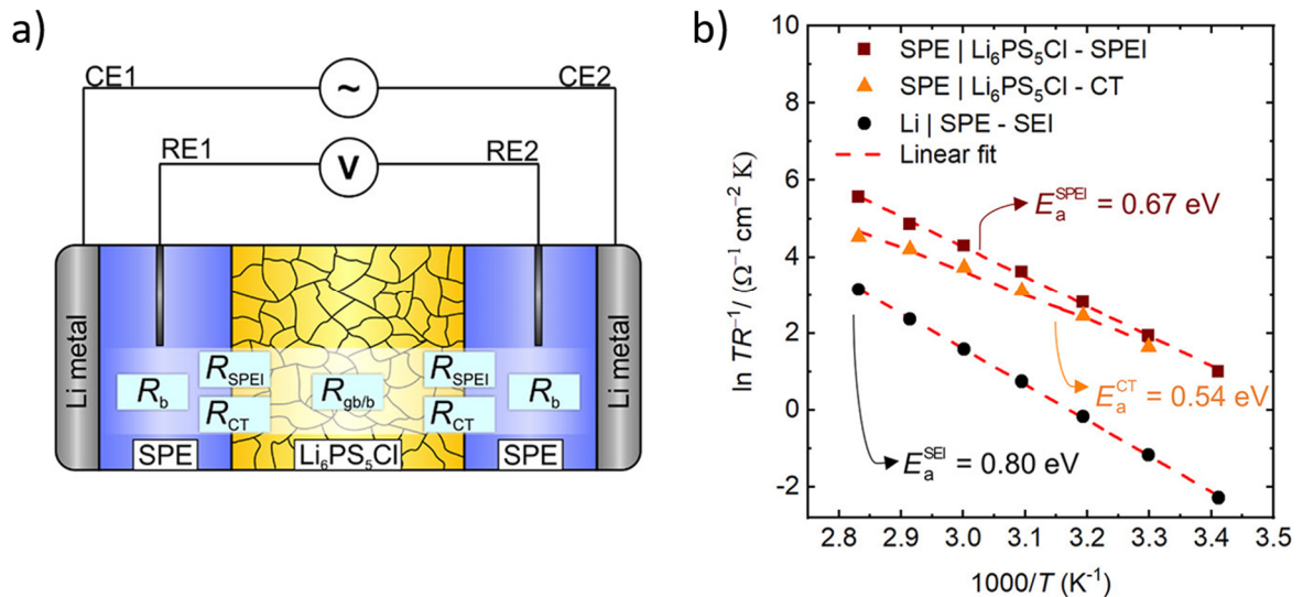
Figure 1.17 (a) Schematics of the four-point cell setup to study the PEO 10 :LiTFSI | Li 6 PS 5 Cl interface. (b) Temperature-dependent resistances of the solid-polymer electrolyte interphase (SPEI), ionic charge transfer (CT) and the Li | PEO 10 :LiTFSI solid electrolyte interphase (SEI). Reproduced from reference. 113
