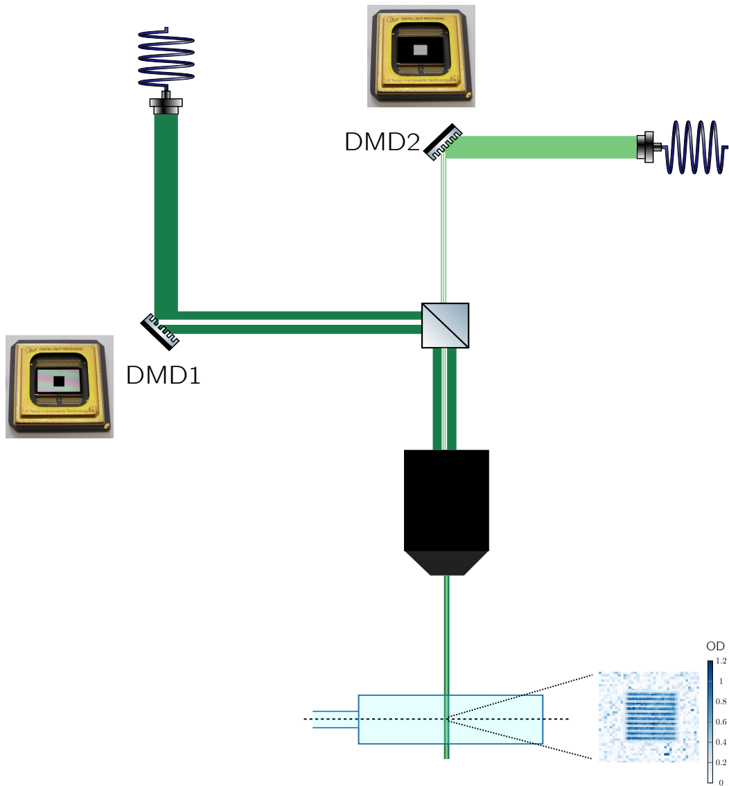
FIGURE 1.5: DMD1 and DMD2 setup. Green beams coming from two fibers are directed to both DMDs. In this example, we choose a black square box pattern for DMD1 and a sinusoidal modulation for DMD2 (zoom in to see the discretization of the mirrors). The beams are shaped according to the patterns after diffraction by the DMDs. A black mirror indicates no light is reflected to the atoms, while a white mirror indicates light is reflected to the atoms. The beams are then combined and directed towards the atoms via a microscope objective. The atomic plane, represented by the dashed line, is then imaged vertically onto a camera (Princeton Instruments, Pixis 1024 BR Excelon) using another microscope objective. An example of an absorption image obtained with these patterns is shown. The imaging setup is not depicted in the drawing. The verticality is not respected.
