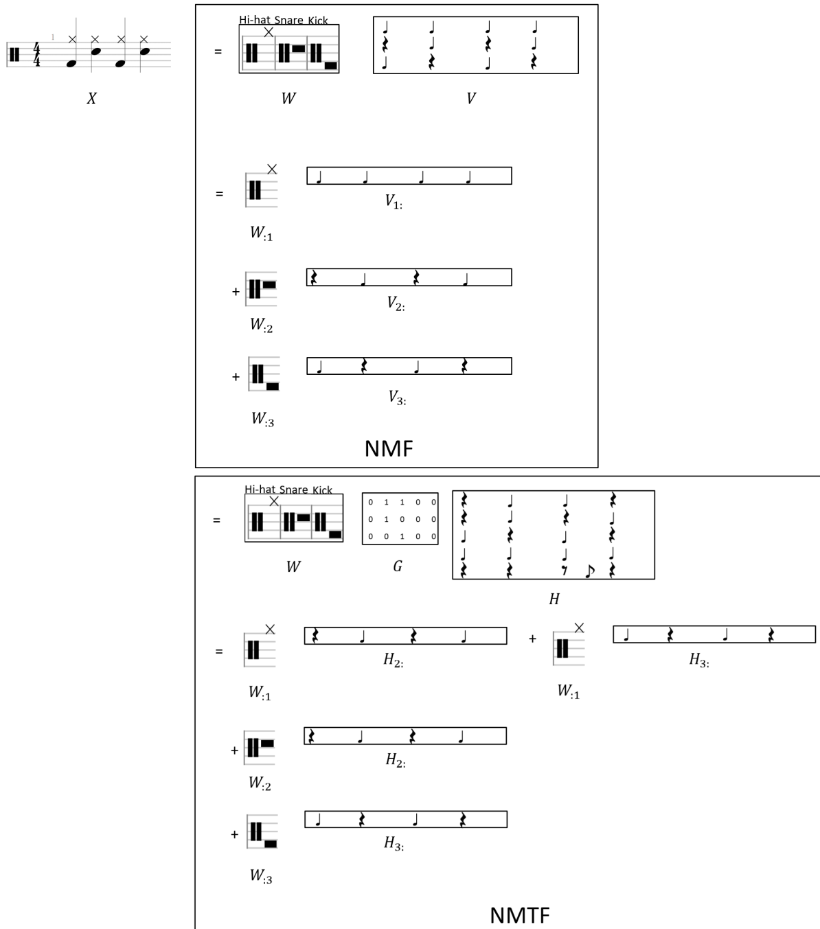
Figure 4.7 – Drum pattern from Figure 4.6, decomposed in both NMF and NMTF models. Matrix H is composed of 5 different barwise rhythmic templates, but only 2 are actually used ( H_{2:} and H_{3:} ), presenting H as a dictionary of rhythmic patterns. This is useful in the interpretation of NTD, as matrices W and H can be interpreted as dictionaries of pitch-related and duration-related information (at barscale) in the song.
