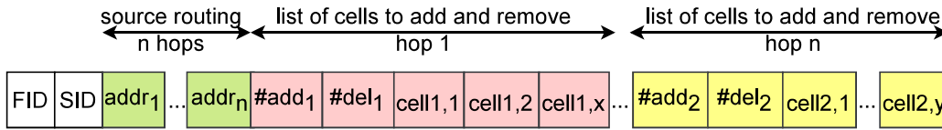
Figure 5.2: Enhanced format of config packet
