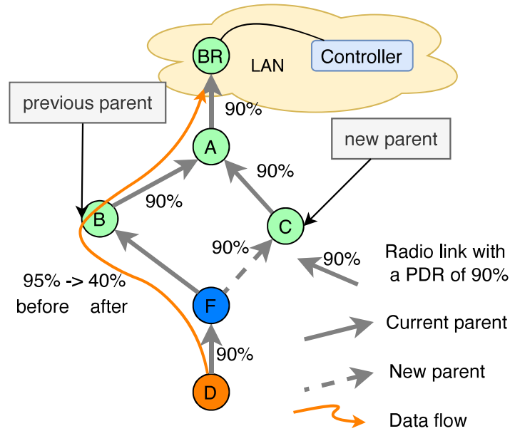
Figure 5.1: A controller needs to reconfigure the control and data planes to redirect the flows through the link ( F \rightarrow C ) when the PDR of the link ( F \rightarrow B ) decreases from 95% to 40%
