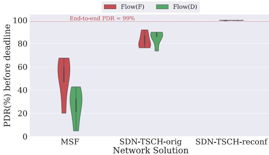
Figure 5.5: Per-flow PDR
