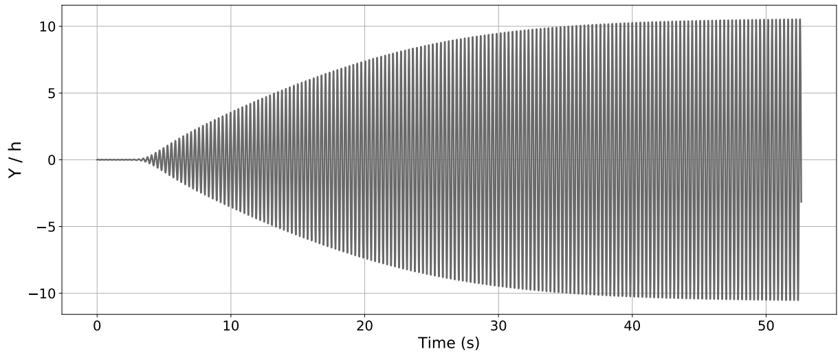
(a) Vertical displacement of the beam tip
