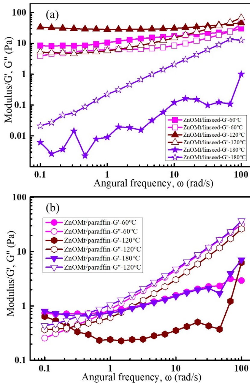
Fig. 6.15 The frequency sweep tests of the ZnOMt/linseed (a) and ZnOMt/paraffin (b) systems at different temperatures
