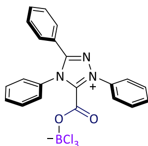
(7-BCl 3 )
