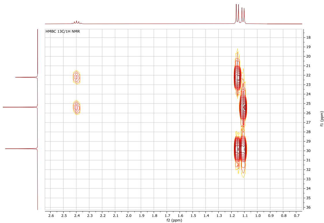
Figure S35. Zoom HMBC ^{13}\text{C}/^1\text{H} NMR spectrum of 5\text{-B}(\text{C}_6\text{F}_5)_3 in \text{CD}_2\text{Cl}_2 at 298 K.
