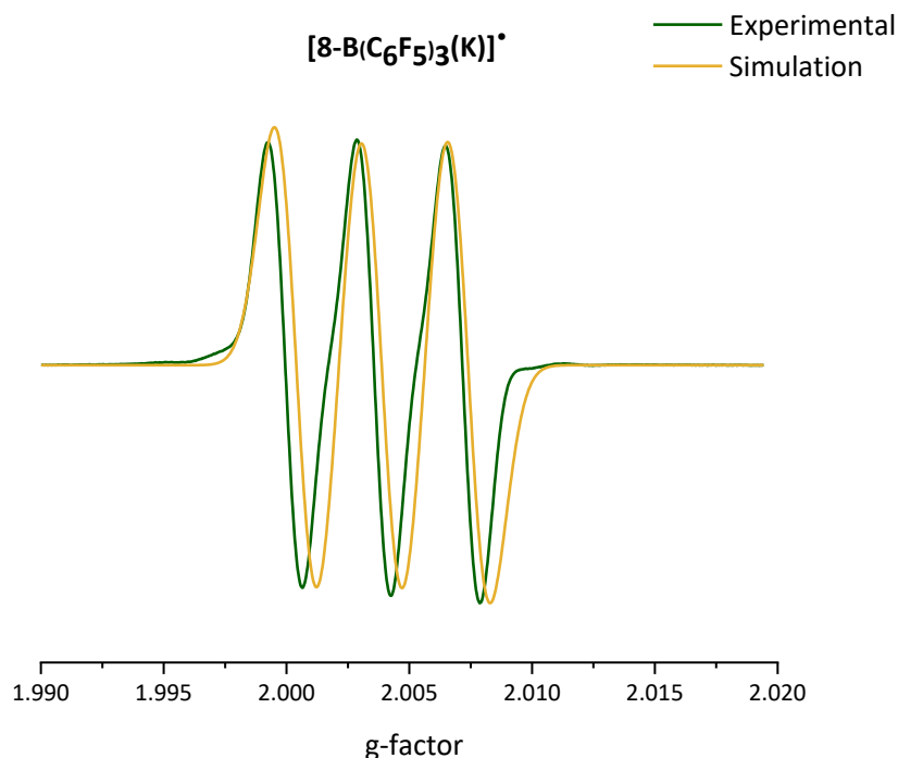
Figure 9. Experimental and calculated EPR spectra of adduct [8-B(C_6F_5)_3(K)]^\bullet in tetrahydrofuran.
