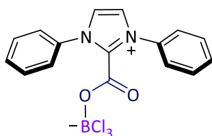
(4-BCl 3 )
