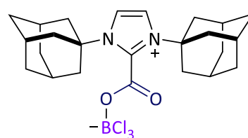
(3-BCl 3 )
