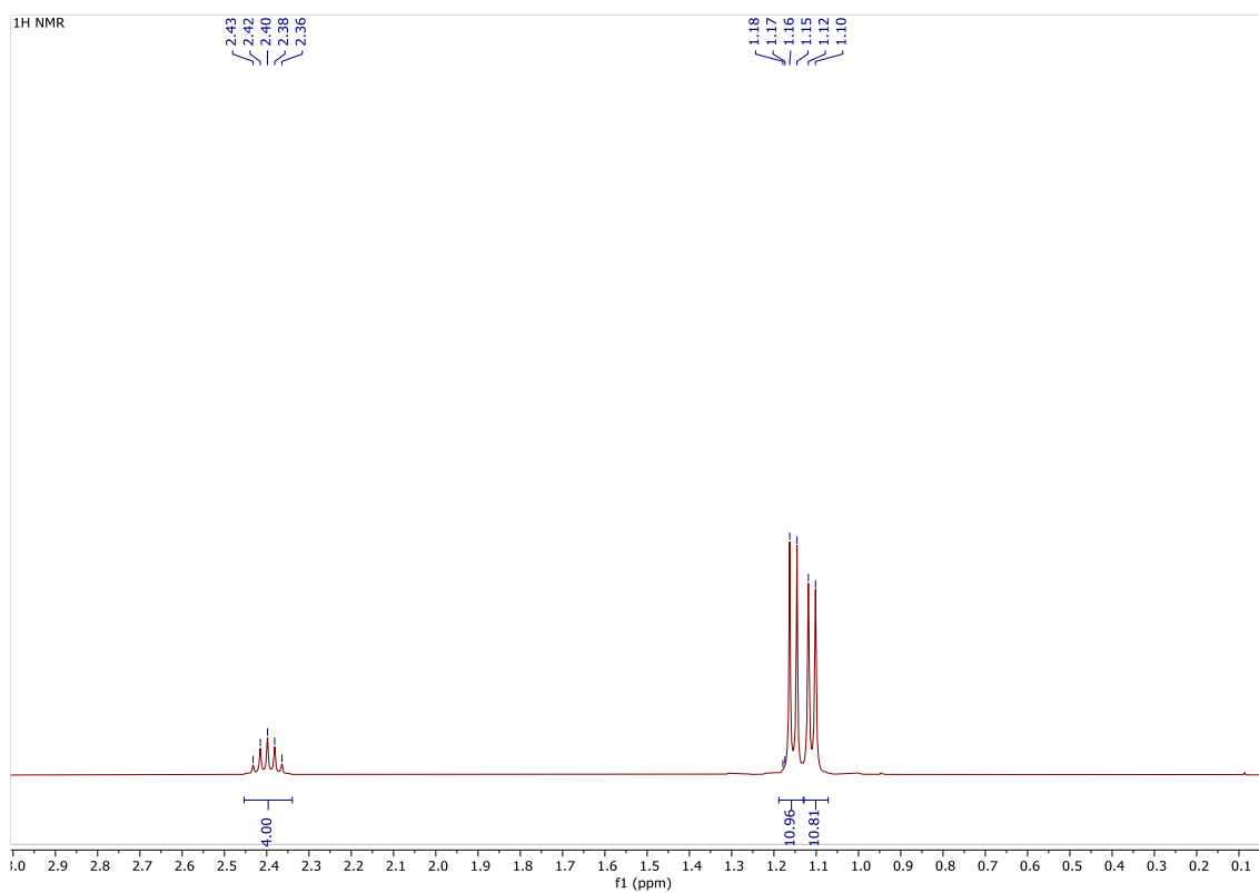
Figure S20. Zoom ^1\text{H} NMR spectrum of 5\text{-B}(\text{C}_6\text{F}_5)_3 in \text{CD}_2\text{Cl}_2 at 298 K between 2.9 and 0.1 ppm.
