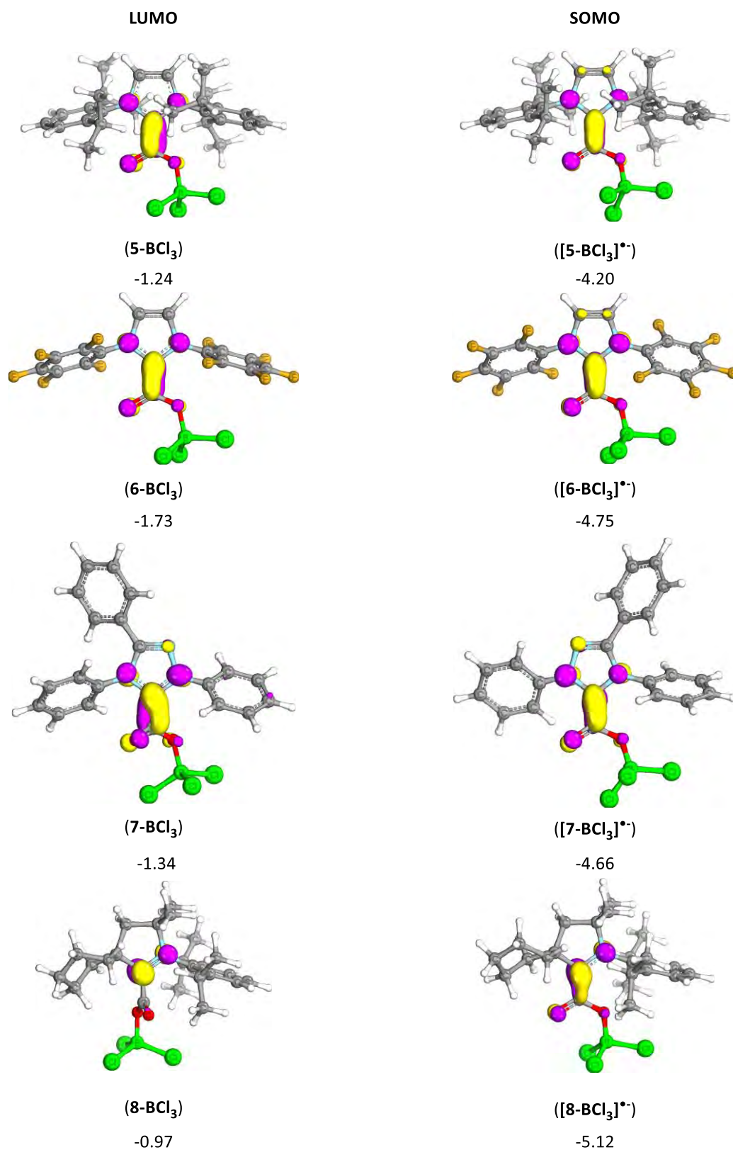
Figure 19. Localisation of the LUMO in NHC-CO 2 -BCl 3 adducts (( 5-8 )-BCl 3 ) and its energy below (left) and localisation of the SOMO in monoreduced NHC-CO 2 -BCl 3 adducts (([ 5 ] •- -[ 8 ] •- )-BCl 3 ) and its energy below (right). The energies associated to each orbital was
