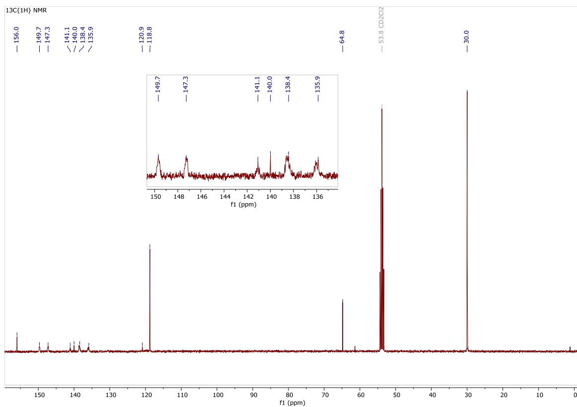
Figure 3. ^{13}\text{C}\{^1\text{H}\} NMR spectrum of 2-B(C 6 F 5 ) 3 in CD 2 Cl 2 at 298 K.
