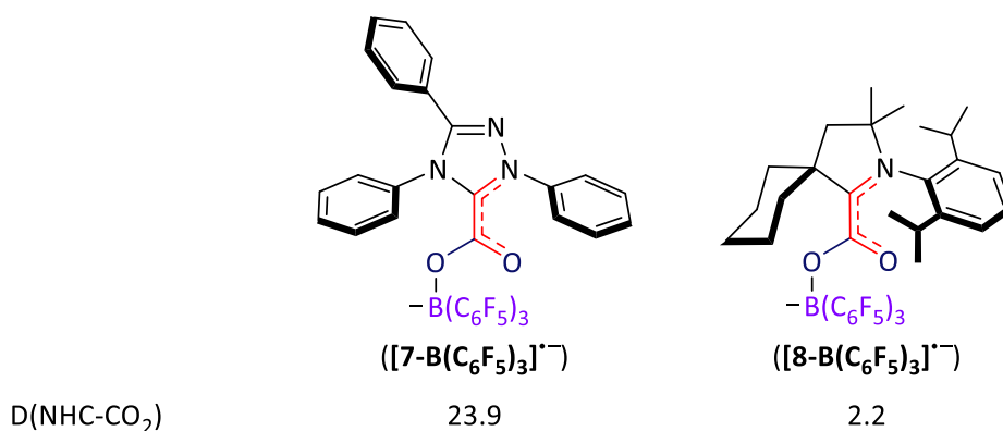
Scheme 13. Studied monoreduced NHC-CO 2 -B(C 6 F 5 ) 3 adducts ( [1-B(C_6F_5)_3]^- - [8-B(C_6F_5)_3]^- ) and the torsion angle (D(NHC-CO 2 )). The dihedral angles are expressed in degrees (°).
