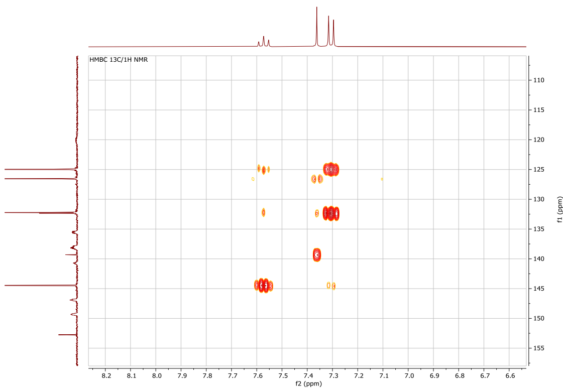
Figure S31. Zoom HMBC ^{13}\text{C}/^1\text{H} NMR spectrum of 5\text{-B}(\text{C}_6\text{F}_5)_3 in \text{CD}_2\text{Cl}_2 at 298 K.
