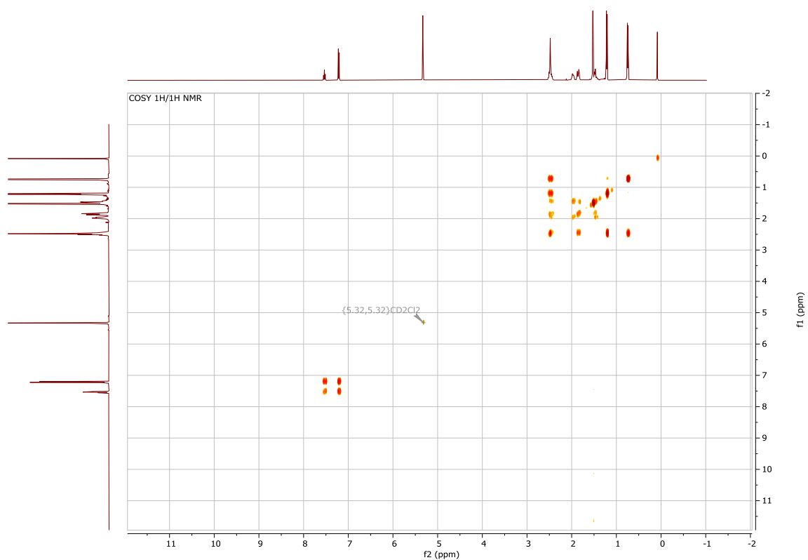
Figure S59. COSY ^1\text{H}/^1\text{H} NMR spectrum of 8-B(C 6 F 5 ) 3 in \text{CD}_2\text{Cl}_2 at 298 K.
