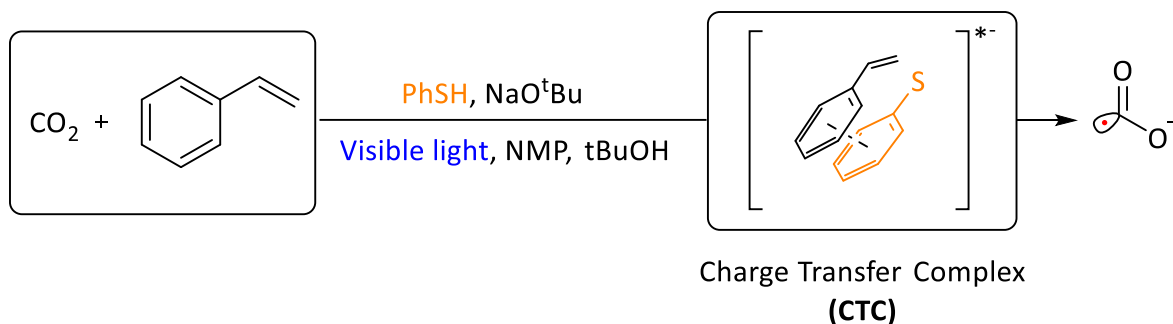
Scheme 5. Photoreduction of \text{CO}_2 using CTCs under visible light.
