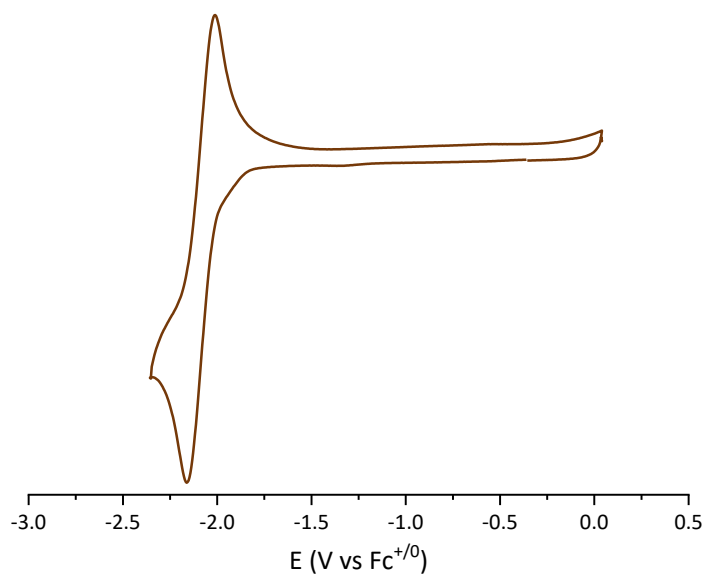
Figure S39. Normalised CV response of 5-B(C 6 F 5 ) 3 at reducing potentials under Ar atmosphere in \text{CH}_2\text{Cl}_2 . Conditions: 5 mM compound 5-B(C 6 F 5 ) 3 and 0.1 M [\text{n-Bu}_4\text{N}][\text{PF}_6] , scan 200 mV/s.
