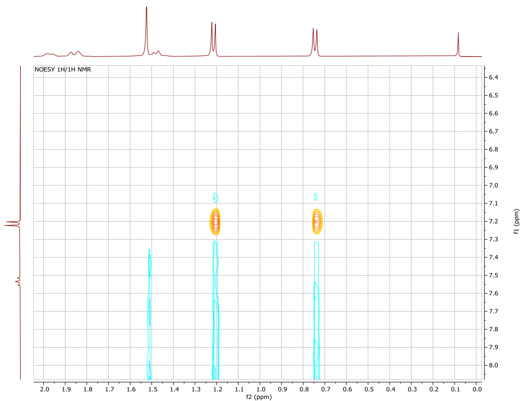
Figure S65. Zoom NOESY ^1\text{H}/^1\text{H} NMR spectrum of 8-B(C 6 F 5 ) 3 in \text{CD}_2\text{Cl}_2 at 298 K.
