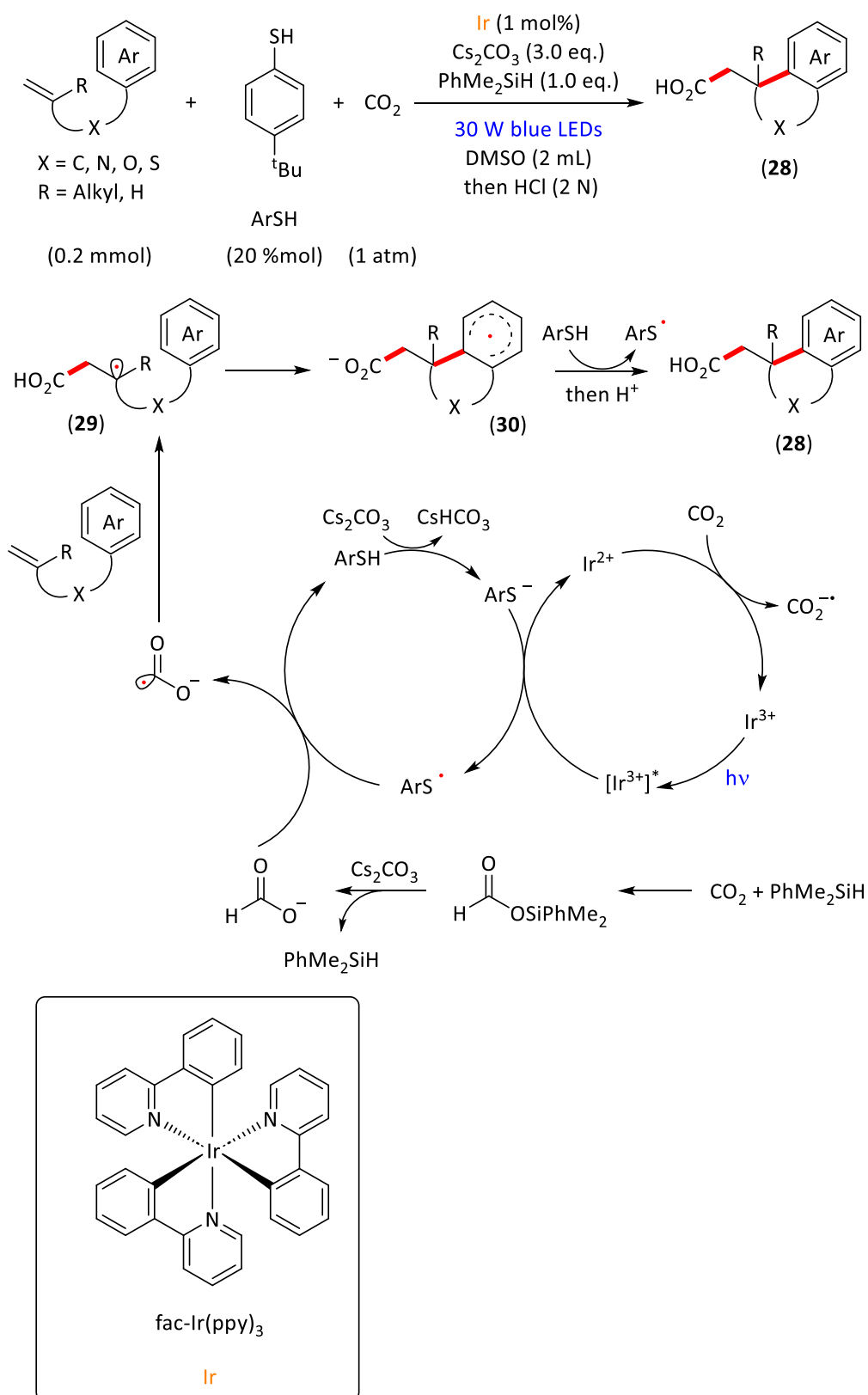
Scheme 28. Arylcarboxylation of unactivated alkenes with CO 2 using an Ir-based photocatalyst.
