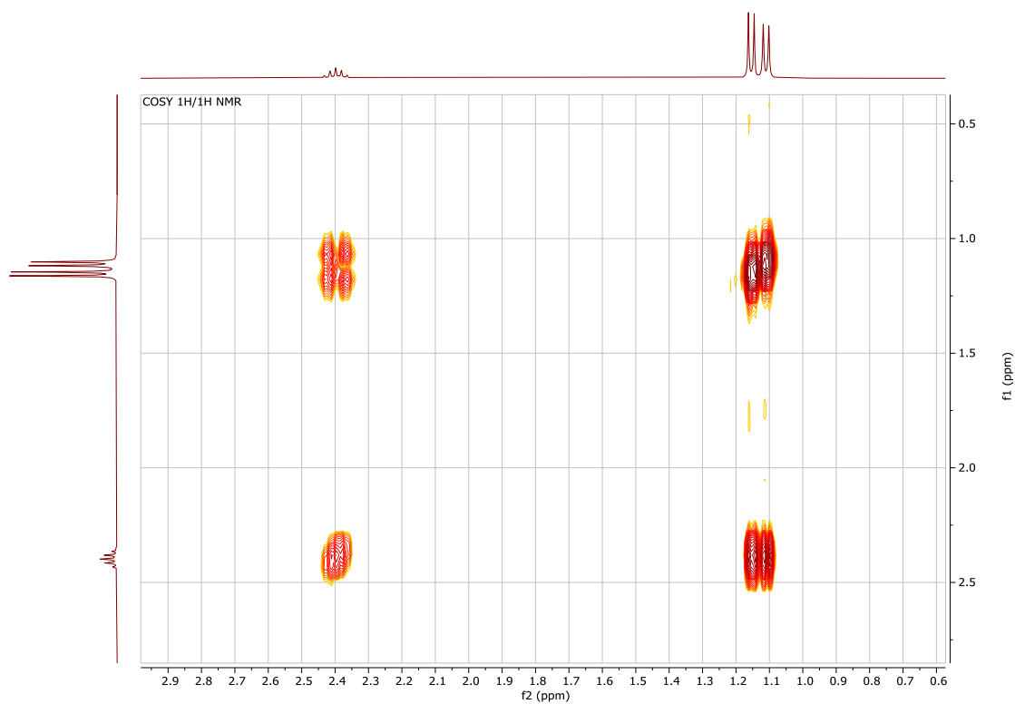
Figure S38. Zoom COSY ^1\text{H}/^1\text{H} NMR spectrum of 5-B(C 6 F 5 ) 3 in \text{CD}_2\text{Cl}_2 at 298 K.
