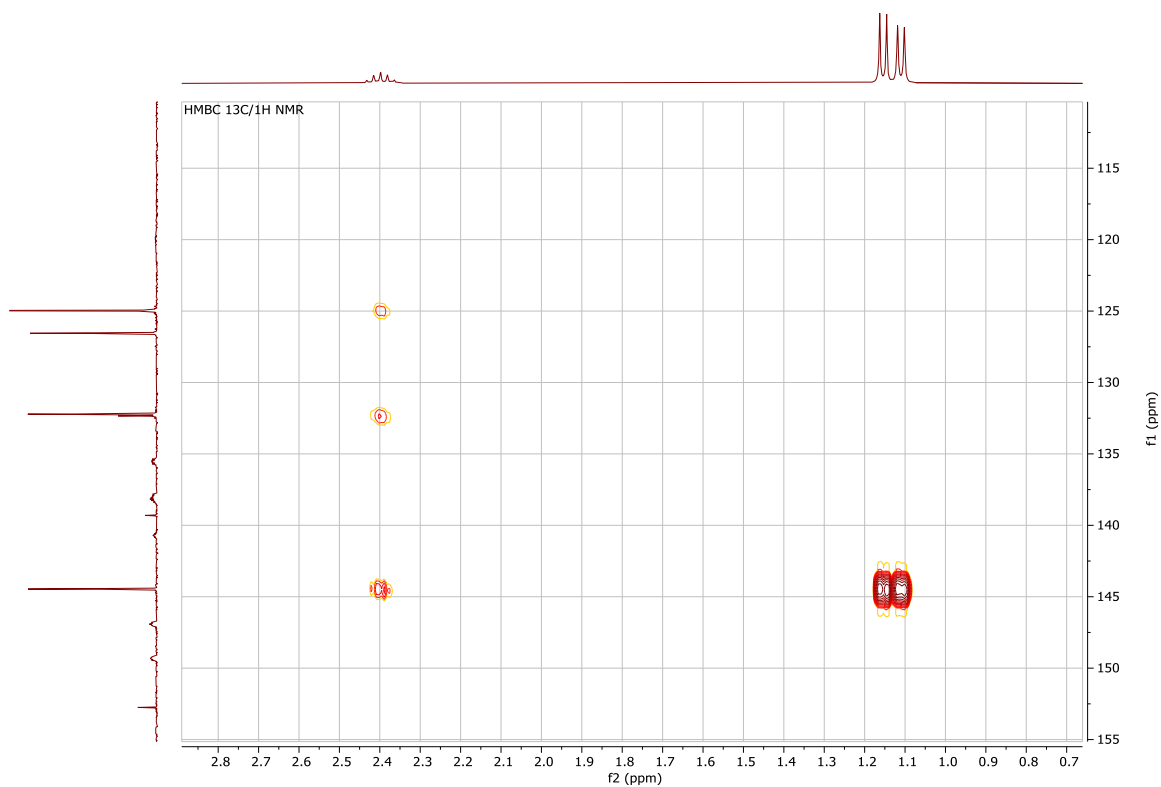
Figure S34. Zoom HMBC ^{13}\text{C}/^1\text{H} NMR spectrum of 5\text{-B}(\text{C}_6\text{F}_5)_3 in \text{CD}_2\text{Cl}_2 at 298 K.
