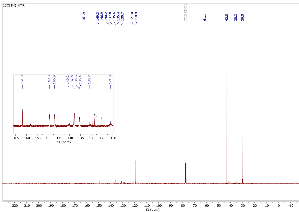
Figure S9. 13 C{ 1 H} NMR spectrum of 3-B(C 6 F 5 ) 3 in CDCl 3 at 298 K. (* C 6 H 5 CH 3 ) 40 mg of 3-B(C 6 F 5 ) 3 , ns = 8249.
