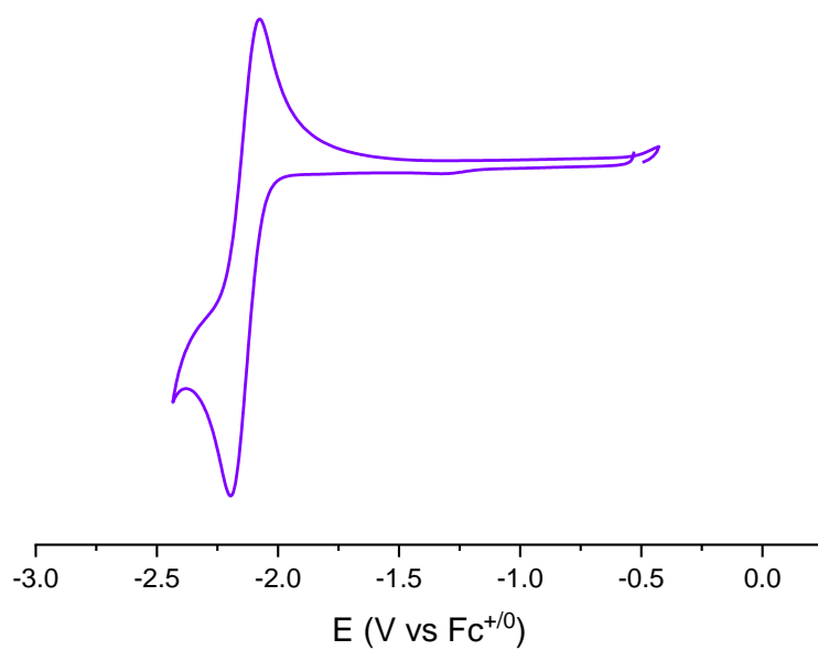
Figure S20. Normalised CV response of 8 at reducing potentials under Ar atmosphere in dichloromethane. Conditions: 5 mM compound 8 and 0.1 M [n\text{-Bu}_4\text{N}][\text{PF}_6] , scan 200 mV/s.
