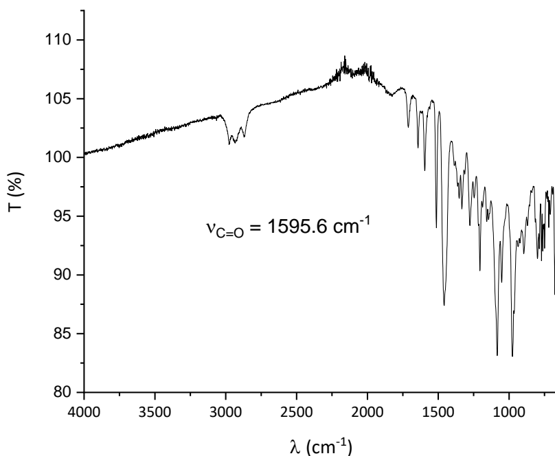
Figure S69. FTIR (solid state) of [8-B(C_6F_5)_3(K)]^* at 298 K.
