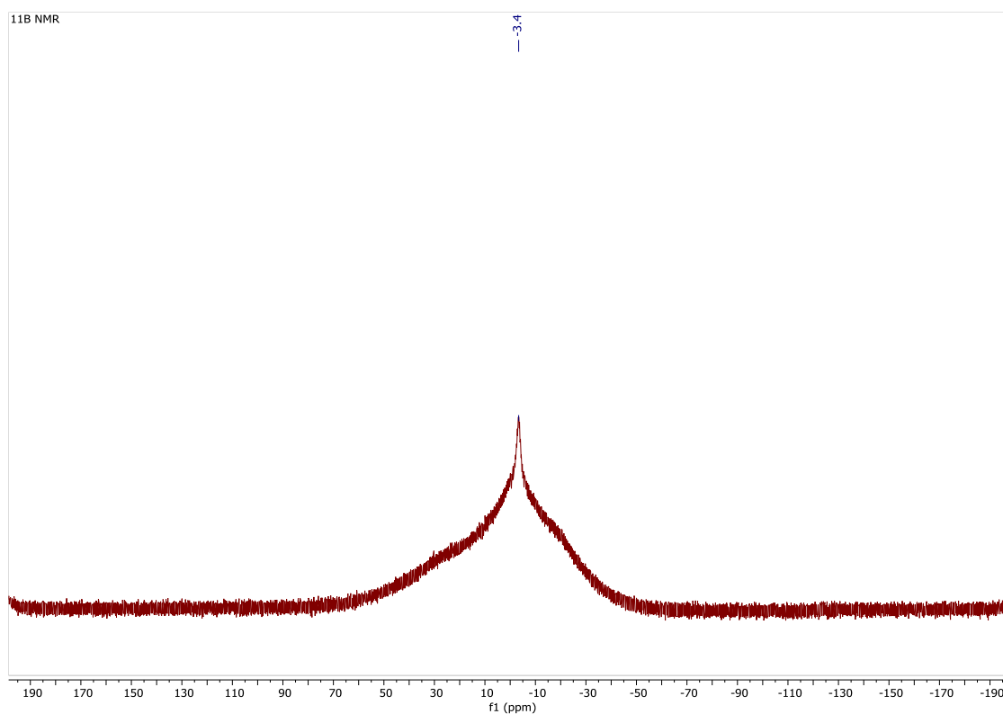
Figure S21. ^{11}\text{B} NMR spectrum of 5\text{-B}(\text{C}_6\text{F}_5)_3 in \text{CD}_2\text{Cl}_2 at 298 K.
