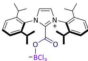
(5-BCl 3 )
