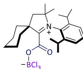
(8-BCl 3 )
