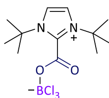
(2-BCl 3 )
