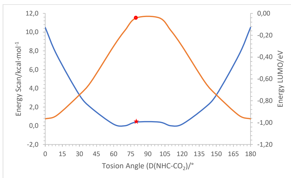
Figure 22. Conformation analysis of adduct 2-B(C 6 F 5 ) 3 and its LUMO energy as function of the torsion angle between the NHC and the CO 2 moiety (D(NHC-CO 2 )). The blue line corresponds to the evolution of the energy associated with each conformer respect to D(NHC-CO 2 ) and the orange one is related to the evolution of the energy of the LUMO with the torsion angle. The red circle and star correspond to the absolute minimum conformer.
