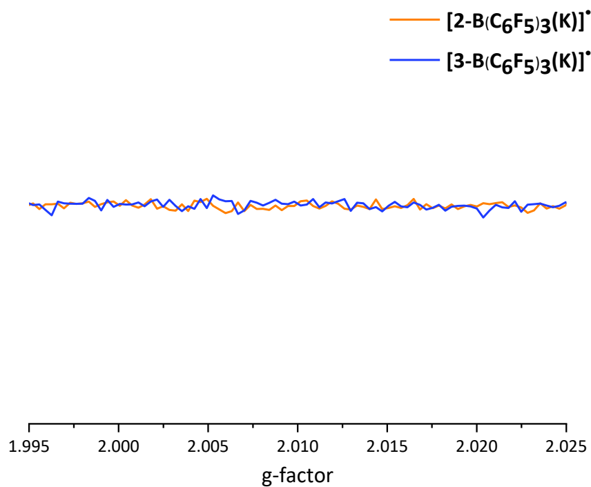
Figure 6. Continuous wave X-band EPR spectra of [2-B(C_6F_5)_3(K)]^\bullet and [3-B(C_6F_5)_3(K)]^\bullet taken on a 3.7 mM THF solution at rt.
