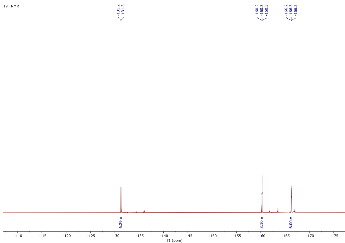
Figure S4. ^{19}\text{F} NMR spectrum of 2-B(C 6 F 5 ) 3 in CD 2 Cl 2 at 298 K.
