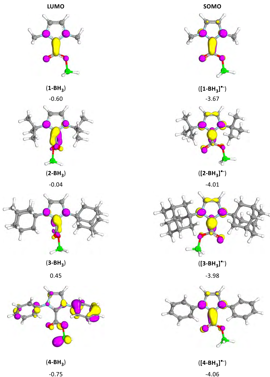
Figure 16. Localisation of the LUMO in NHC-CO 2 -BH 3 adducts ((1-4)-BH 3 ) and its energy below (left) and localisation of the SOMO in monoreduced NHC-CO 2 adducts (([5] - -[8] - )-BH 3 ) and its energy below (right). The energies associated to each orbital was expressed in electron-volts (eV). The isosurface threshold value is 45% and the resolution, 12/Å.
