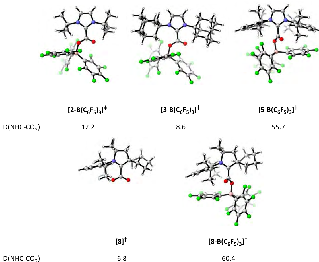
Figure 28. Transition state of each adduct ( [8] ‡ , [2-B(C 6 F 5 ) 3 ] ‡ , [3-B(C 6 F 5 ) 3 ] ‡ , [5-B(C 6 F 5 ) 3 ] ‡ and [8-B(C 6 F 5 ) 3 ] ‡ ) along with the torsion angle ( D(\text{NHC-CO}_2) ) expressed in degrees (°).
