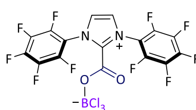
(6-BCl 3 )
