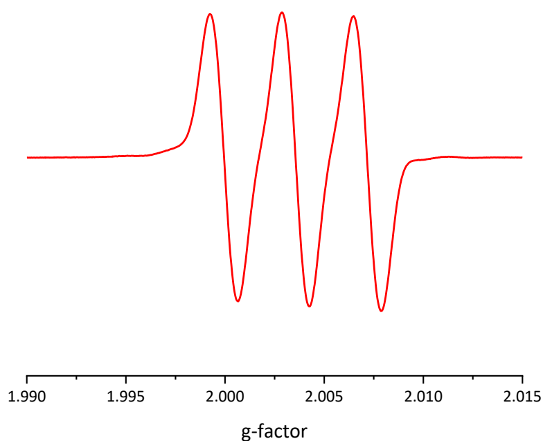
Figure S71. Continuous wave X-band EPR spectrum taken on a 2 mM [\text{8-B}(\text{C}_6\text{F}_5)_3(\text{Co})]^* dichloromethane solution at room temperature.
