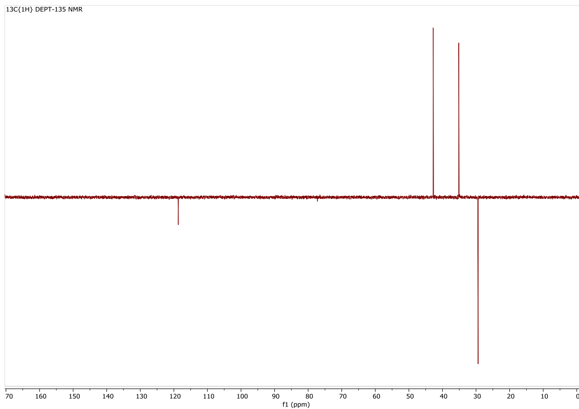
Figure S10. 13 C{ 1 H} DEPT-135 NMR spectrum of 3-B(C 6 F 5 ) 3 in CDCl 3 at 298 K.
