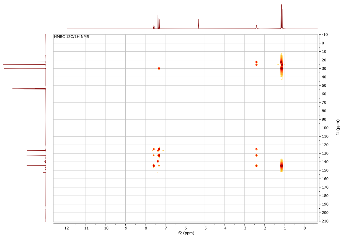
Figure S30. HMBC ^{13}\text{C}/^1\text{H} NMR spectrum of 5\text{-B}(\text{C}_6\text{F}_5)_3 in \text{CD}_2\text{Cl}_2 at 298 K.
