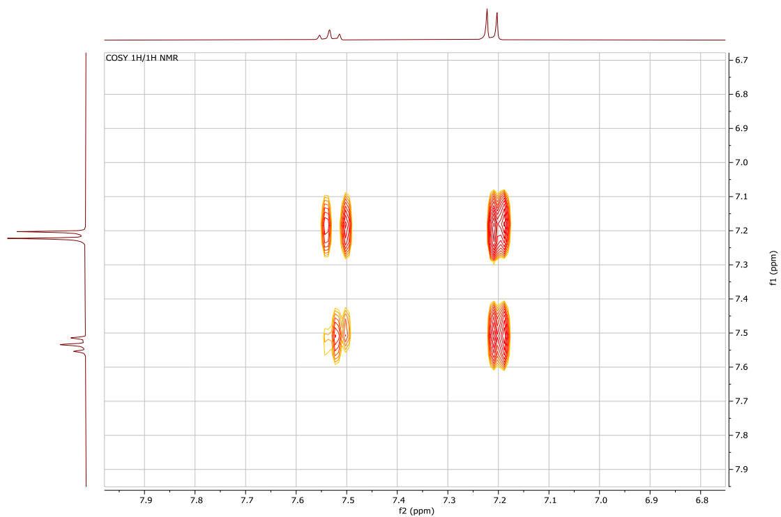
Figure S60. Zoom COSY ^1\text{H}/^1\text{H} NMR spectrum of 8-B(C 6 F 5 ) 3 in \text{CD}_2\text{Cl}_2 at 298 K.
