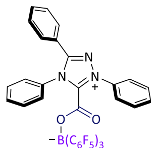
(7-B(C 6 F 5 ) 3 )
