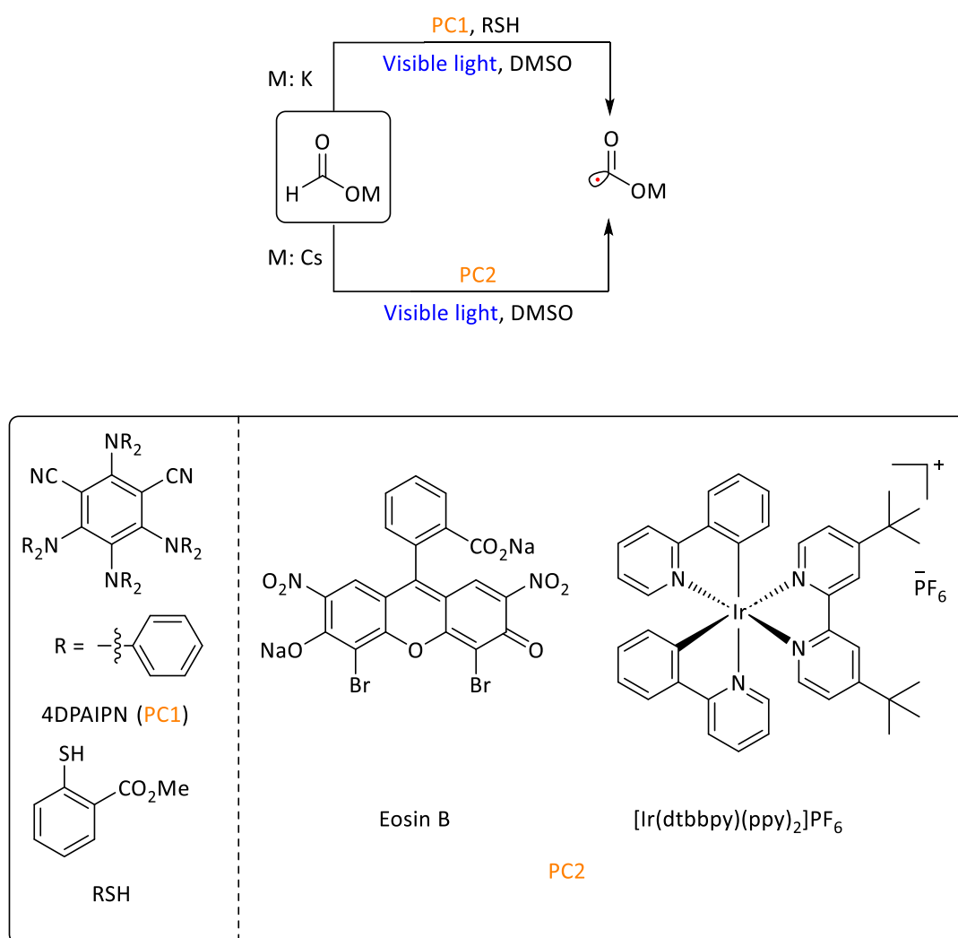
Scheme 10. Generation of \text{CO}_2 radical anion from formate.
