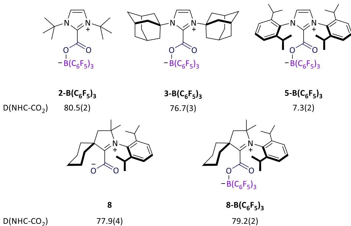
Scheme 14. Synthesised NHC-CO 2 -based adducts along with their torsion angles (D(NHC-CO 2 )) from the XRD analysis. The angles were expressed in degrees.
