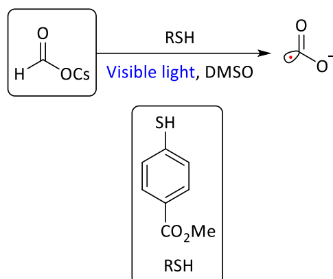
Scheme 11. Formation of \text{CO}_2 radical anion using only thiol derivatives under visible light.
