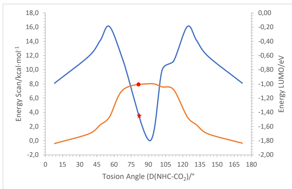
Figure 26. Conformation analysis of adduct 8-B(C 6 F 5 ) 3 and its LUMO energy as function of the torsion angle between the NHC and the CO 2 moiety ( D(\text{NHC-CO}_2) ). The blue line corresponds to the evolution of the energy associated with each conformer respect to D(\text{NHC-CO}_2) and the orange one is related to the evolution of the energy of the LUMO with the torsion angle. The red circle and star correspond to the absolute minimum conformer.
