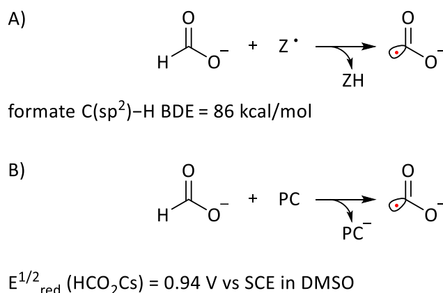
Scheme 9. A) Hydrogen Atom Transfer (HAT). B) Single Electron Transfer (SET) for a formate salt.
