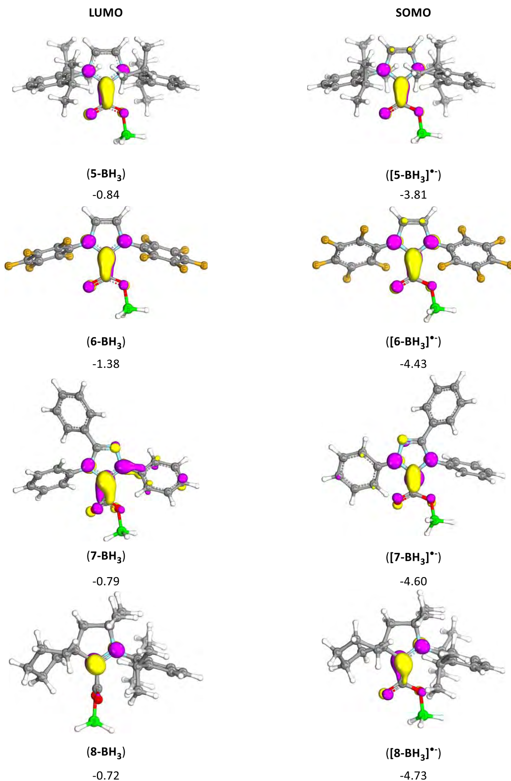
Figure 17. Localisation of the LUMO in NHC-CO 2 -BH 3 adducts (( 5-8 )-BH 3 ) and its energy below (left) and localisation of the SOMO in monoreduced NHC-CO 2 -BH 3 adducts (([ 5 ] •- - [8] •- )-BH 3 ) and its energy below (right). The energies associated to each orbital was
