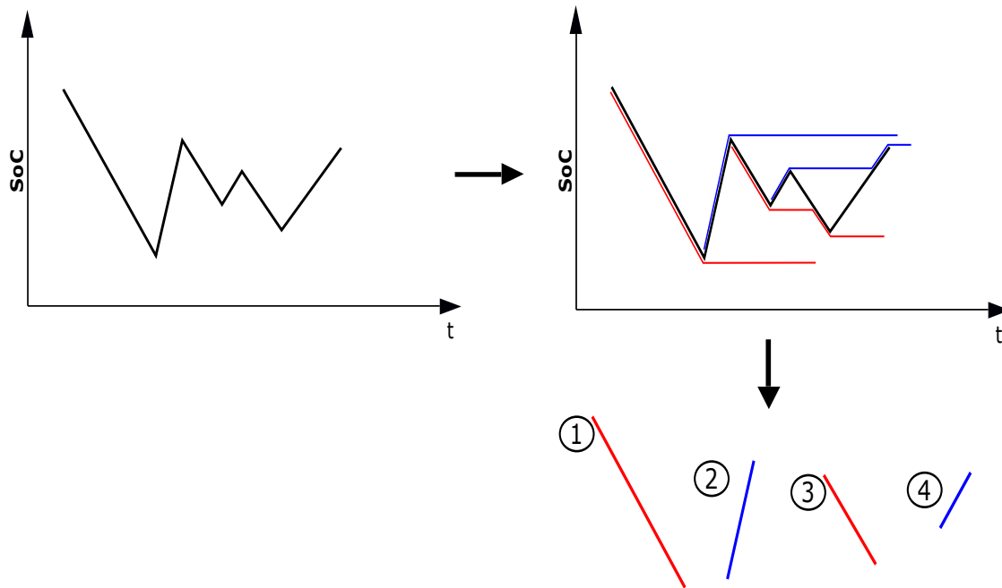
Figure 6.1: Rainflow-Counting applied to a simple SoC(t) .
