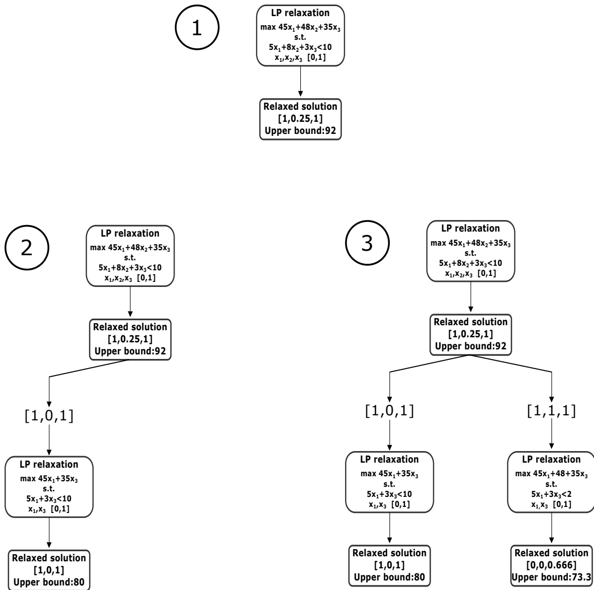
Figure 3.6: BB method for a simple ILP. At step 1, the original problem is relaxed and transformed into a LP. It is then solved, obtaining an upper-bound of 92 for the original problem. The LP solution is not made from integers, therefore, it is rounded creating two branches. In step 2 the first branch is analyzed. Once again, constraints are relaxed and the corresponding LP is solved. This time, the solution corresponds to integers and therefore, the best possible solution on this branch is found. In the third step, the second branch is analyzed. After solving the corresponding LP, it can be seen that the new upper-bound is inferior to the previously found solution and, therefore, this branch is pruned and the algorithm ends
