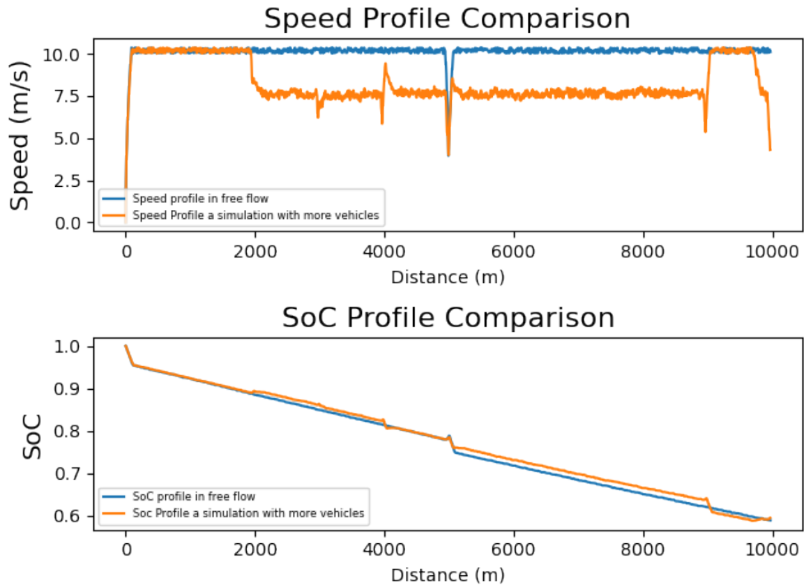
Figure 5.18: Comparison between simulations in free flow and with other vehicles
