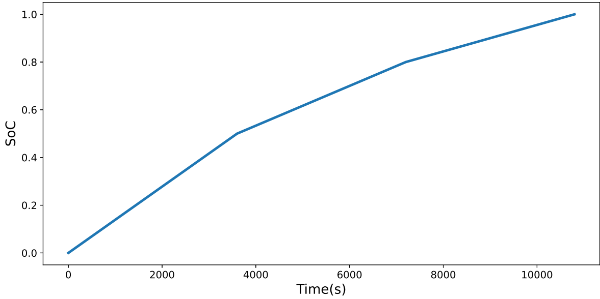
Figure 5.14: Non-linear charging process approximated by a piece-wise linear function.
