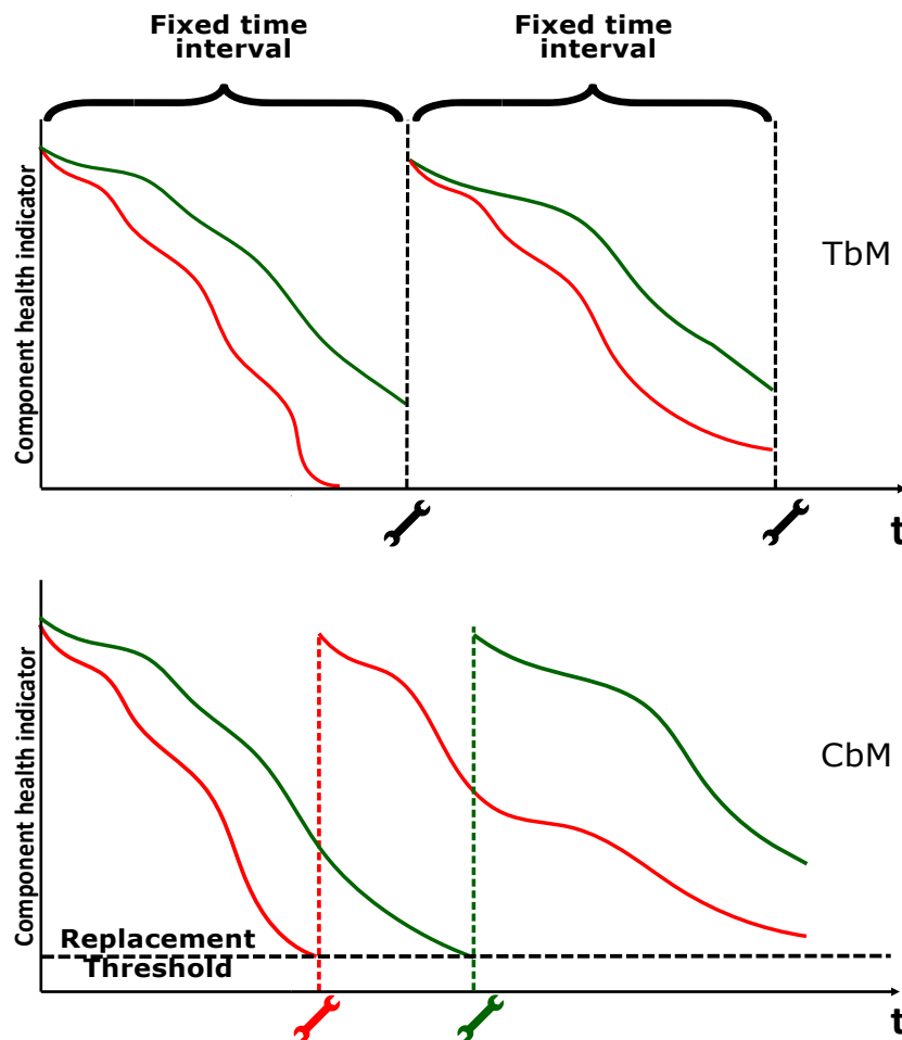
Figure 2.2: Illustration of the difference between the simplest forms of TbM and CbM. Dashed lines represent maintenance operations that restore each component to a as good as new state. Notice that in CbM each component has a different maintenance date while in TbM both are maintained at the same moment. As a consequence, Component 1 - health state represented by the red line - is change too late in the first maintenance interval while component 2 - health state represented by the green line - is replaced too early in the second intervention.
