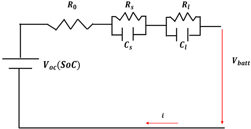
Figure 5.13: Second-order ECM for a battery.
