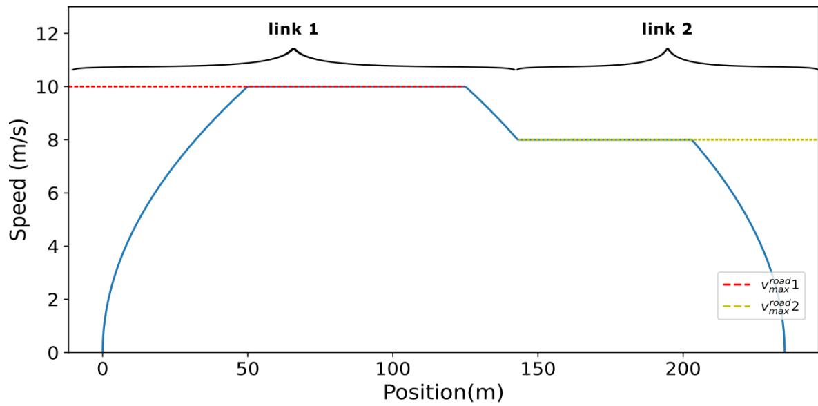
Figure 5.10: Speed with vehicle travelling through two consecutive road links.
