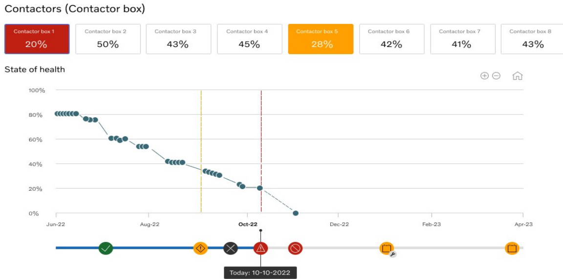
Figure 1.9: Health indicator visualization for a contactor. The graph shows data points collected from the vehicle until the present date. The dashed line seen after October is the predicted trajectory of this indicator, showing when this component is expected to reach a critical state
