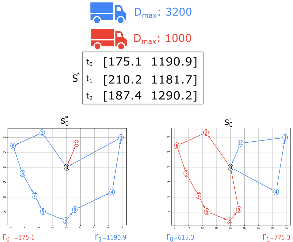
Figure 4.9: Illustration of promising route configuration search. In this instance, assigning the longest routes for the blue vehicle violates its safety constraints, therefore, configurations such as s' must be considered.
