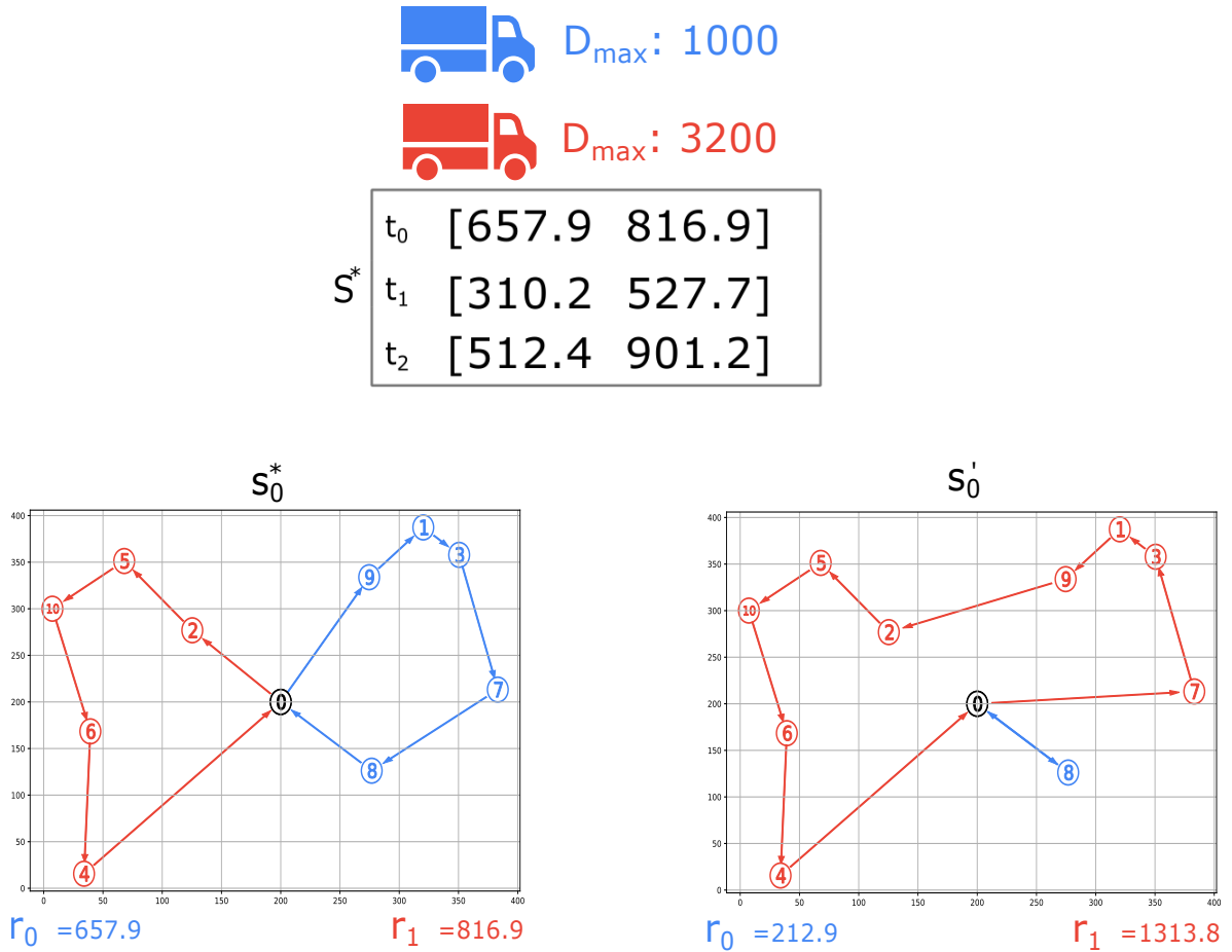
Figure 4.8: Illustration of promising route configuration search. In this instance, assigning the shortest routes for the red vehicle would violate its safety constraints, therefore, configurations such as s' must be considered.
