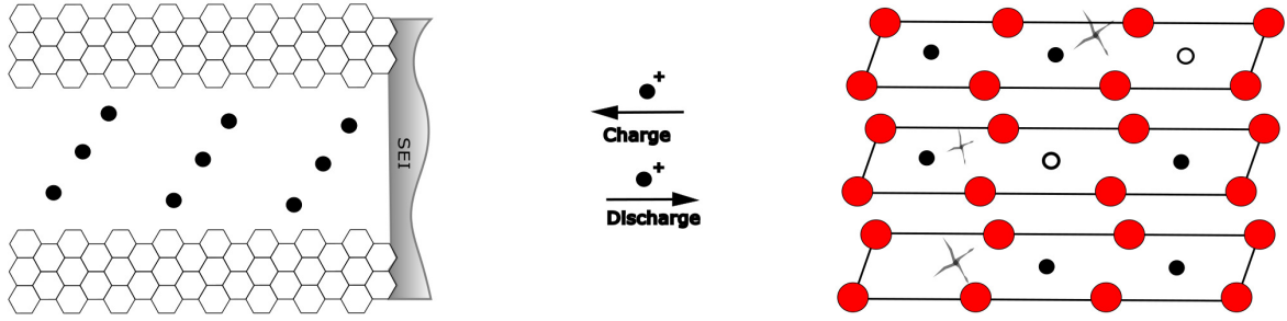
Figure 5.3: Illustration of degradation mechanisms in a Lithium-ion battery cell.
