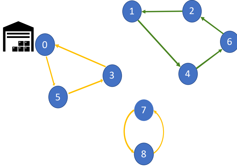
Figure 3.5: Example of solutions obtained when not including sub-tour constraints such as Constraint 3.12 in the VRP optimization model.
