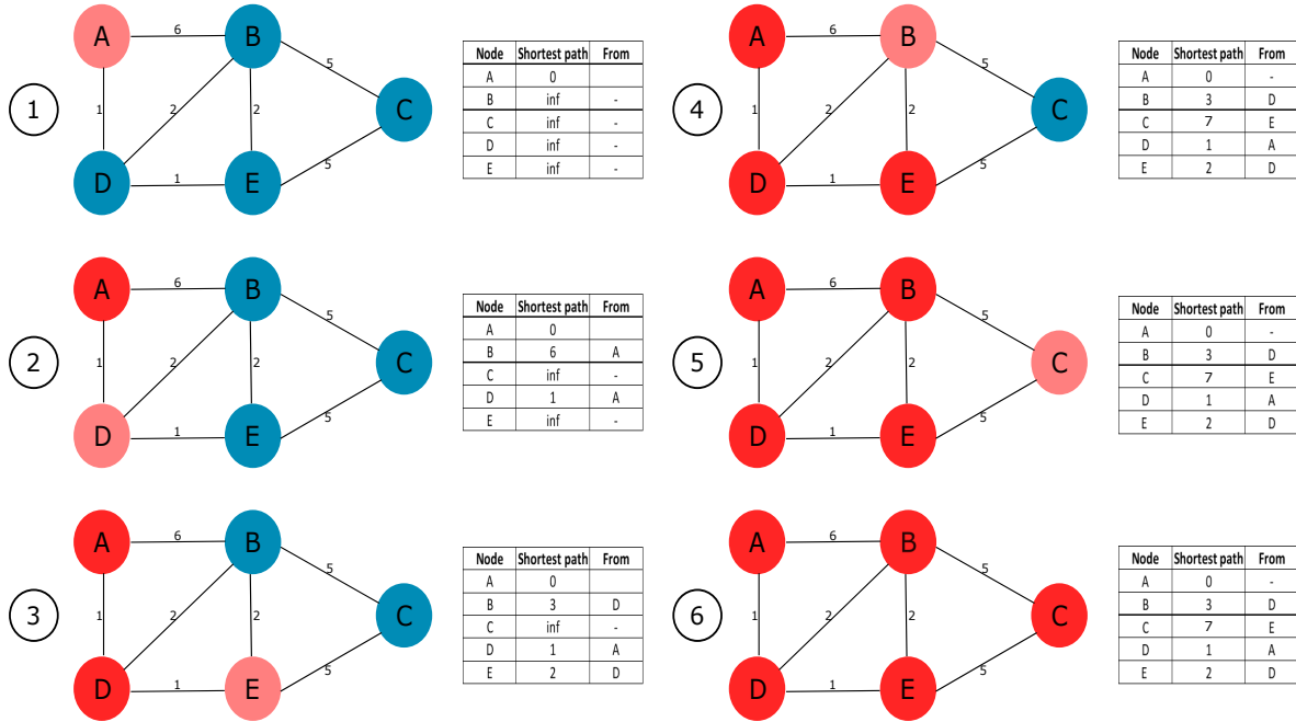
Figure 3.4: Dijkstra's algorithm to find the shortest path between A and C in a small graph. In step one, the algorithm is initialized. the distance to each node is marked as \infty with the exception of source node A. After the distance for reaching each neighbor of A is computed, it is removed from N' (red). The process is repeated for the node with the shortest distance, at each iteration. The algorithm ends once every node is evaluated.
