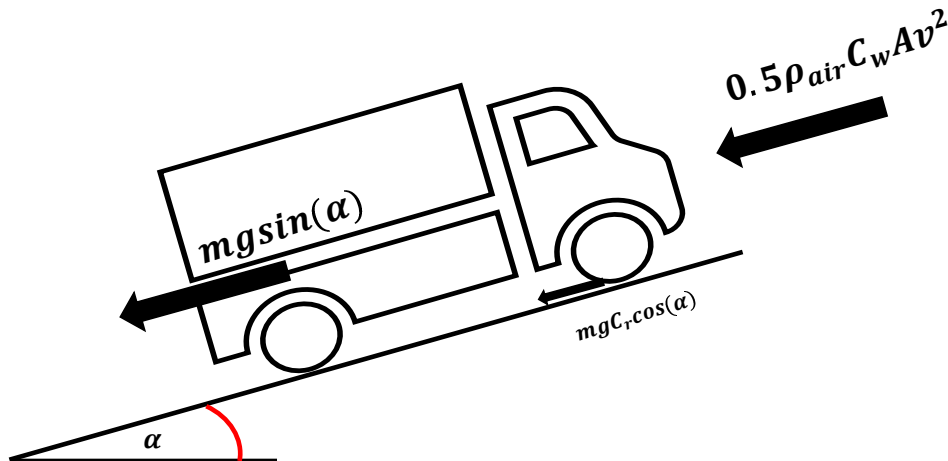
Figure 5.12: Vehicle longitudinal dynamics.
