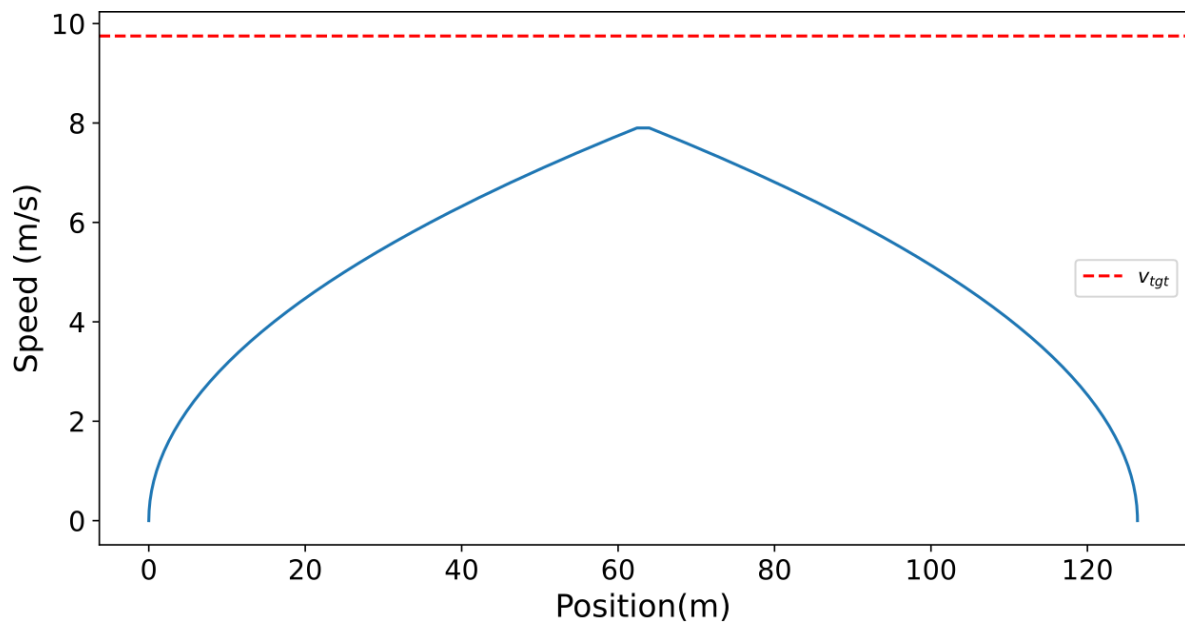
Figure 5.11: Speed in a short link with stop point at beginning and end. The vehicle cannot reach target speed.
