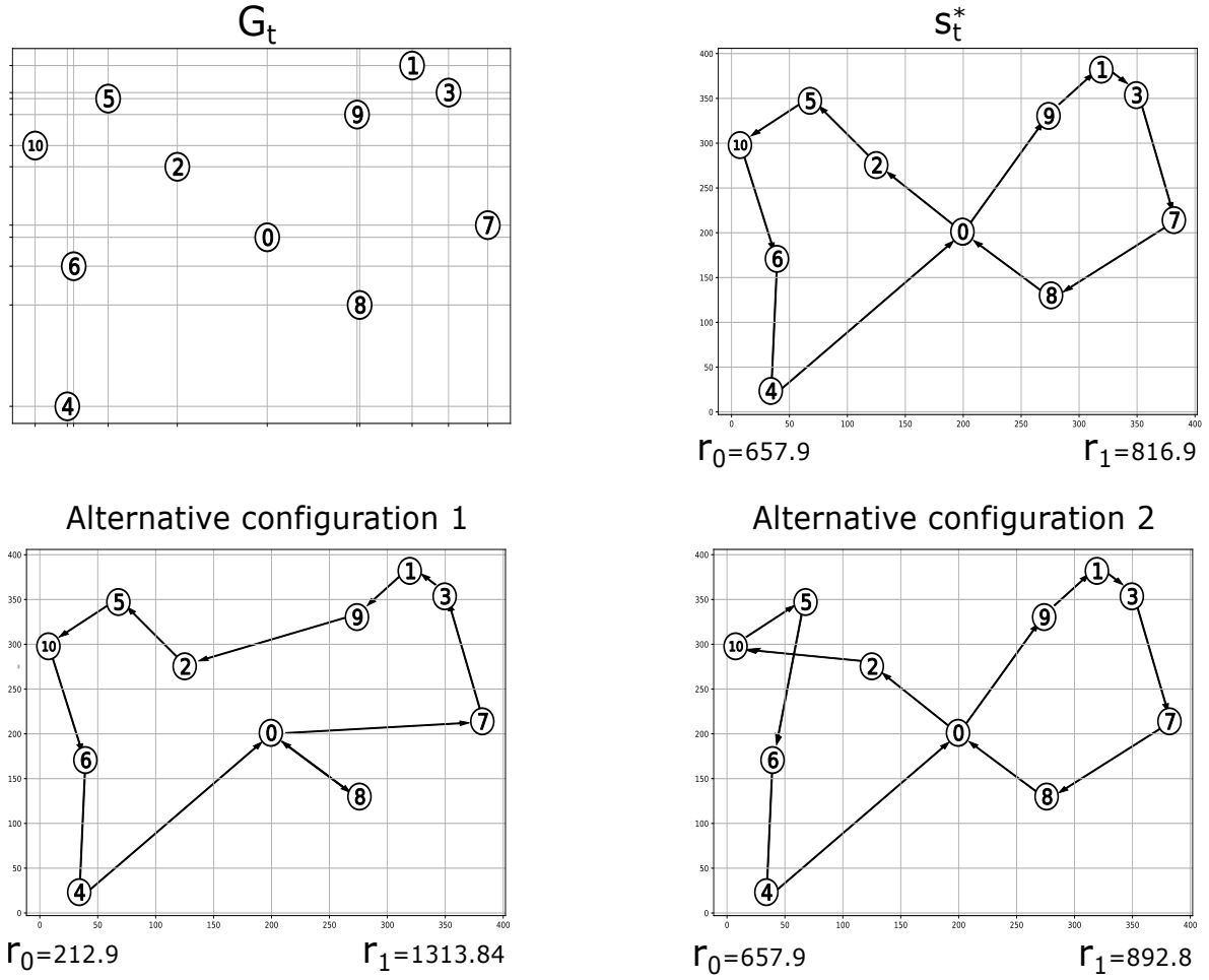
Figure 4.6: Route configuration concept illustration. G_t is the graph containing the points to be visited in working session t . s_t^* is the best route configuration from a fuel cost point of view, obtained through a classic VRP. Two alternative configurations are presented. For every configuration, r_0 and r_1 are the distance of the shortest and longest route, respectively.
