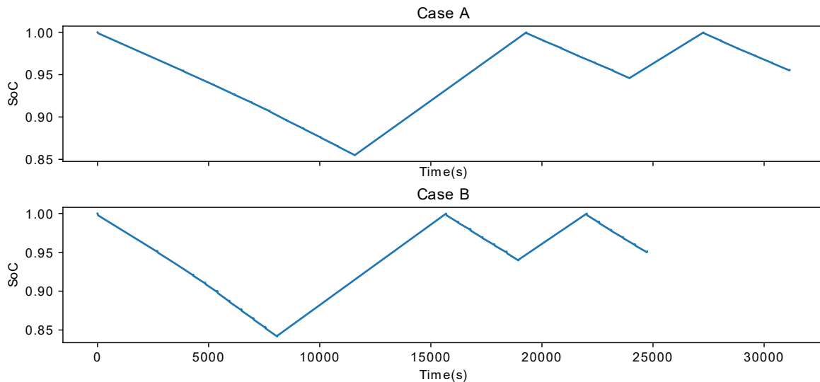
Figure 6.11: Comparison of SoC for optimal mission plan. Case A: acting on driving parameters, Case B: not acting on driving parameters. Notice that in Case B, the mission plan ends earlier because of different driving parameters (higher speed and acceleration)
