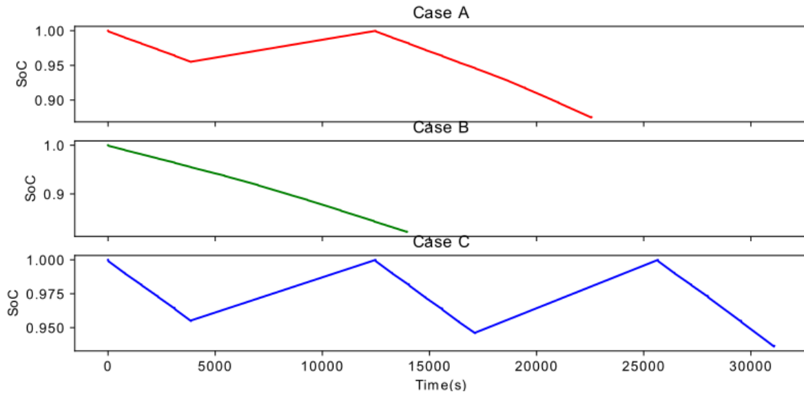
Figure 6.9: Comparison of SoC for optimal mission plan for different optimization cases: Case A accounts for both degradation and energy ( c_{batt} \neq 0 and c_e \neq 0 ), case B only for energy ( c_{batt} = 0 ) and case C only for degradation ( c_e = 0 ).
