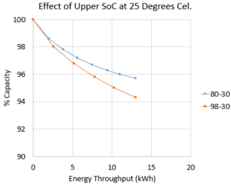
Figure 5.6: Effect of battery usage on capacity fade.
