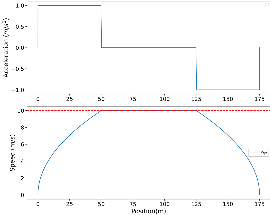
Figure 5.9: Vehicle speed starting at idle and going through a road link with a stop at the end.
