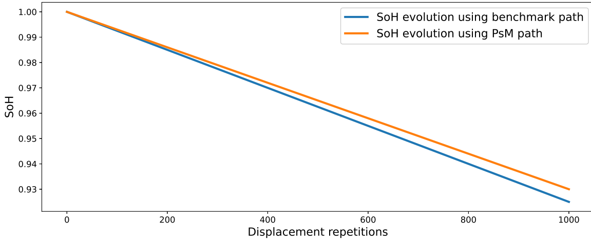
Figure 6.4: Long term comparison between the two vehicles, following the different paths found, in terms of SoH
