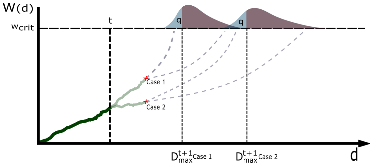
Figure 4.11: Illustration of the closed-loop approach for failure distance distribution updates.
