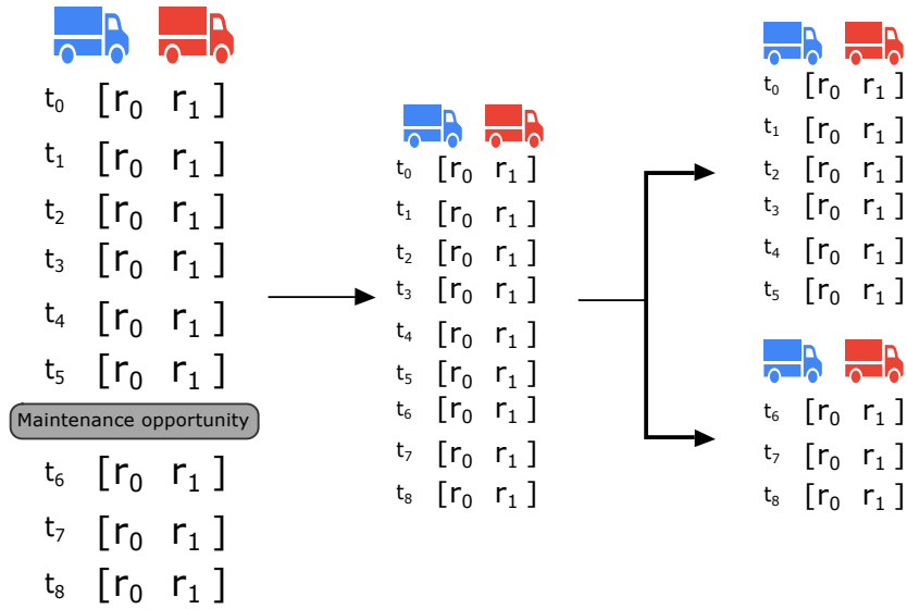
Figure 4.10: Solution strategy to address instances including maintenance
