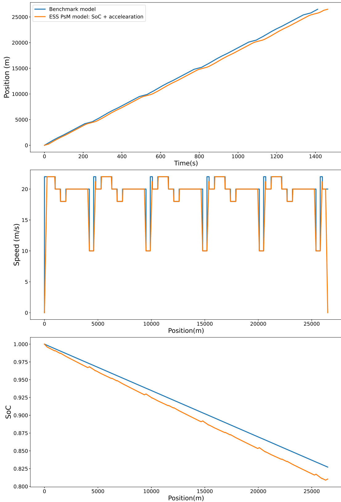
Figure 5.16: Comparison between position, speed and SoC as estimated by the two different models
