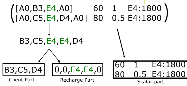
Figure 6.7: First step on the crossover operation.
