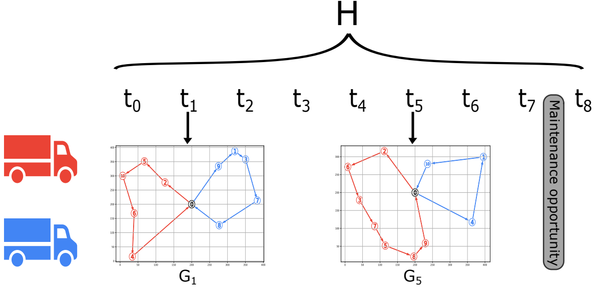
Figure 4.2: Visual representation of the PsM optimization problem for a generic vehicle component. Each working session t is indexed in this Figure for the sake of clarity. At each working session, a graph G_t is used to define routes, as explicitly shown for t_1 and t_5 . In this case, V = [7] , meaning maintenance operations can occur between t_7 and t_8 .
