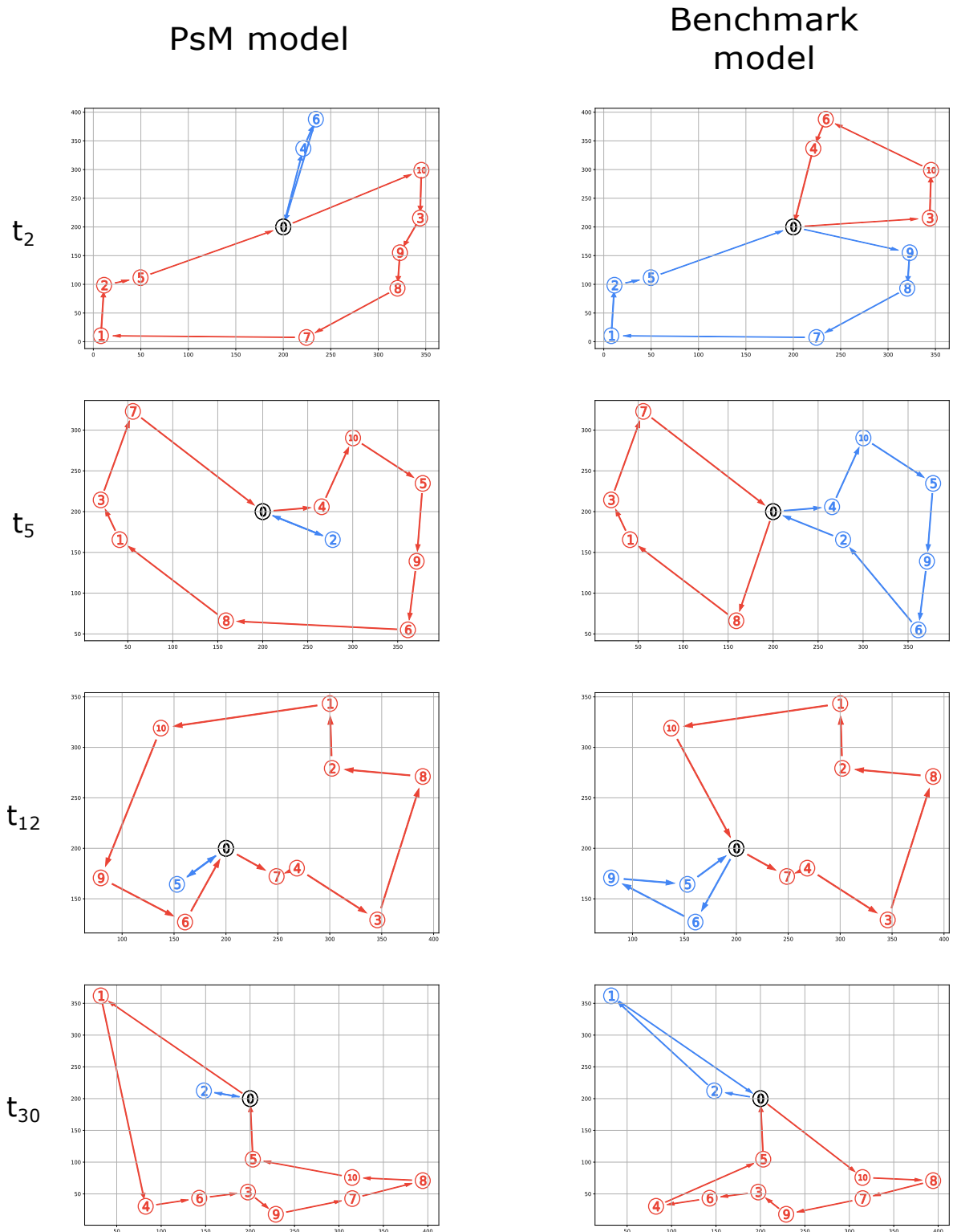
Figure 4.5: working sessions in which routes used by each model were different. Notice that the PsM model chooses routes that allow vehicle 1 (represented in blue) to travel shorter distances and respect its safety constraints.
