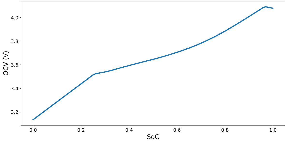
Figure 5.5: OCV SoC curve for a lithium-ion cell.
