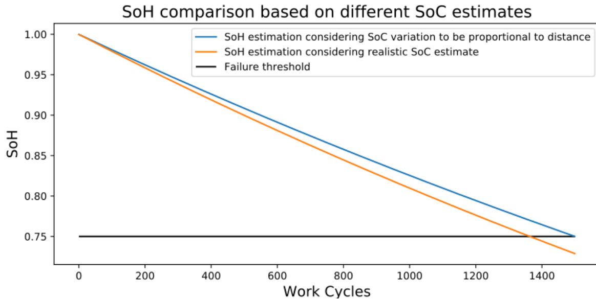
Figure 5.17: Comparison of end of life estimation: PsM SoC model vs benchmark model.
