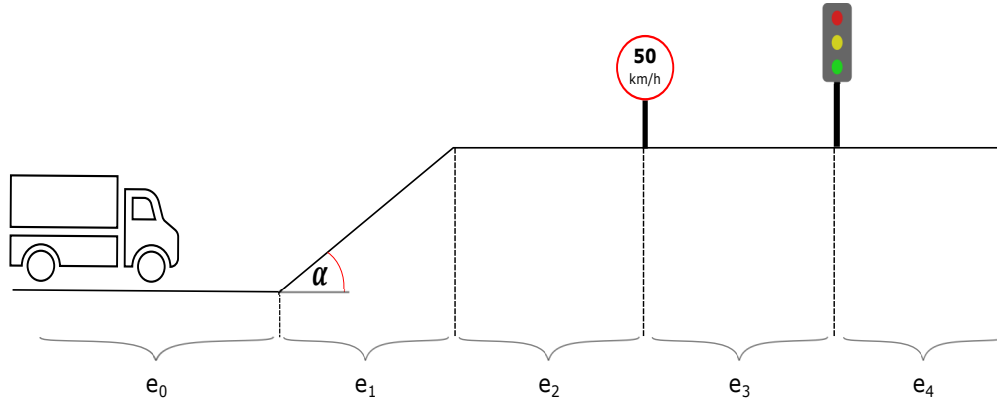
Figure 5.8: Example of how road links are defined. In this example, four links are shown. Links are created to represent differences on the parameters relevant to acceleration or power estimation. In this example, e_1 and e_2 are created due to a inclination difference with respect to the previous link. e_3 is defined due to a speed change and e_4 is due to the presence of a traffic light.
