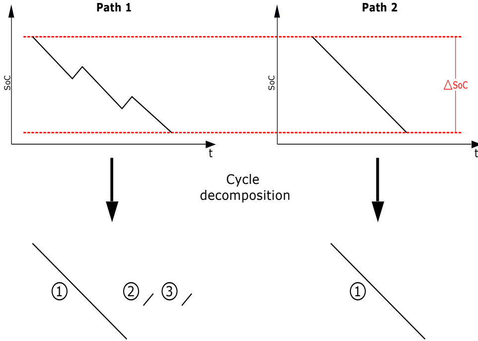
Figure 6.2: SoC(t) for paths considered equivalent in classical SPPs
