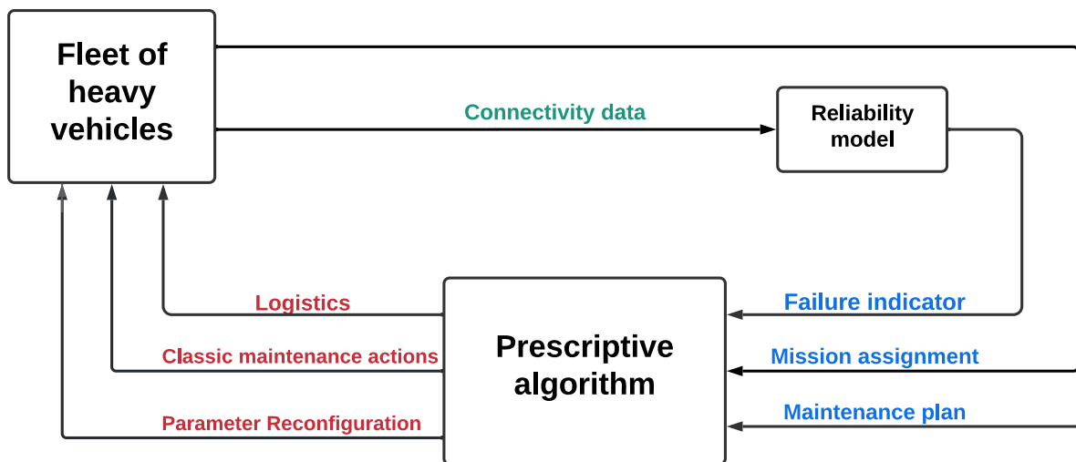
Figure 7.1: General PsM loop for heavy vehicles
