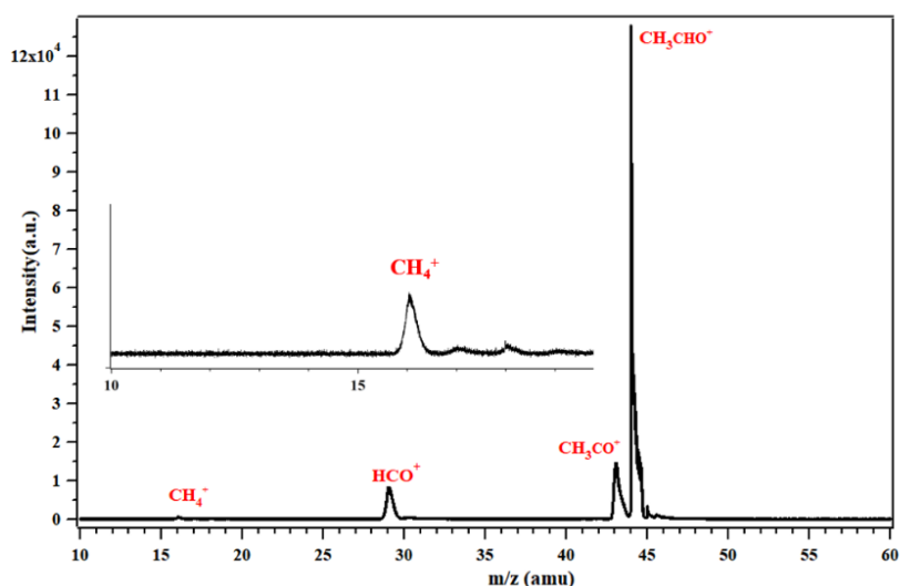
Figure 5.1 Synchrotron photoionization mass spectrum in 10.0-13.8eV energy range.
