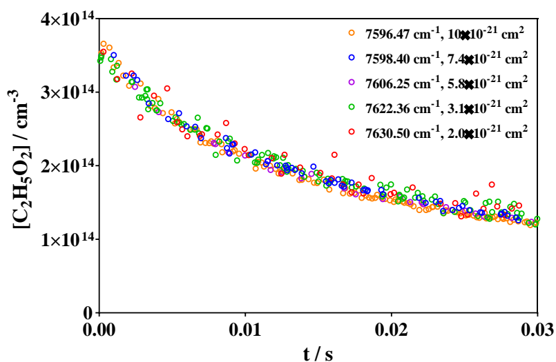
Figure 3.9 Examples of C_2H_5O_2 decays following the 351 nm photolysis [Cl_2] = 3 \times 10^{16} cm^{-3} in presence of [C_2H_6] = 2.6 \times 10^{16} cm^{-3} , obtained at 5 different wavelengths: the absorption cross-section of C_2H_5O_2 (given in the legend of the figure) varies over a factor of 5 for the different wavelengths.
