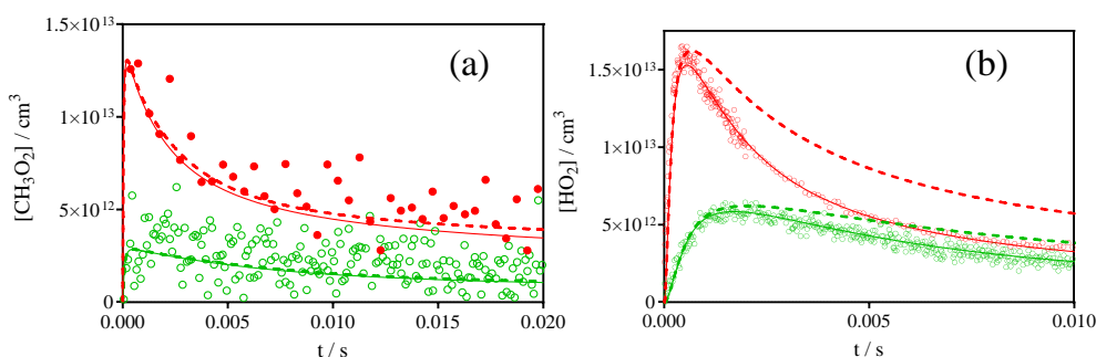
Figure 4.8 Experimental results of CH 3 O 2 and HO 2 for Exp.1 and 5 and simulation results with model in Table 4.6 (solid line) and model from Table 4.6 but without the self-reaction of CH 2 OO and the reaction of the stabilized Criegee sCH 2 OO with HO 2 and CH 3 O 2 (dashed line).
