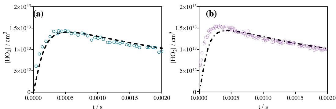
Figure 4.4 Zoomed HO 2 profiles over the first 2 ms for Exp.2 (a) and Exp.3 (b), the black dashed line (a) and dash-dotted line (b) are the simulation profiles with additional HO 2 formed by Cl + CH 2 O reaction, the added concentration of CH 2 O is 8 \times 10^{12} \text{ cm}^{-3} .
