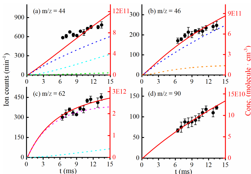
Figure 3.12 Time-evolutions of products in the self-reaction of C 2 H 5 O 2 and its cross-reaction with HO 2 . (a) CH 3 CHO, m/z = 44 , (b) C 2 H 5 OH, m/z = 46 , (c) C 2 H 5 OOH, m/z = 62 , (d) C 2 H 5 OOC 2 H 5 , m/z = 90 . Black dots are experimental data and red curves are calculated from a theoretical model. Blue line: from C 2 H 5 O 2 self-reaction contribution; cyan line: from C 2 H 5 O + C 2 H 5 O 2 contribution; pink line: from C 2 H 5 O 2 + HO 2 contribution; green line: from C 2 H 5 O + O 2 contribution; orange line: from C 2 H 5 O + HO 2 contribution.
