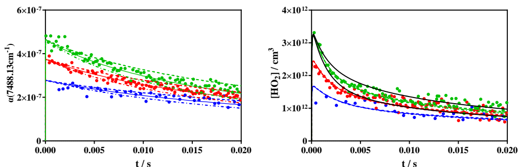
Figure 4.15 Left graph: CH 3 O 2 profiles for highest C 2 H 5 O 2 excess: full lines represent best simulation with rate constants from Table 4.10 ( k(\text{CH}_3\text{O}_2 + \text{C}_2\text{H}_5\text{O}_2) = (3.8 \pm 1.5) \times 10^{-13} \text{ cm}^3 \text{ s}^{-1} ), dashed lines represent a variation of k(\text{CH}_3\text{O}_2 + \text{C}_2\text{H}_5\text{O}_2) of \pm 1.5 \times 10^{-13} \text{ cm}^3 \text{ s}^{-1} . Right graph: HO 2 profiles for the same experiment. Full colored line represents best model with a radical yield of 0.4, dashed lines in the right graph show the model with k(\text{CH}_3\text{O}_2 + \text{C}_2\text{H}_5\text{O}_2) varied as shown in left graph, but the branching ratio varied to best reproduce experiment (see text). The black lines show a variation of \pm 0.2 for the branching ratio for the highest radical concentration.
